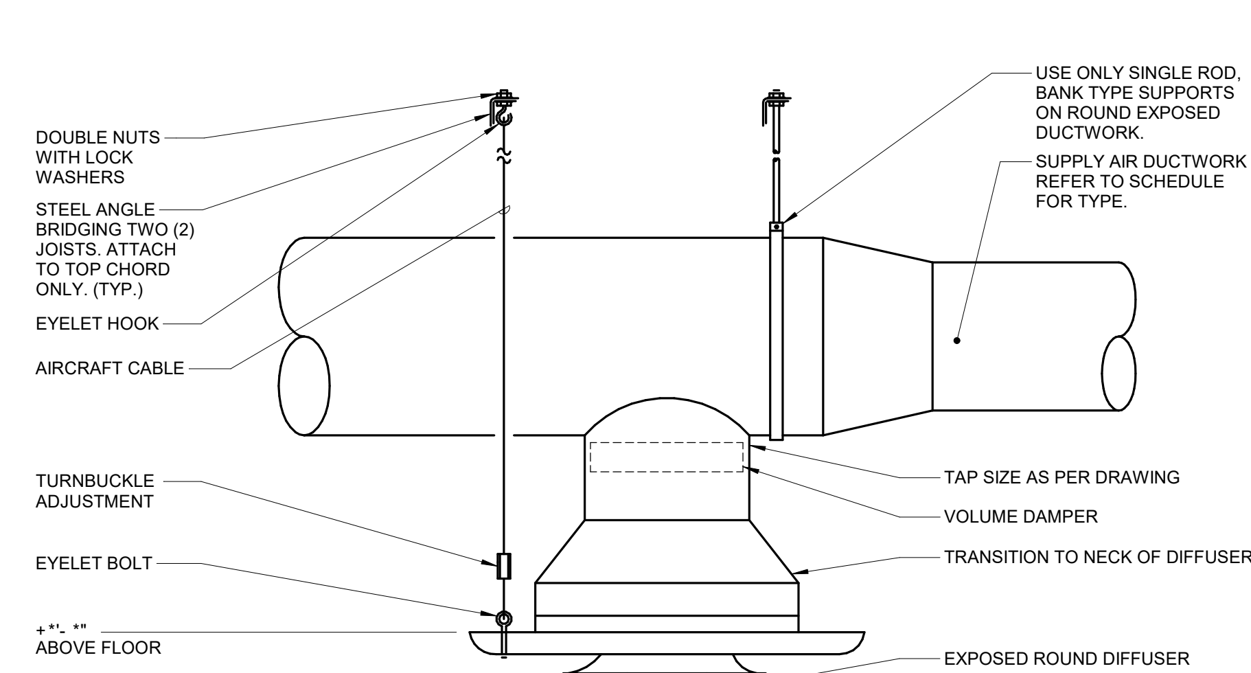
1 AIR TERMINAL - ROUND RIGID CONNECTION NO SCALE
