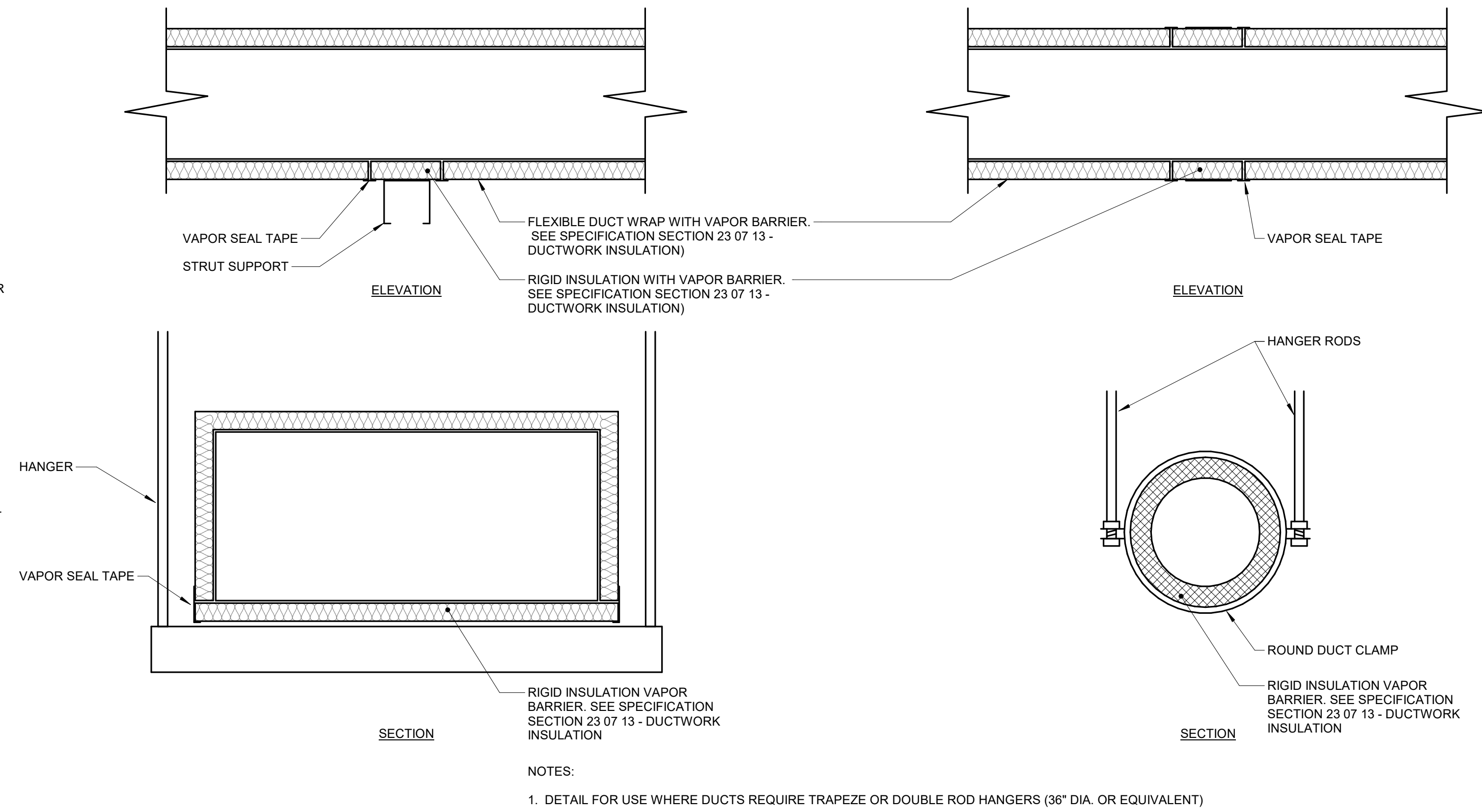
7 DUCT - HANGERS WRAPPED NO SCALE
