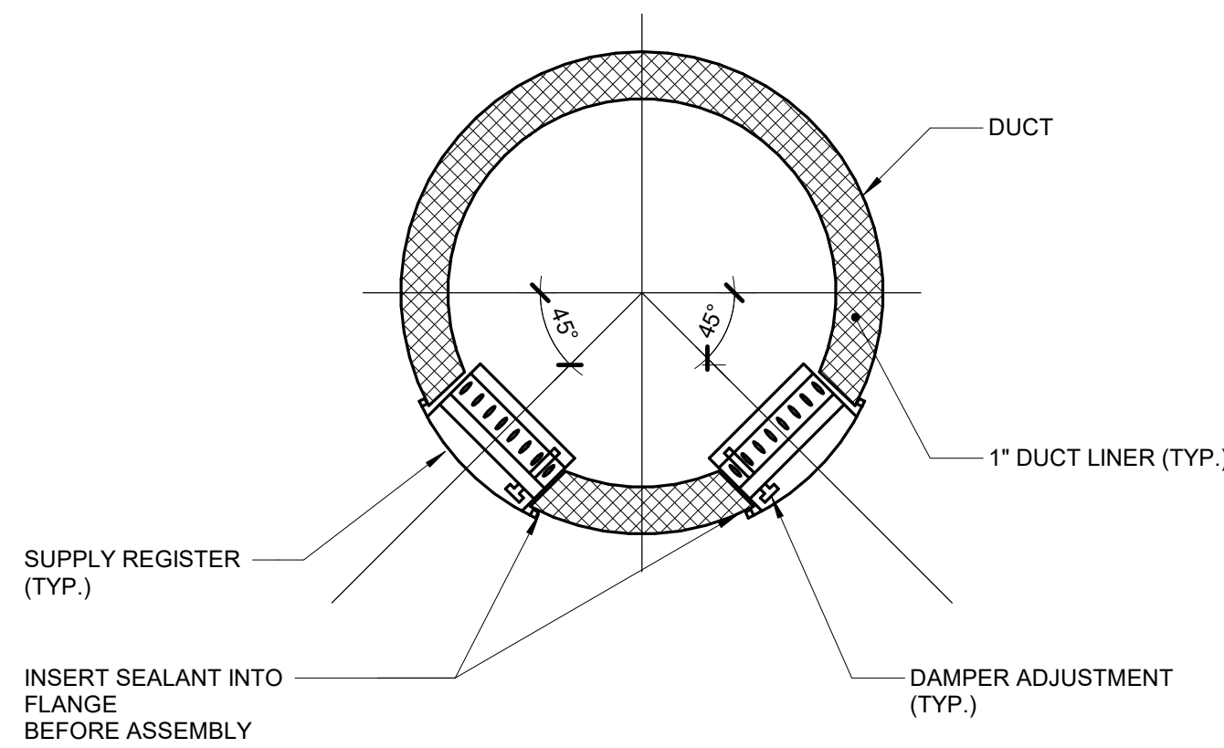
5 AIR TERMINAL - SUPPLY REGISTER ROUND INSET NO SCALE
