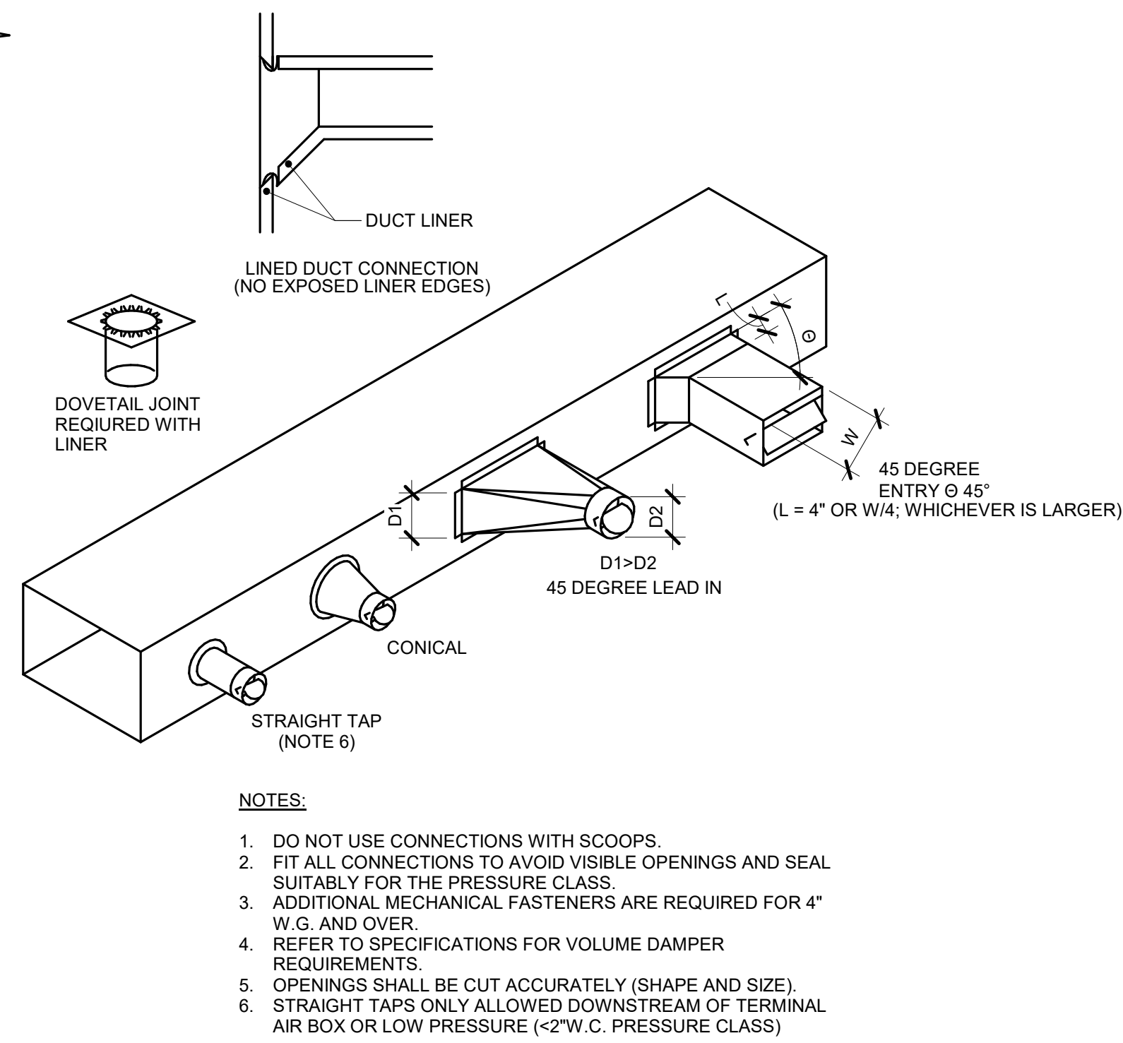
8 DUCT - BRANCH CONNECTIONS NO SCALE
