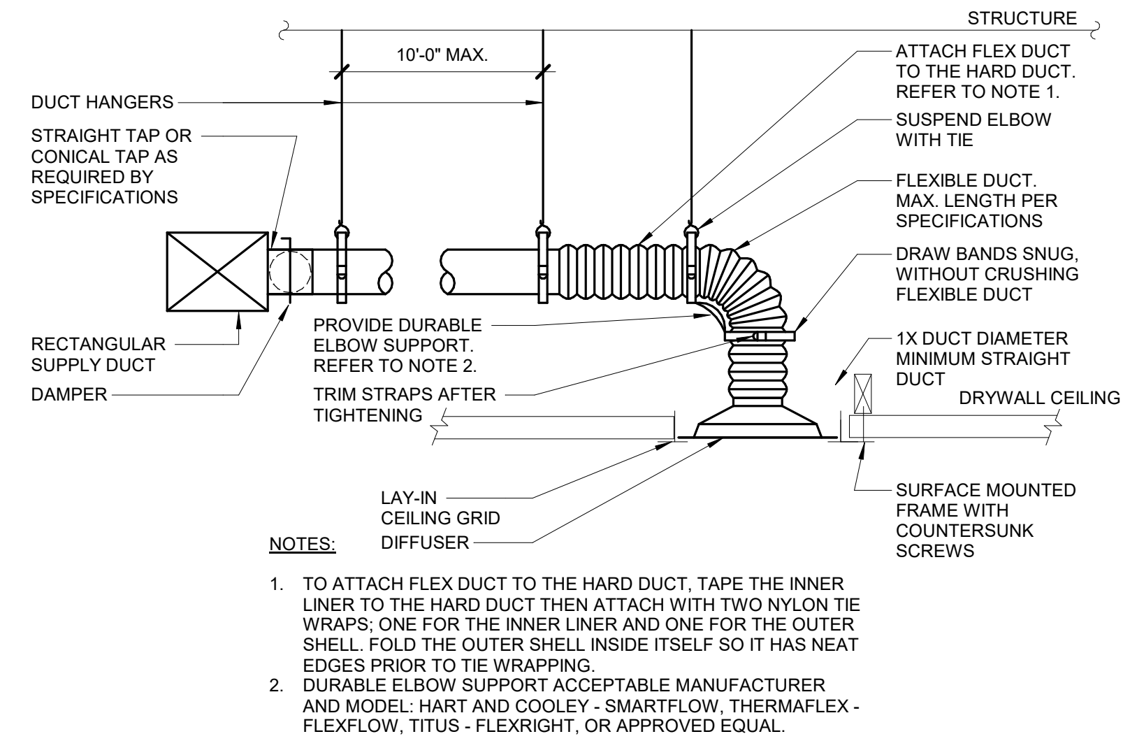
3 AIR TERMINAL - DIFFUSER CONNECTION (W/ RADIUS FORMING ELBOW) NO SCALE
