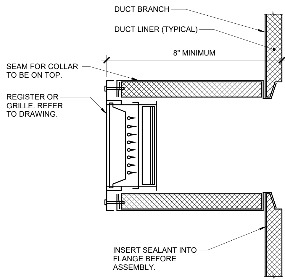
4 DUCT - EXPOSED REGISTER NO SCALE
