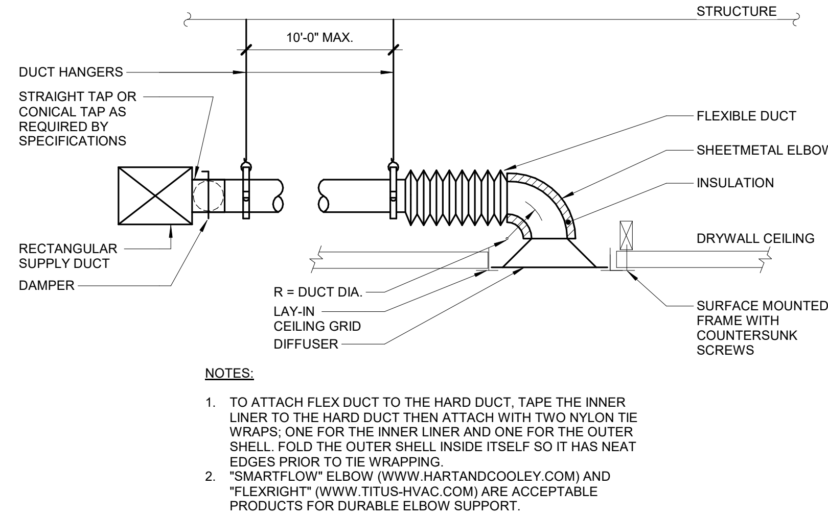
2 AIR TERMINAL - DIFFUSER FLEX LOW PROFILE ELBOW NO SCALE
