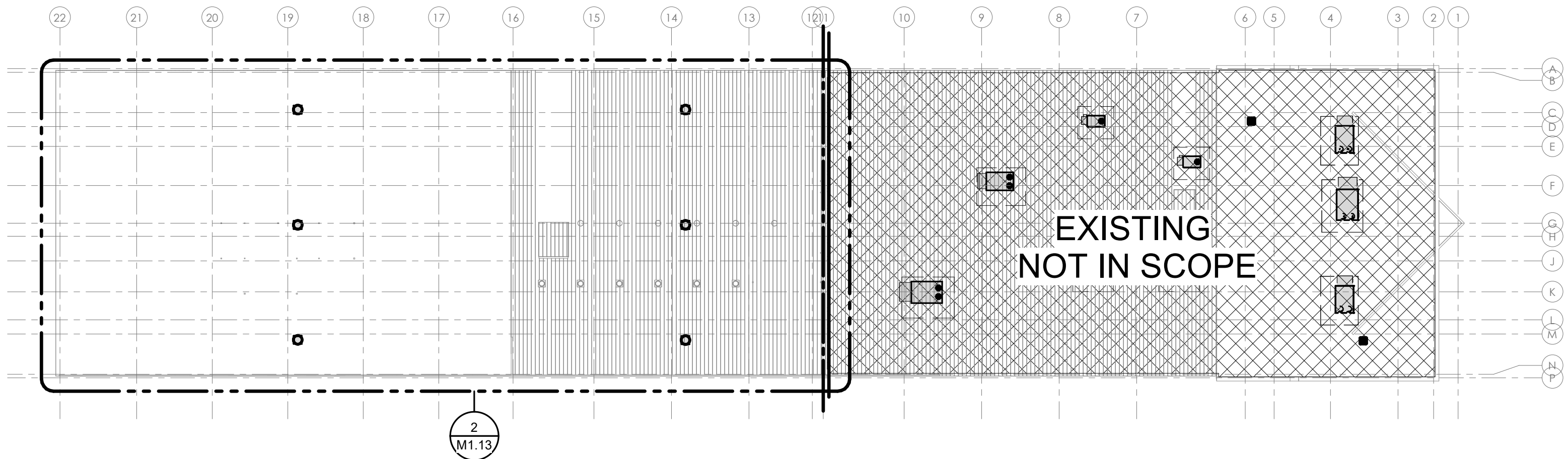
1 ROOF HVAC DEMOLITION PLAN OVERALL 1/32" = 1'-0"
