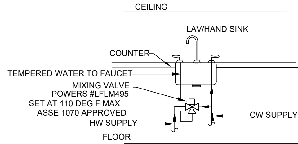
4 MIXING VALVE DETAIL NO SCALE
