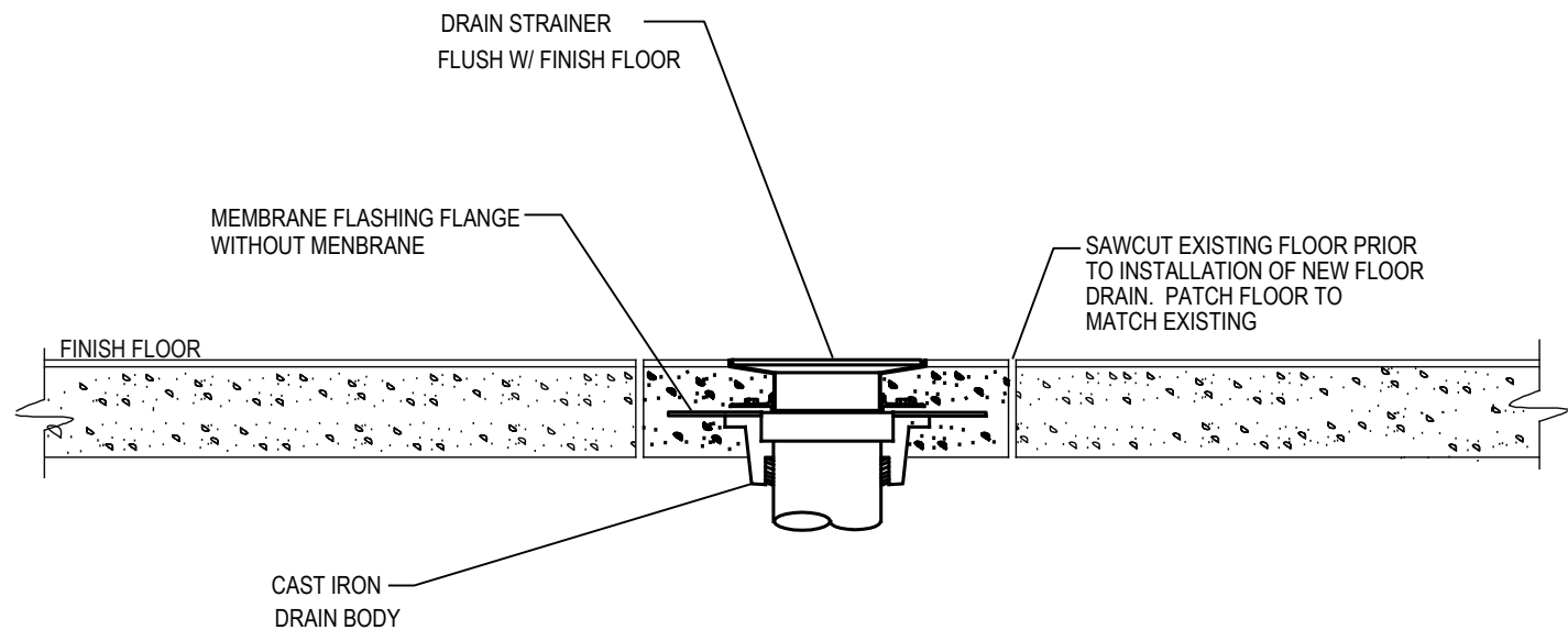
2 FLOOR SINK FLASHING DETAIL NO SCALE
