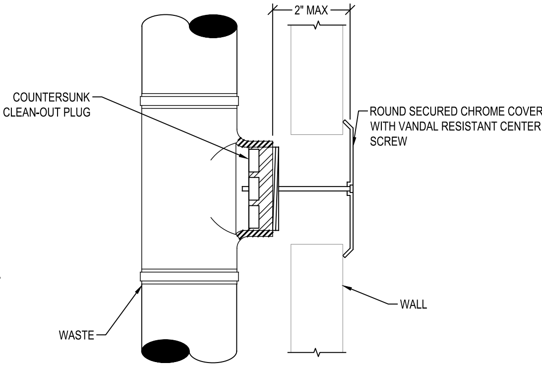
1 WALL CEANOUT DETAIL NO SCALE
