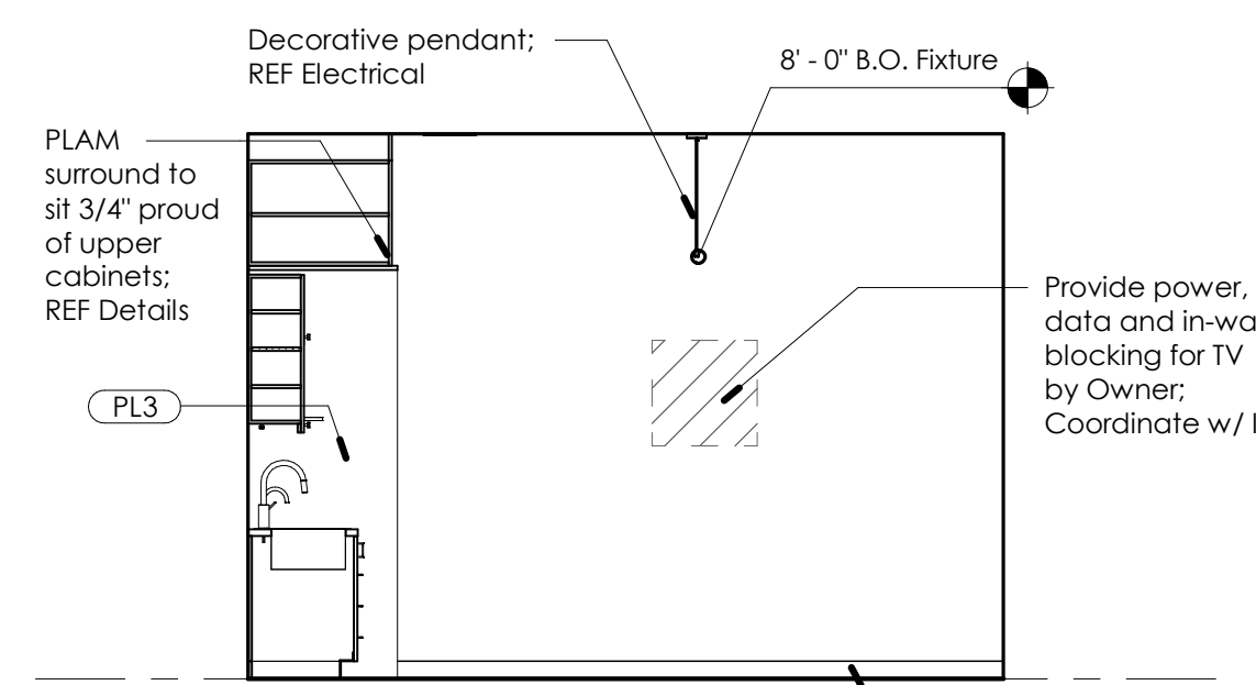
11 319 - Staff - East 1/4" = 1'-0"
