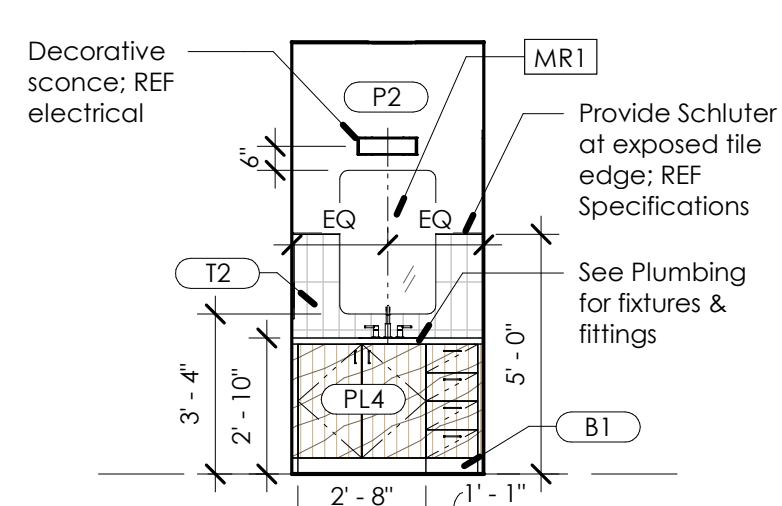
12 322 - Private Restroom - North 1/4" = 1'-0"
