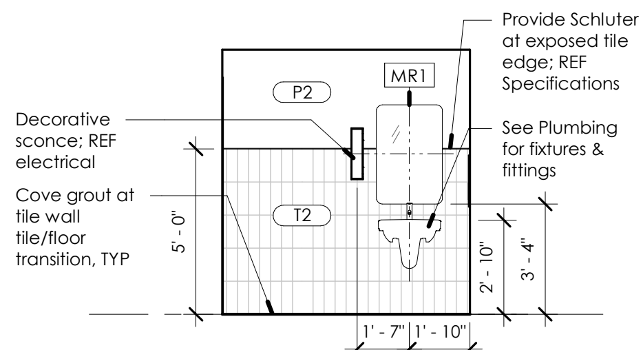
5 317 - Restroom - North 1/4" = 1'-0"
