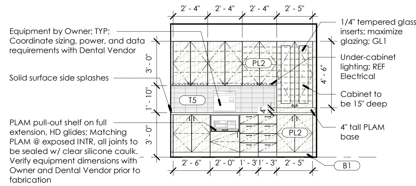
2 313 - Sterilization - East 1/4" = 1'-0"
