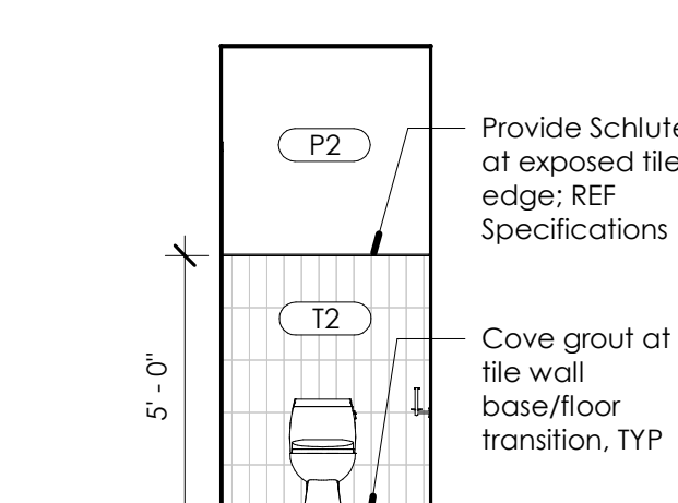
14 322 - Private Restroom - South 1/4" = 1'-0"
