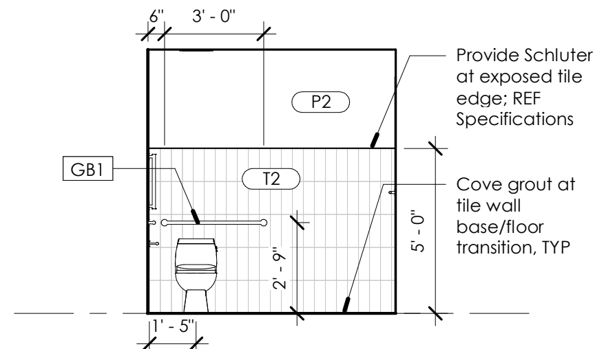
7 317 - Restroom - South 1/4" = 1'-0"
