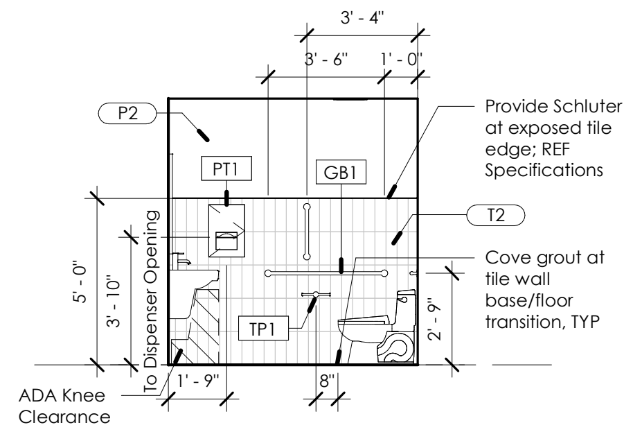
6 317 - Restroom - East 1/4" = 1'-0"
