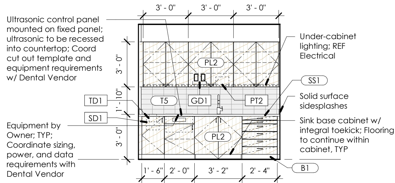
1 313 - Sterilization - West 1/4" = 1'-0"
