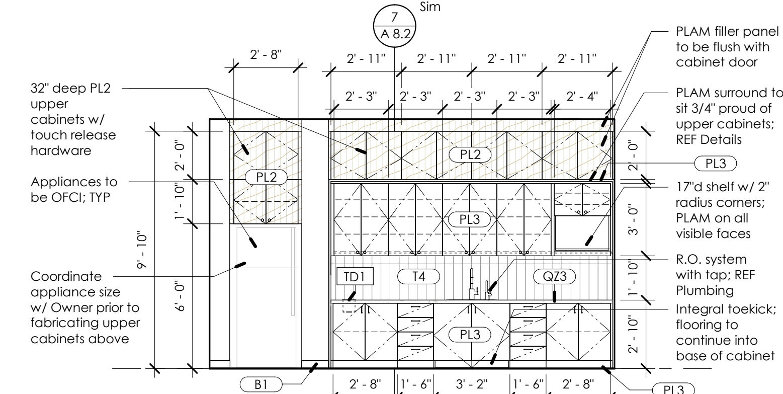
10 319 - Staff - North 1/4" = 1'-0"
