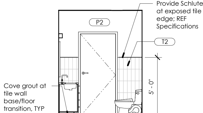
13 322 - Private Restroom - East 1/4" = 1'-0"
