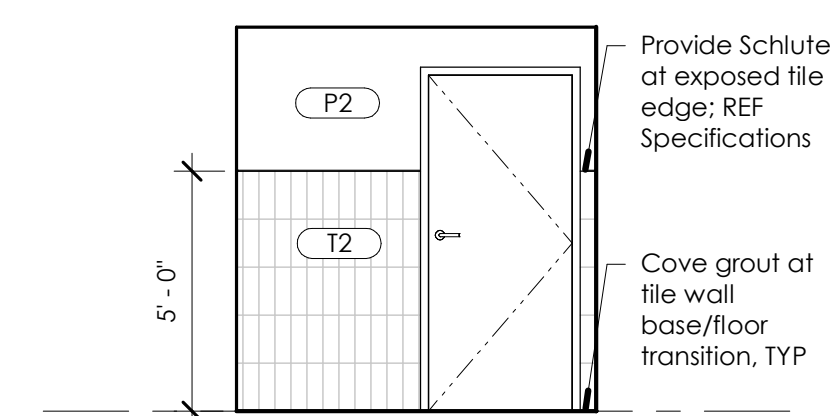
8 317 - Restroom - West 1/4" = 1'-0"
