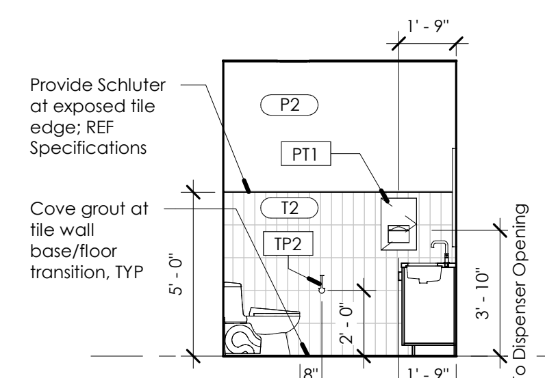
15 322 - Private Restroom - West 1/4" = 1'-0"
