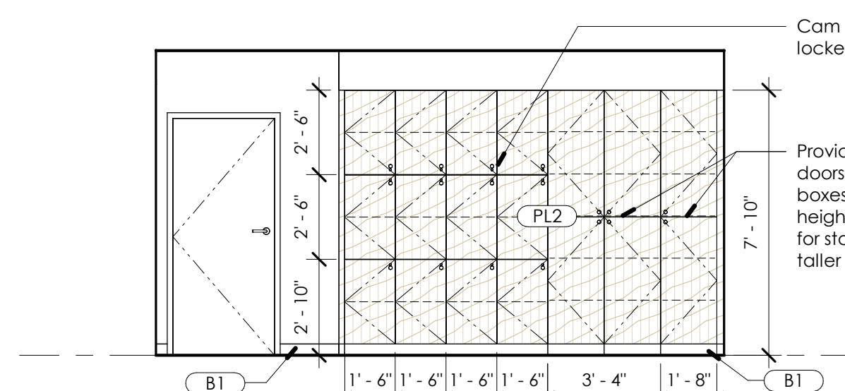
9 318 - Hallway - North 1/4" = 1'-0"
