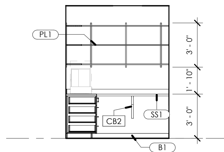
4 315 - Lab - East 1/4" = 1'-0"
