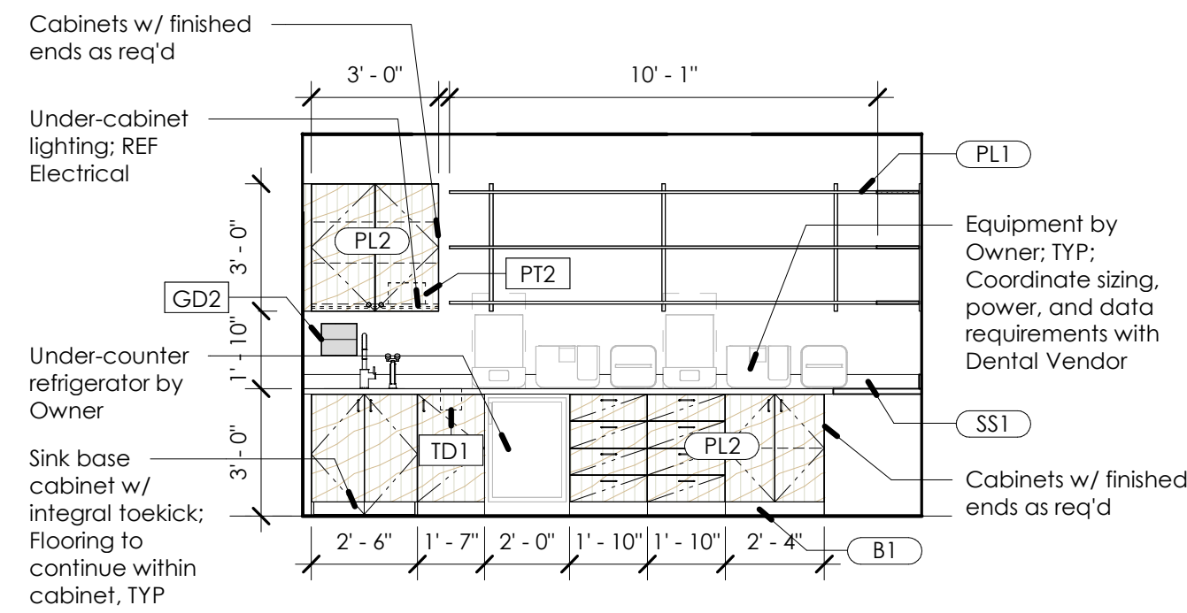
3 315 - Lab - North 1/4" = 1'-0"
