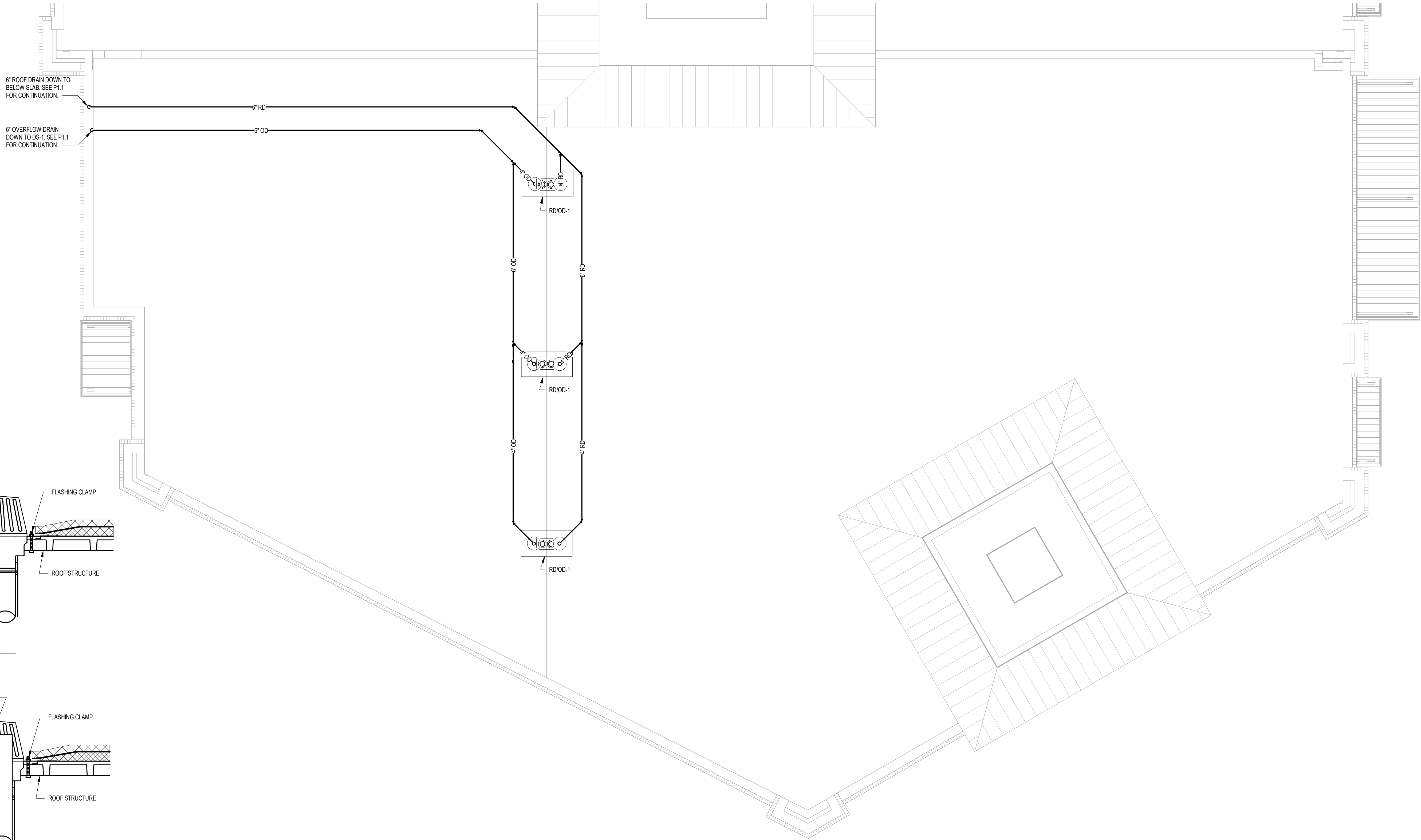
1 PLUMBING DRAIN ROOF PLAN SCALE: 1/4" = 1'-0"
