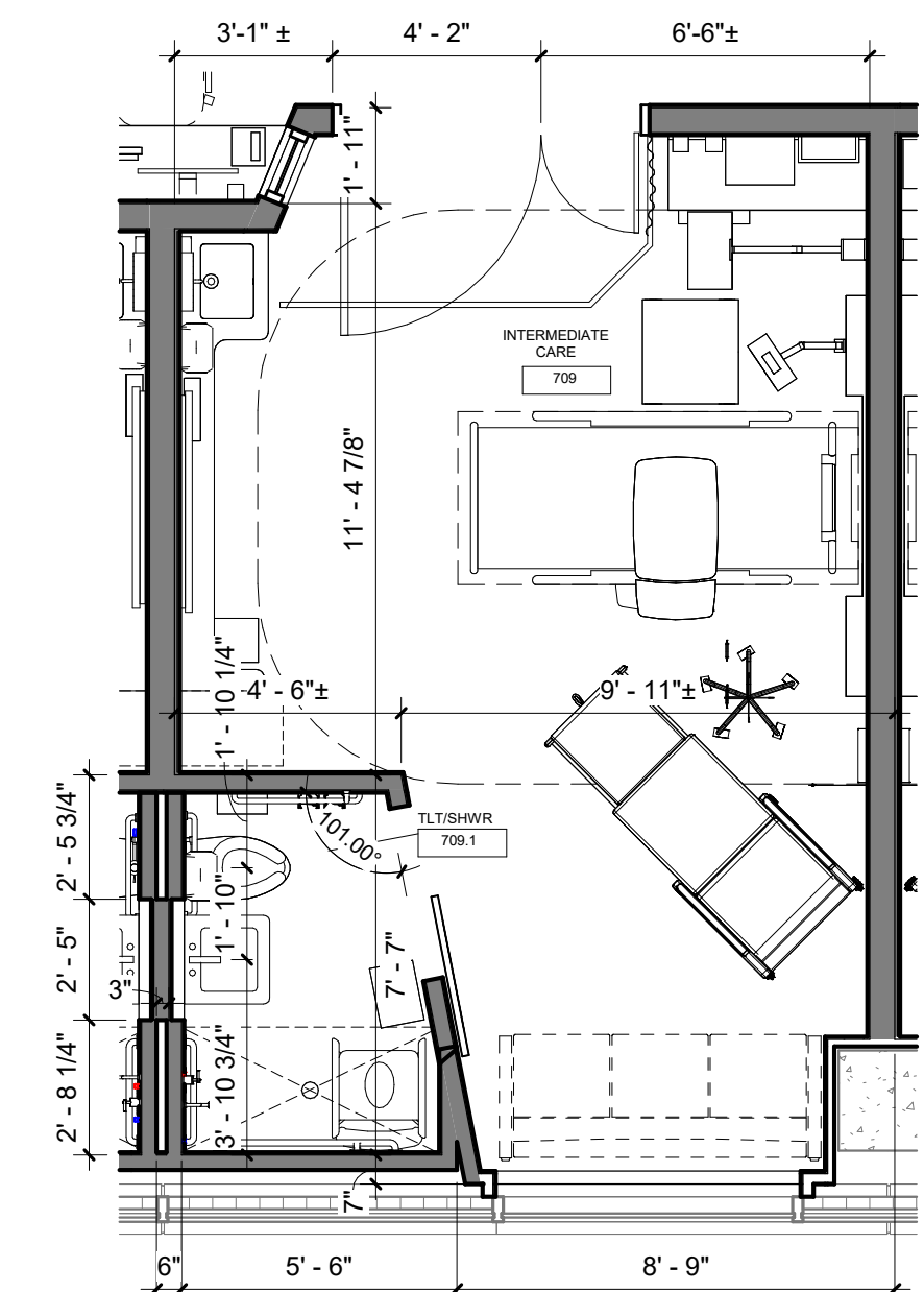
3 TYP. PCU ROOM 1/4" = 1'-0"
