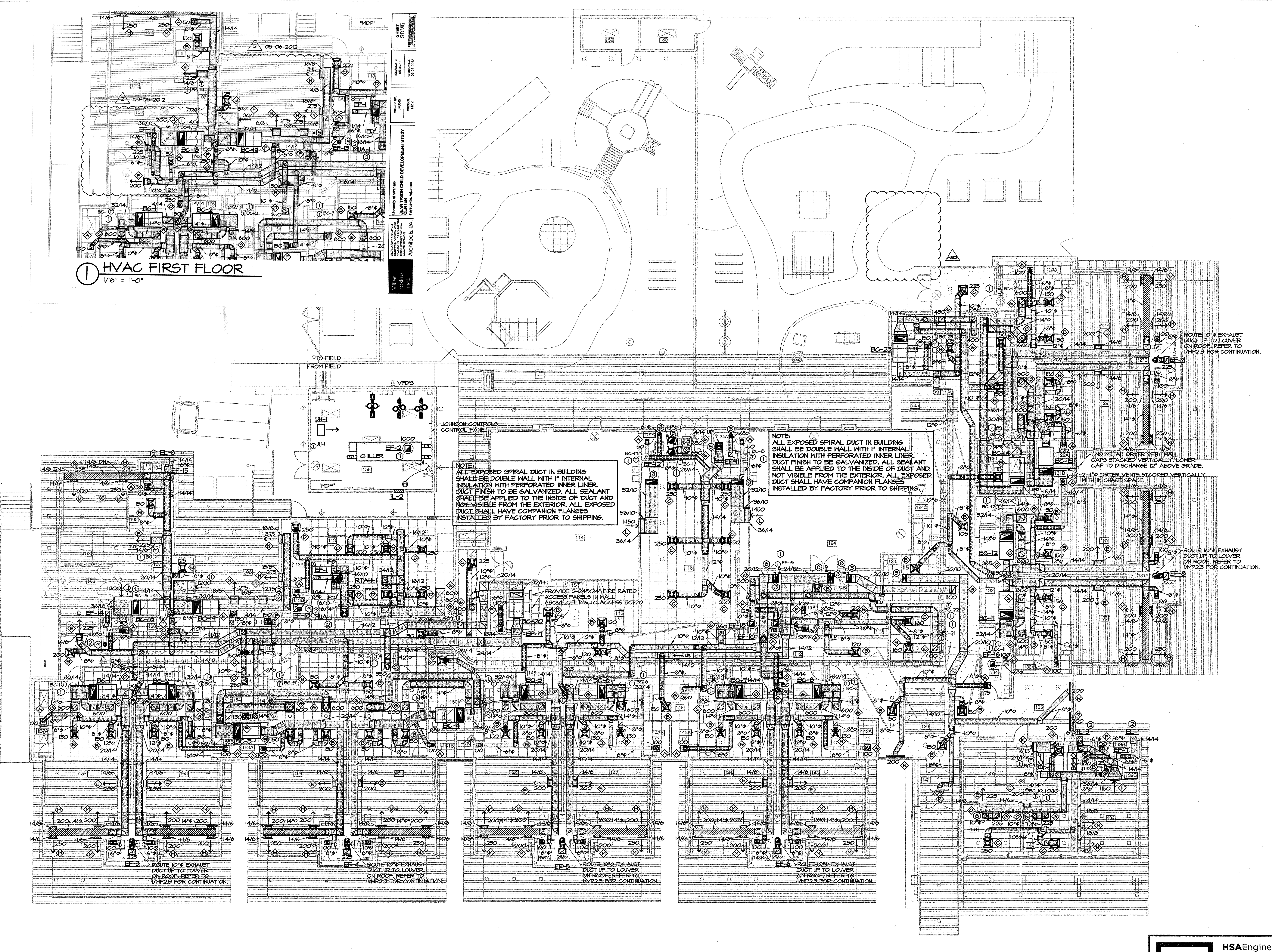
① HVAC FIRST FLOOR PLAN 1/8" = 1'-0"
