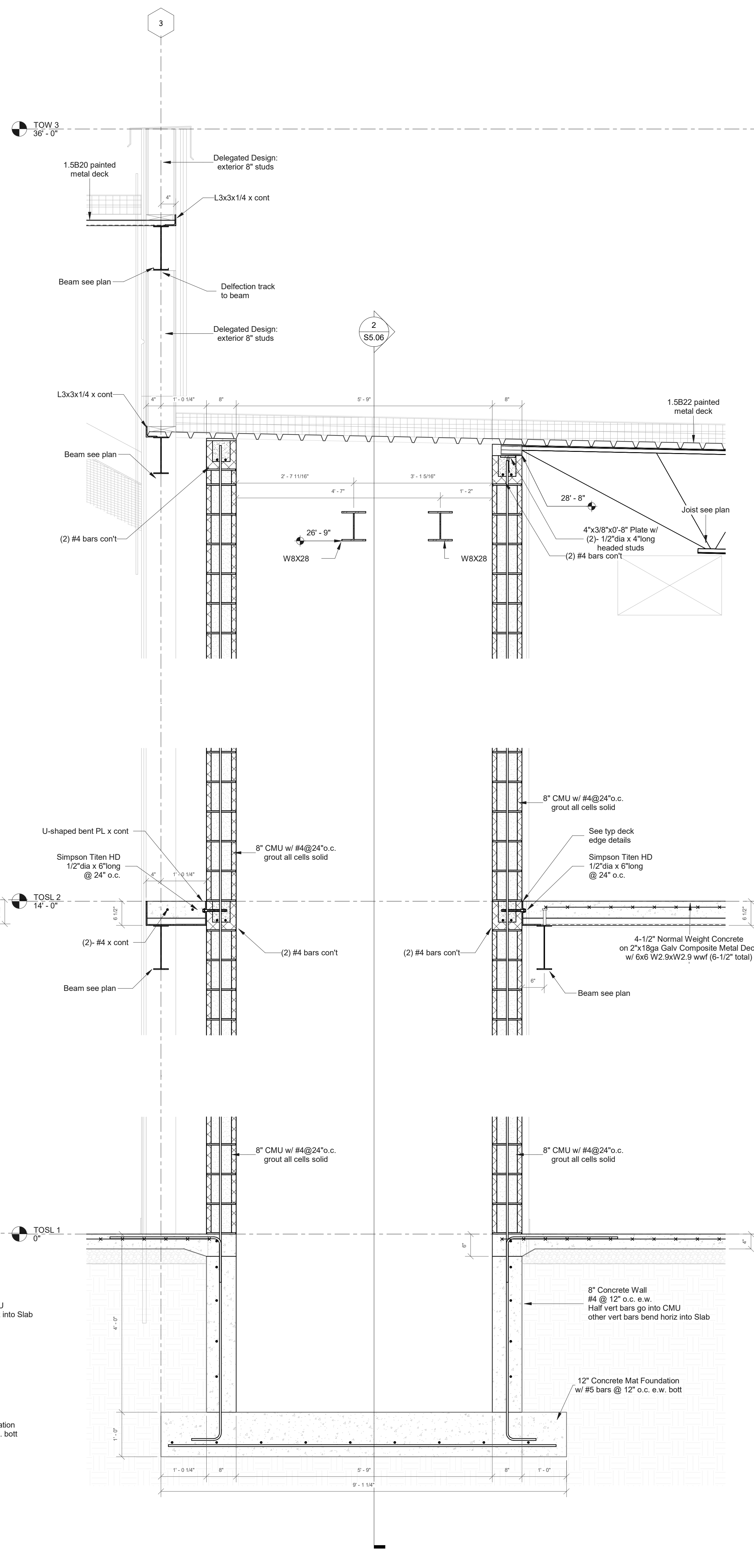
1 Elevator S5.06 3/4" = 1'-0"
