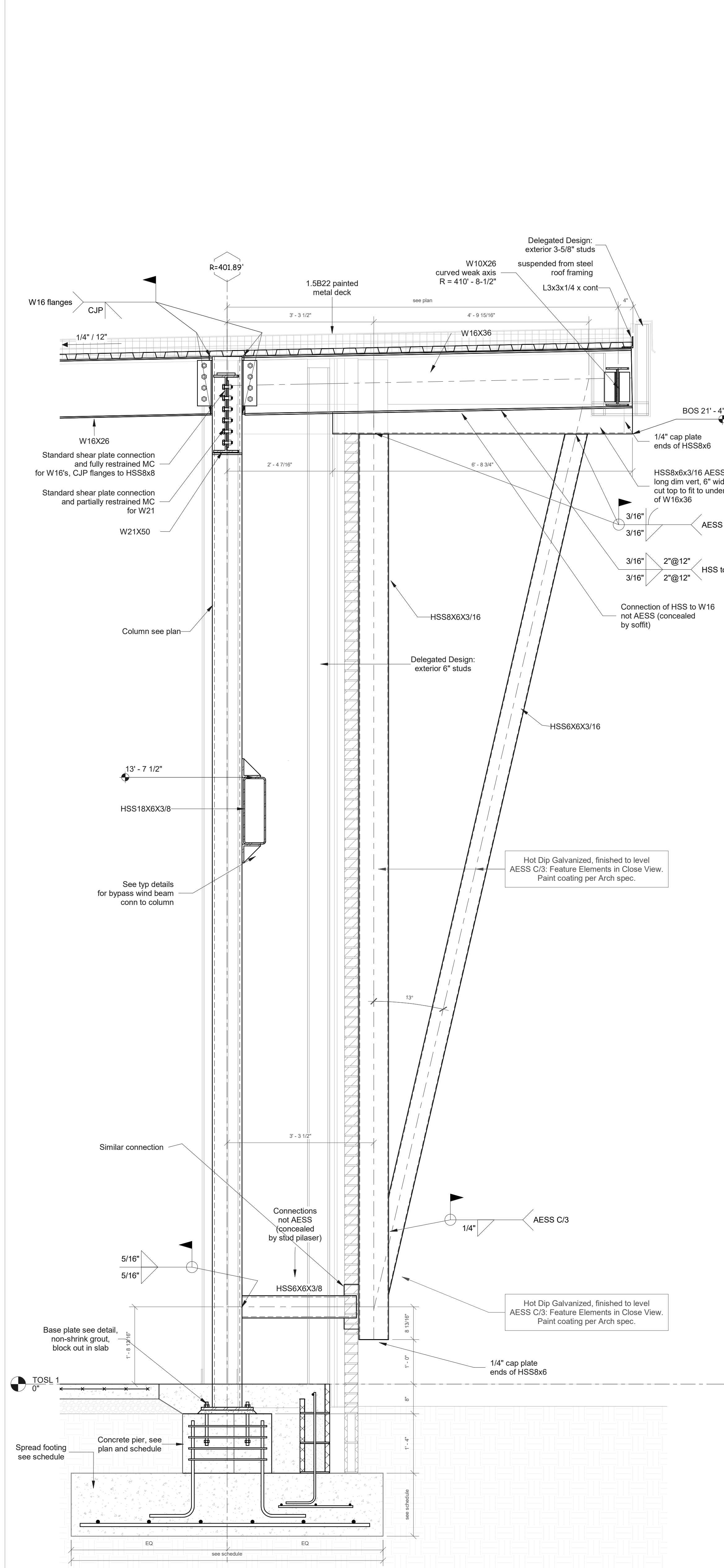
3 Section S5.06 3/4" = 1'-0"
