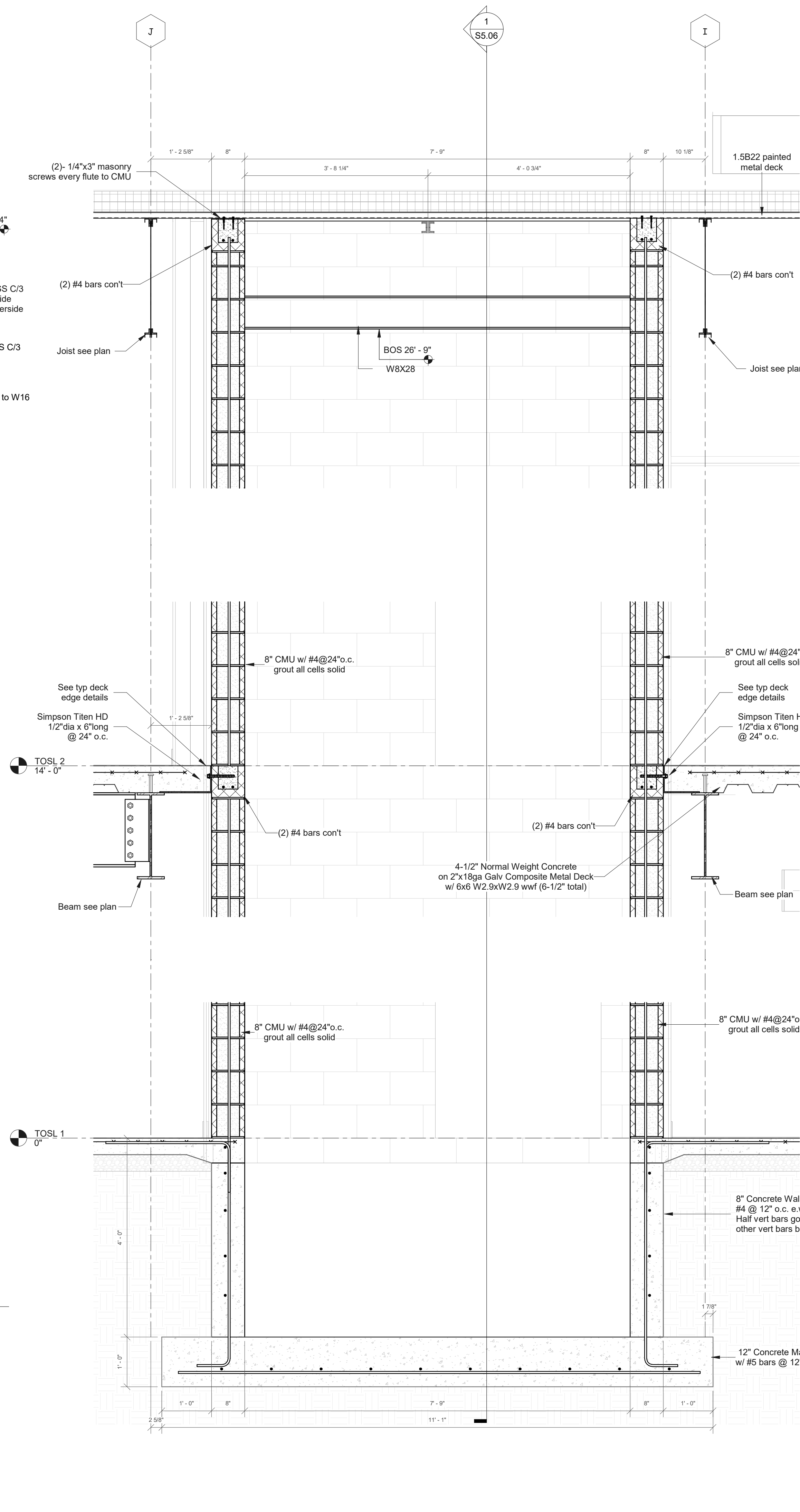
2 Elevator S5.06 3/4" = 1'-0"
