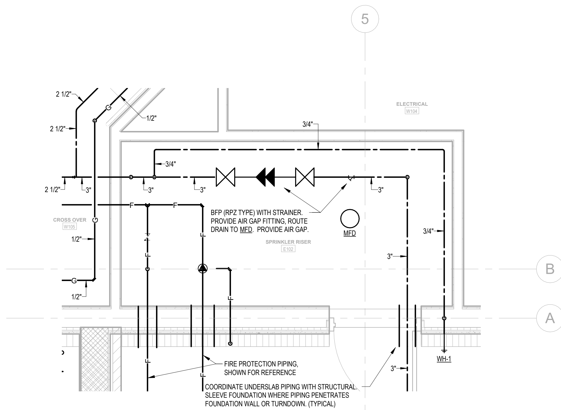
3 ENLARGED SPRINKLER RISER ROOM - PRESSURE 1/2" = 1'-0"
