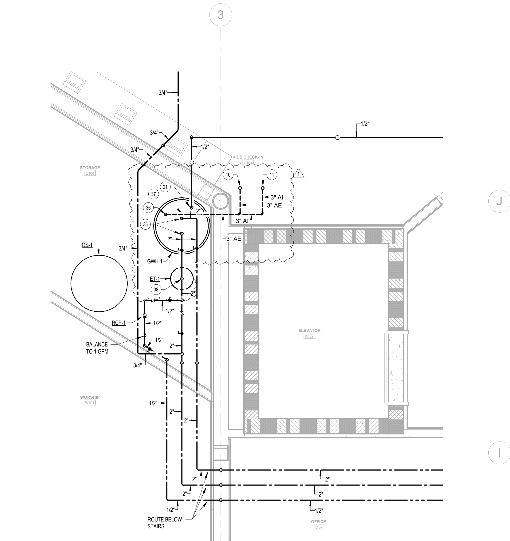
2 ENLARGED EAST SIDE STORAGE ROOM - PRESSURE 1/2" = 1'-0"
