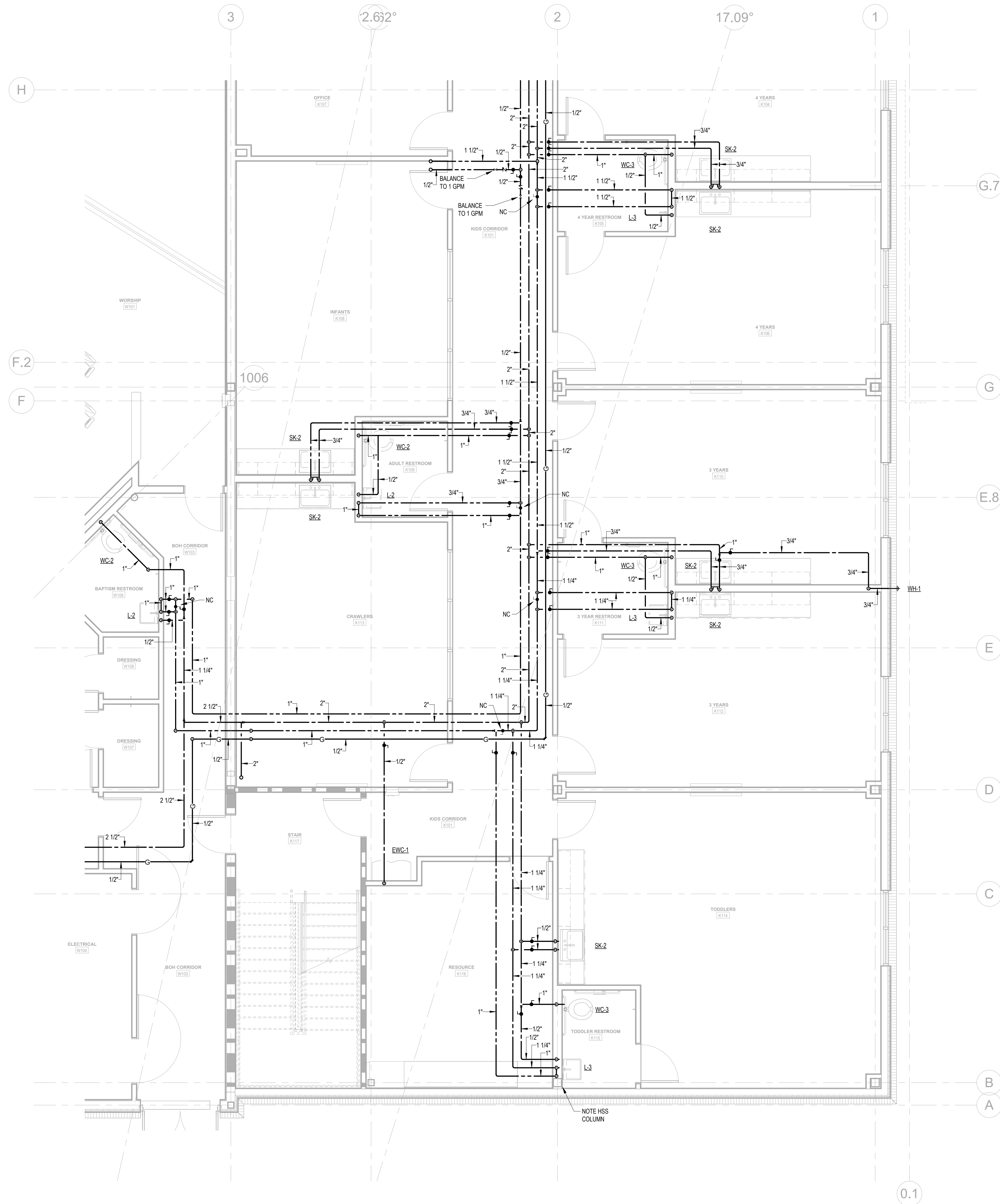
1 ENLARGED EAST SIDE PLAN - PRESSURE 1/4" = 1'-0"
