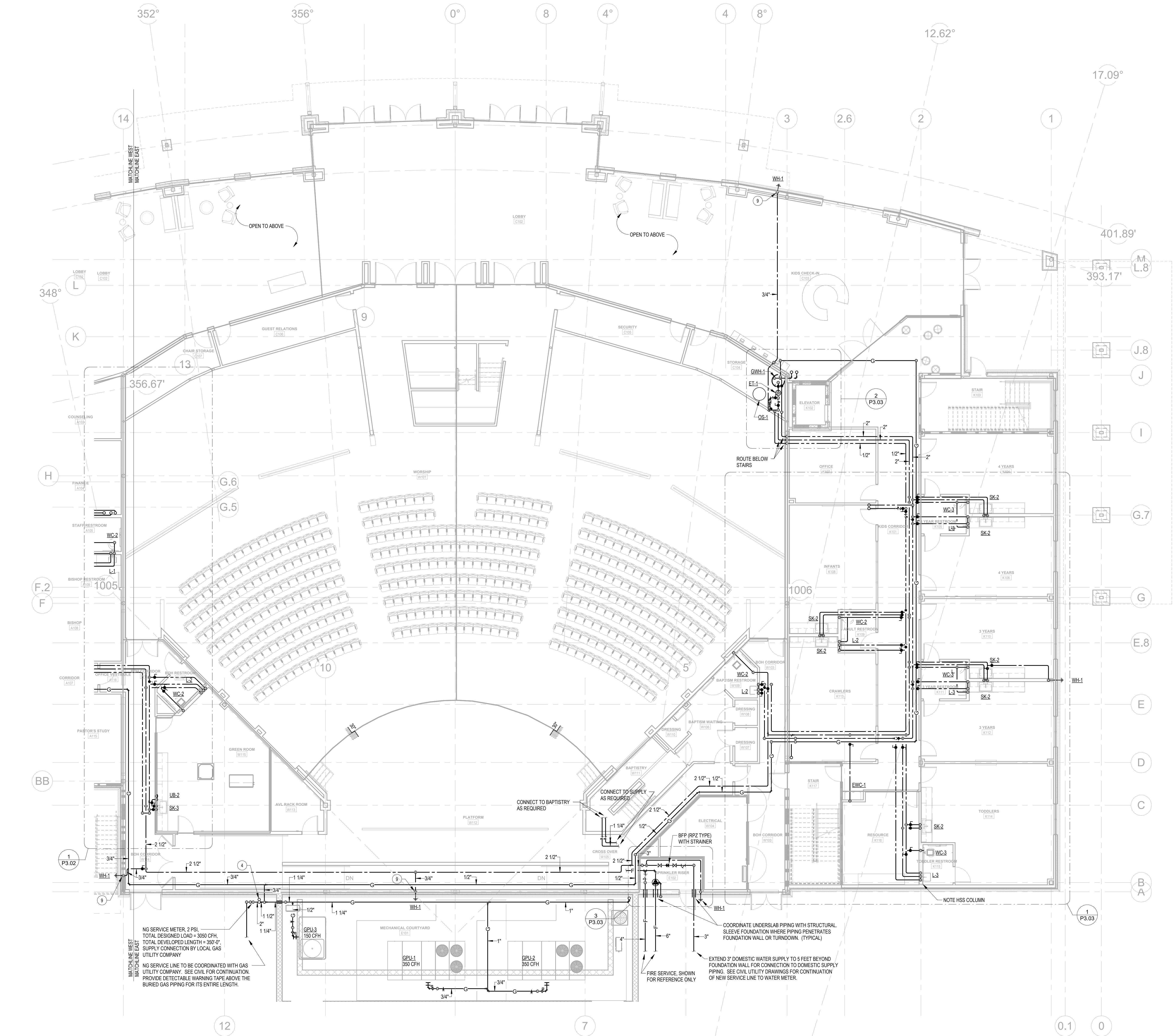
1 PLUMBING FIRST FLOOR PLAN - PRESSURE - EAST SIDE 1/8" = 1'-0"
