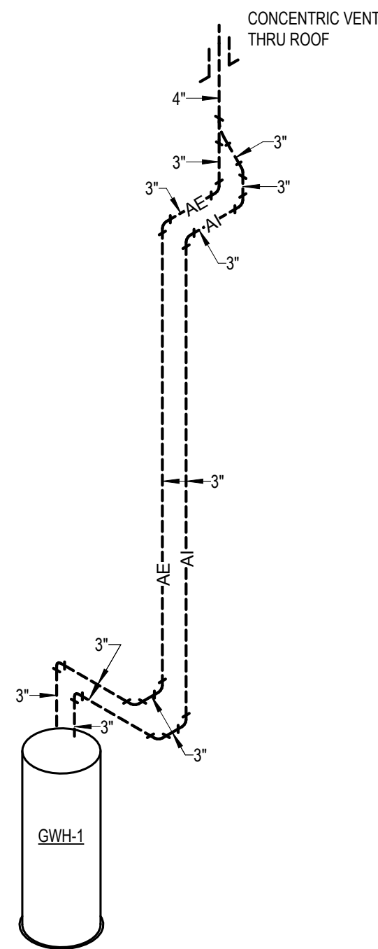
3 PLUMBING RISER DIAGRAM - GWH-1 VENTING
