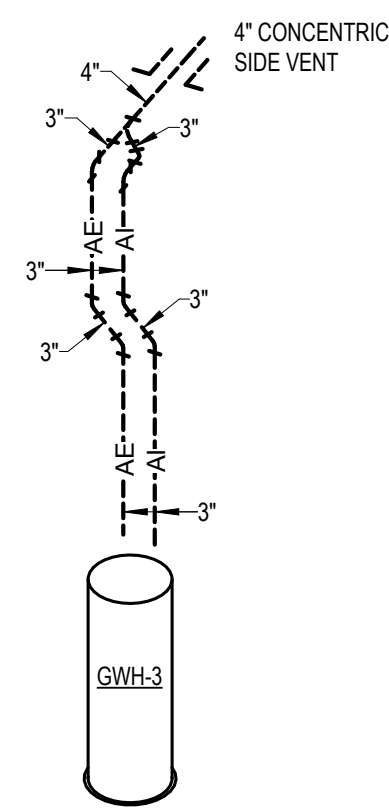
5 PLUMBING RISER DIAGRAM - GWH-3 VENTING
