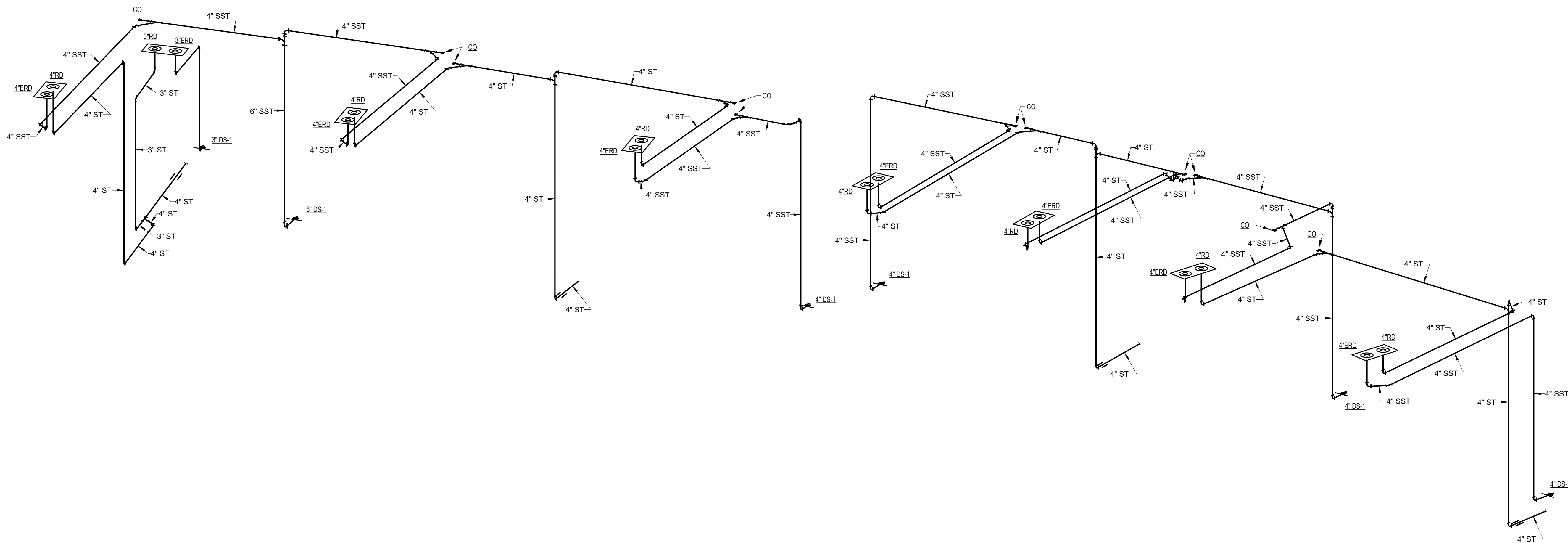
1 PLUMBING RISER DIAGRAM - STORM - EAST SIDE
