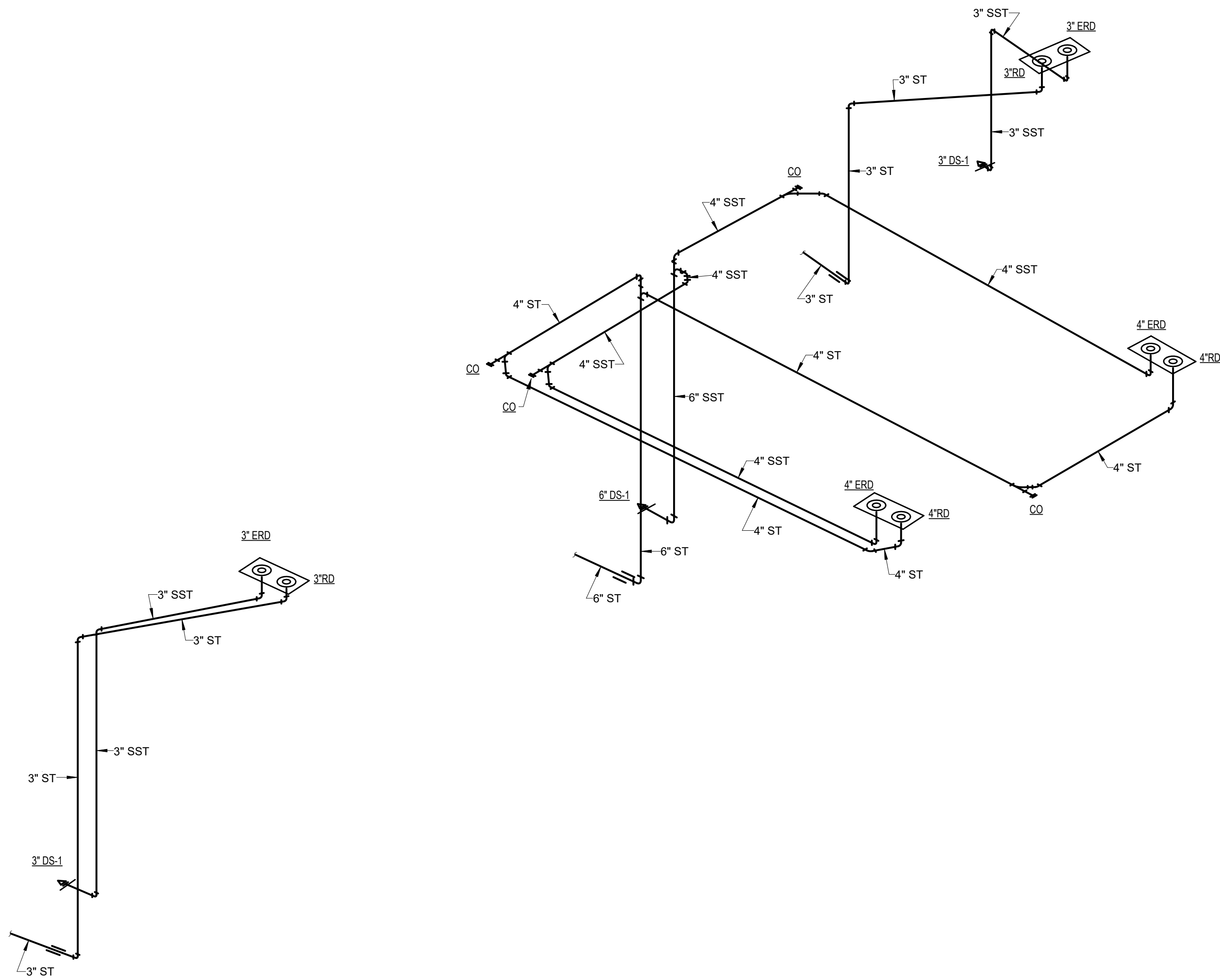
2 PLUMBING RISER DIAGRAM - STORM - WEST SIDE
