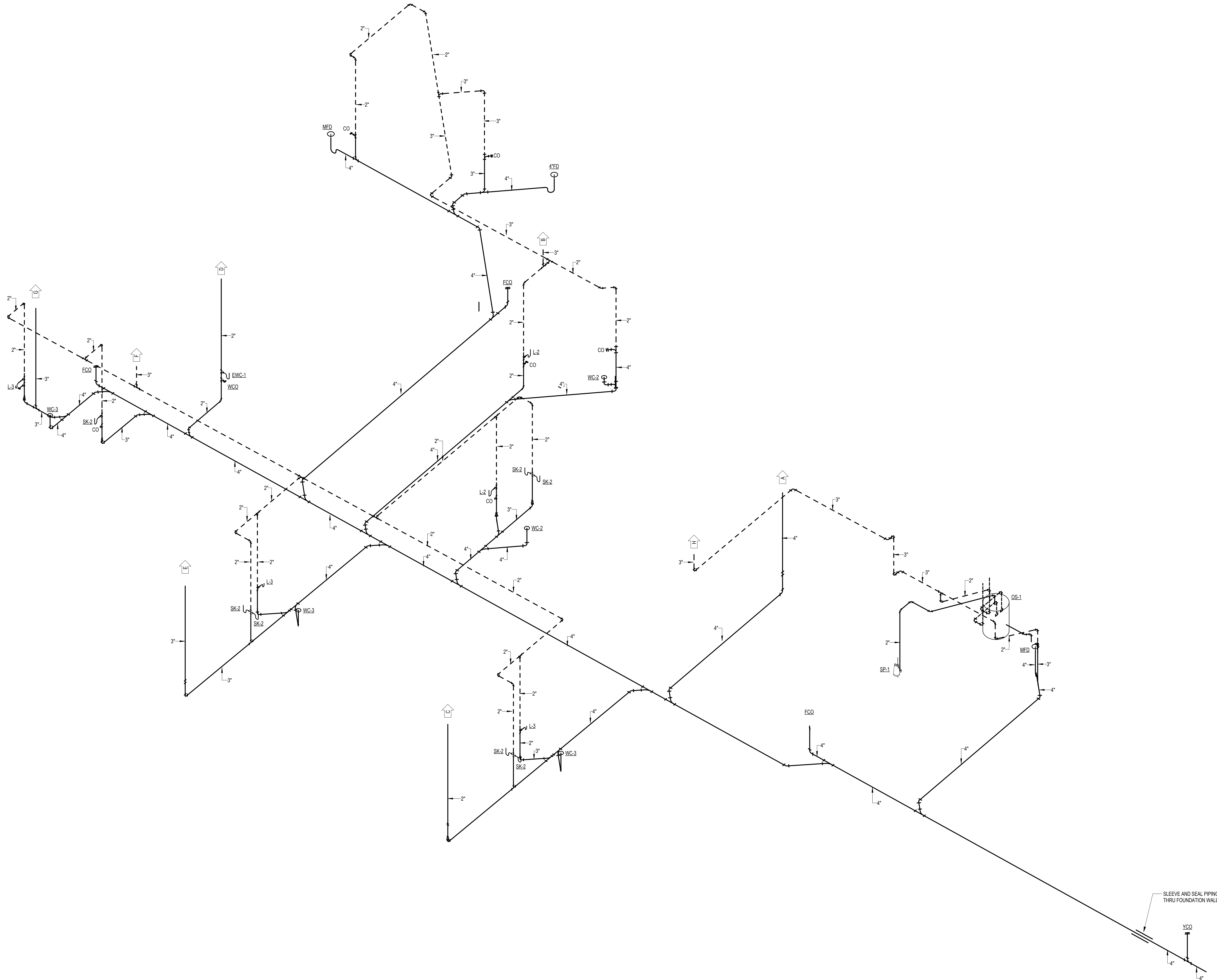
1 PLUMBING RISER DIAGRAM - FIRST FLOOR EAST SIDE - NON-PRESSURE
