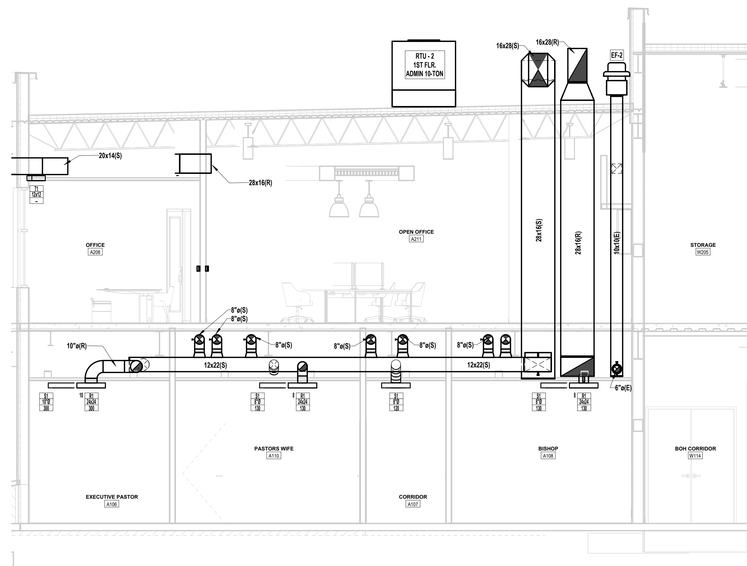
2 Section 17 1/4" = 1'-0"
