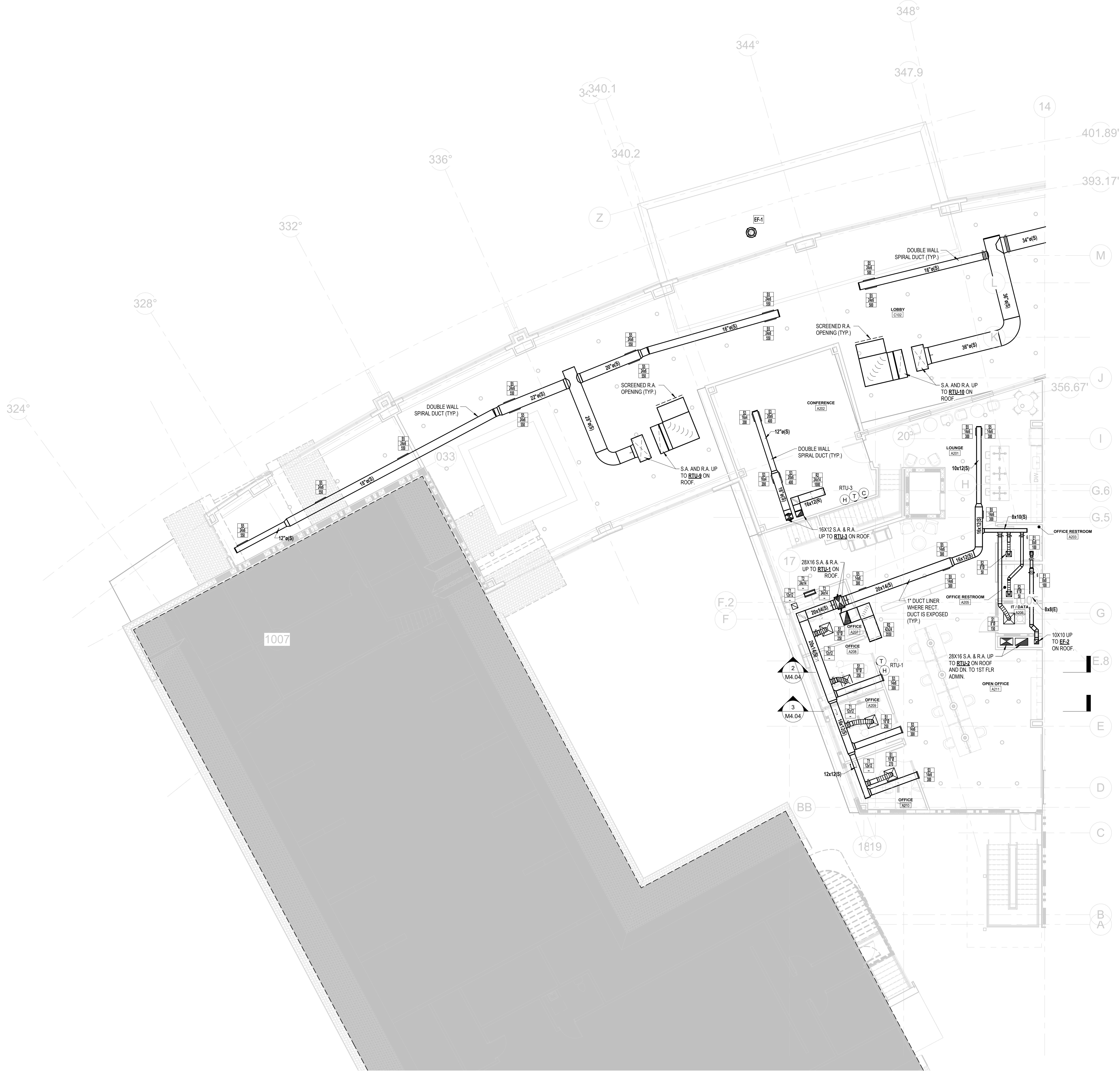
1 SECOND FLOOR PLAN - HVAC - WEST DUCTWORK 1/8" = 1'-0"
