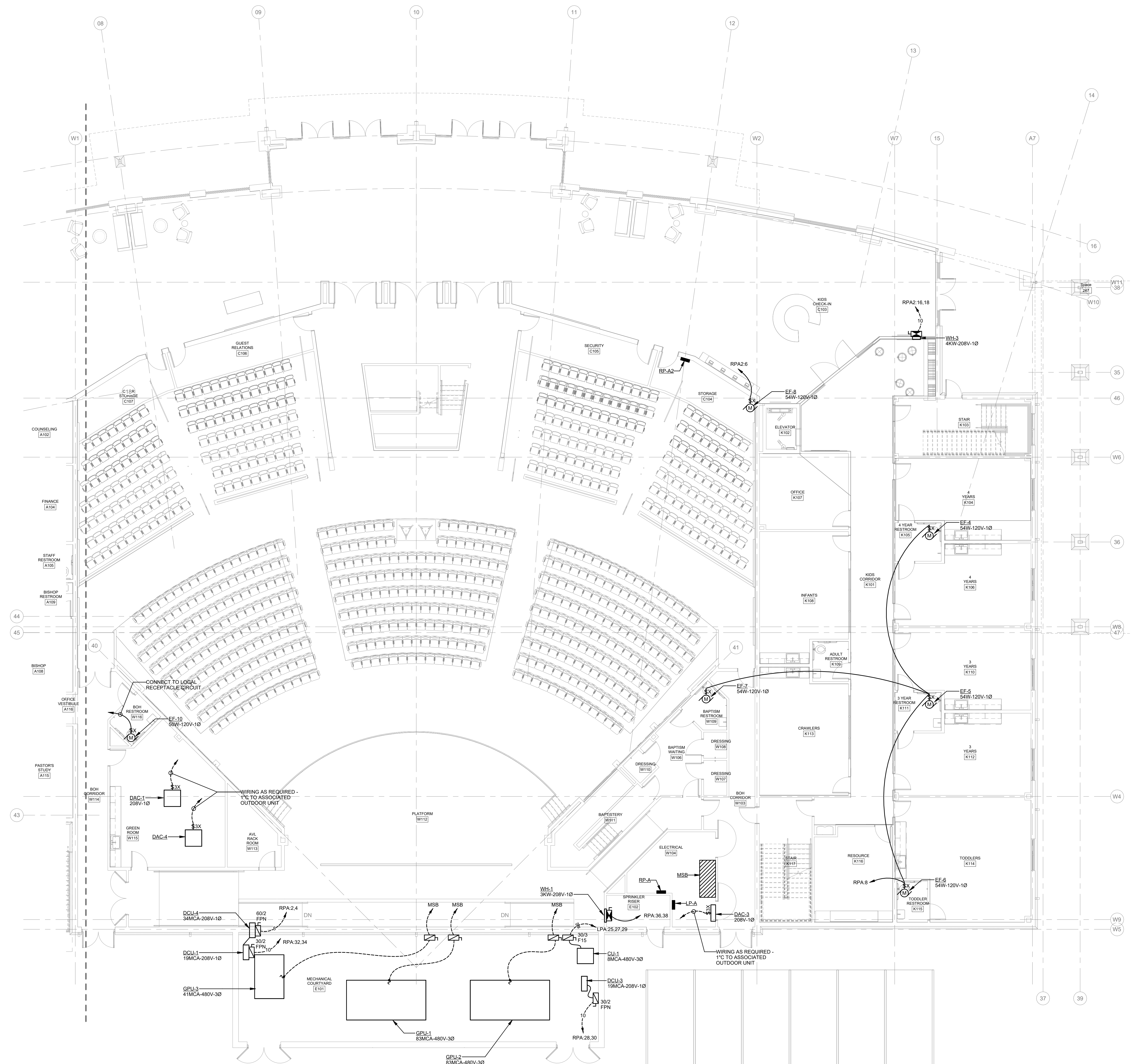
FIRST FLOOR HVAC ELECTRICAL PLAN - EAST SCALE: 1/8" = 1'-0"
