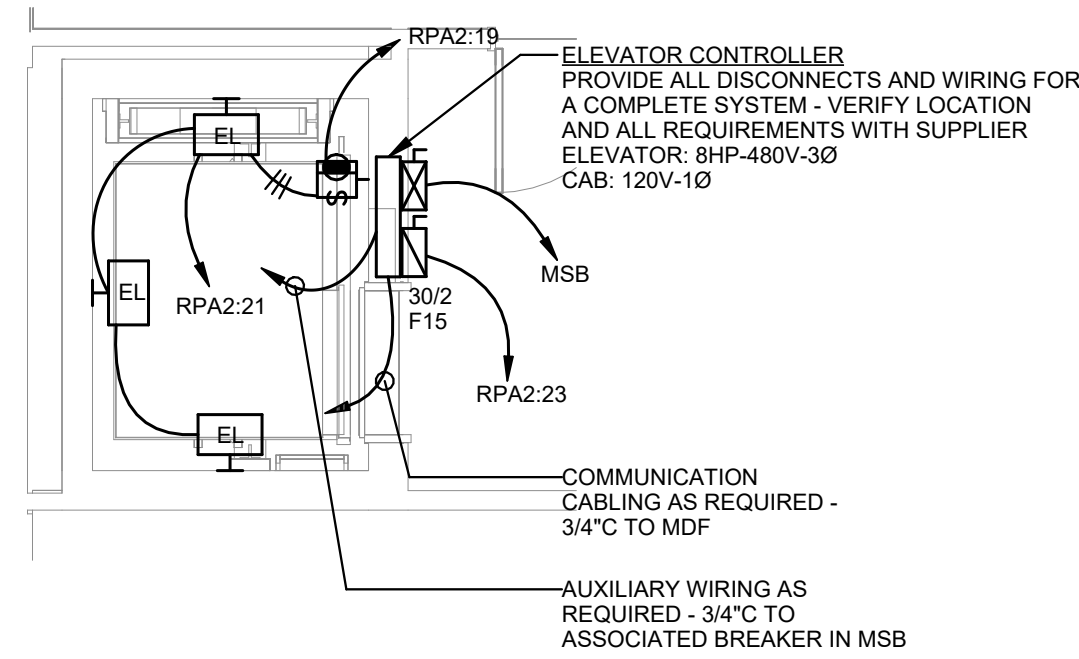
ENLARGED ELEVATOR SHAFT 1 POWER PLAN SCALE: 1/4" = 1'-0"
