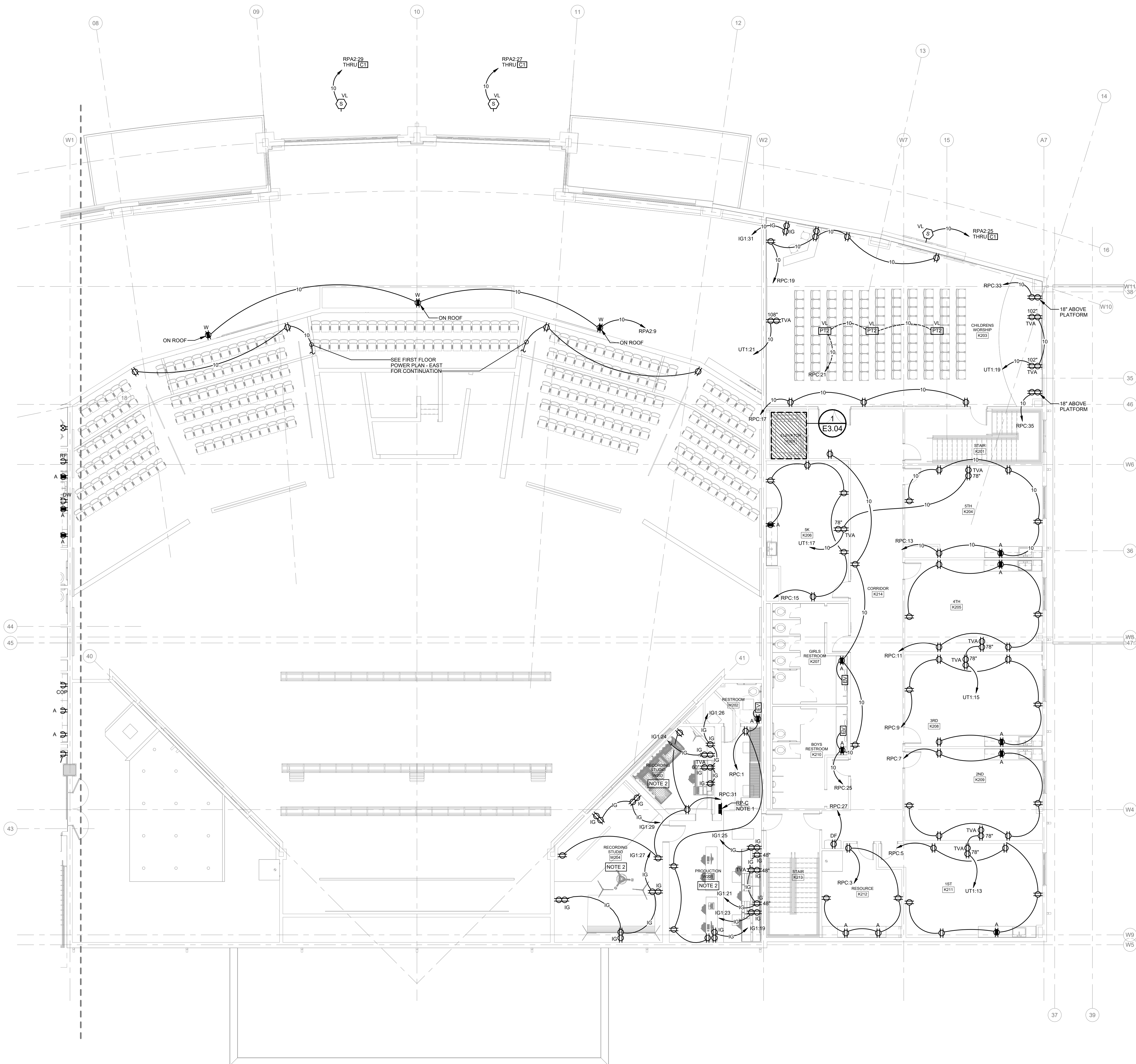
SECOND FLOOR POWER PLAN - EAST SCALE: 1/8" = 1'-0"
