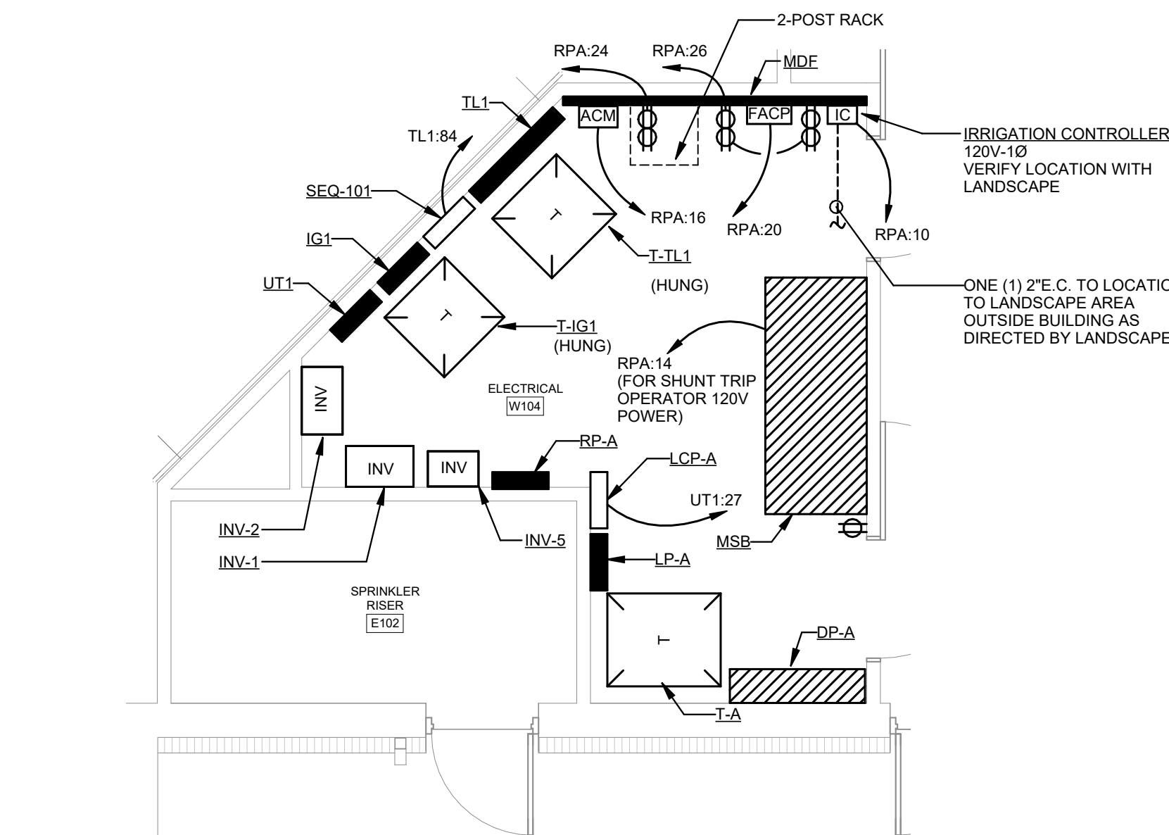
ENLARGED ELECTRICAL W104 POWER PLAN SCALE: 1/4" = 1'-0"
