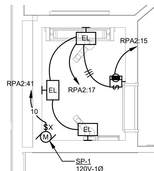
ENLARGED ELEVATOR K102 PIT POWER PLAN SCALE: 1/4" = 1'-0"
