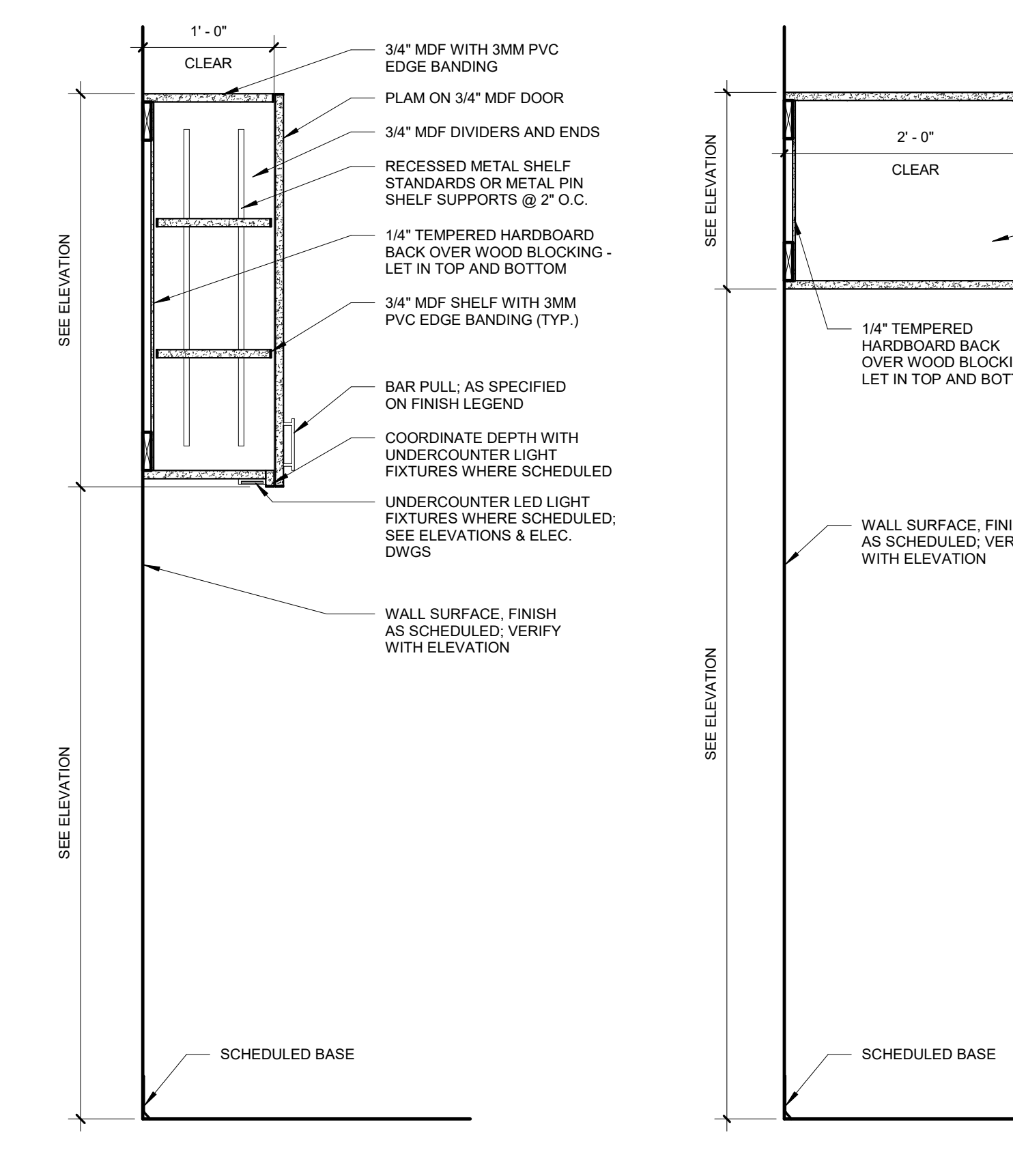
4 WALL CABS - DOORS 1" = 1'-0"
