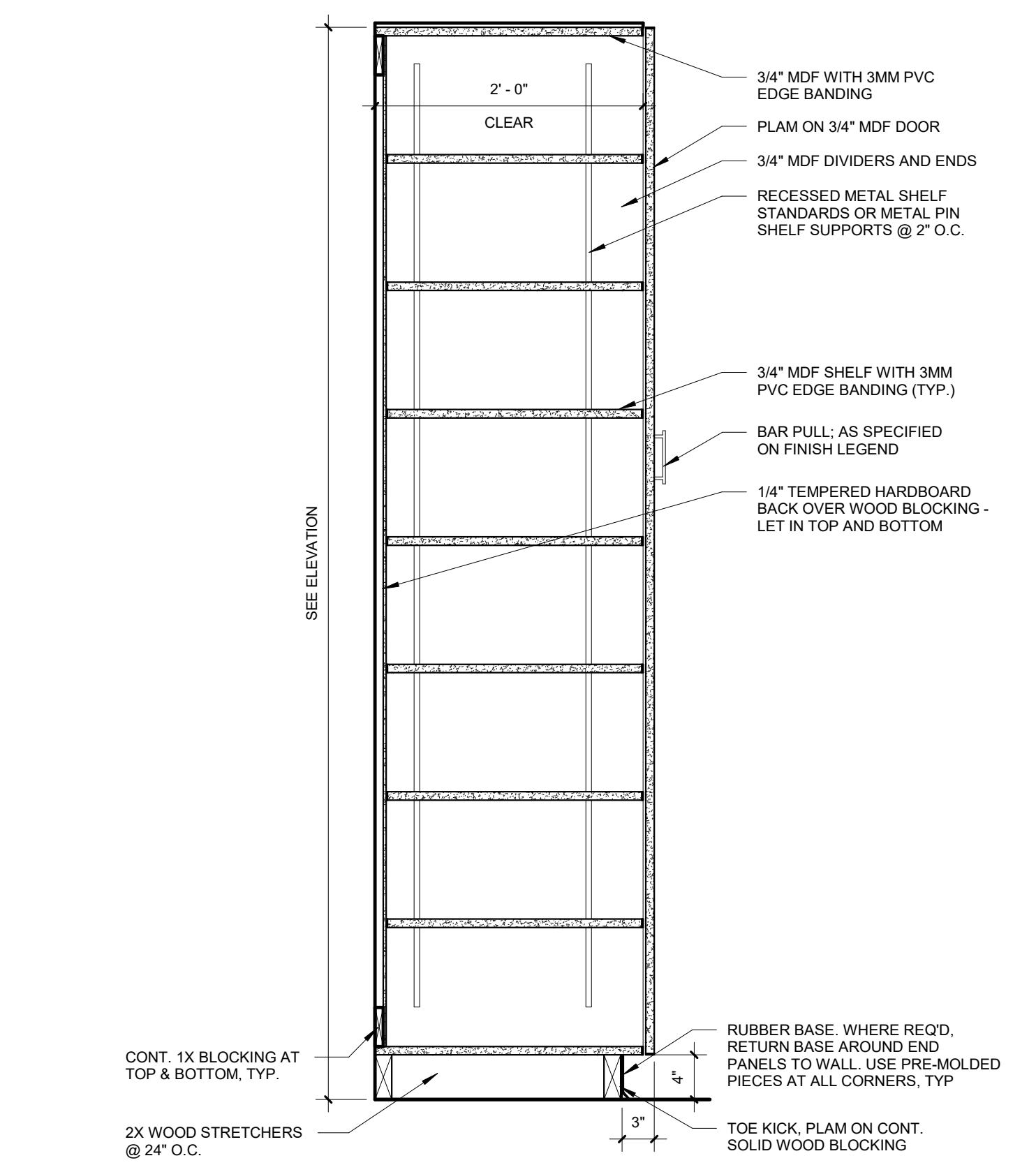
6 BASE CABS - FULL HEIGHT DOORS 1" = 1'-0"
