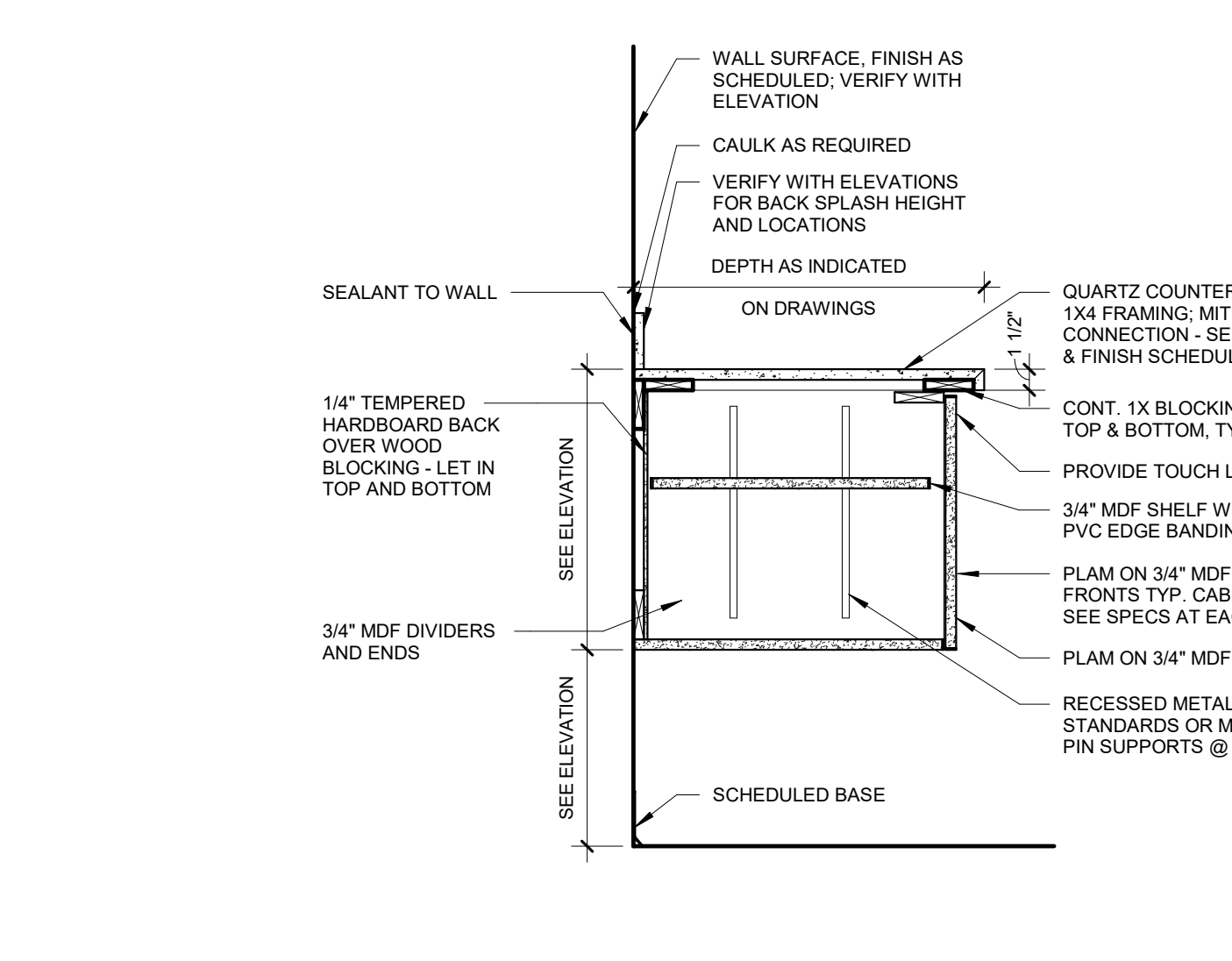
14 BASE CABS - FLOATING DOORS - QZ CTR 1" = 1'-0"
