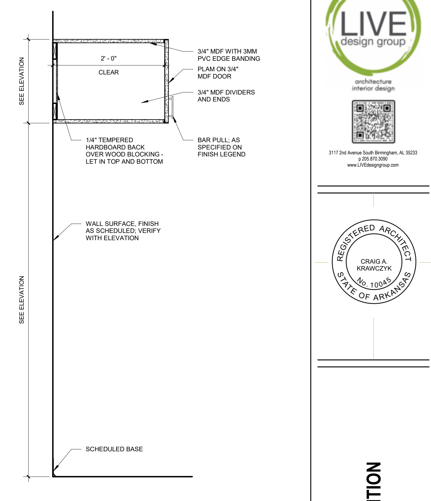
5 WALL CABS - ABOVE FRIDGE DOORS 1" = 1'-0"
