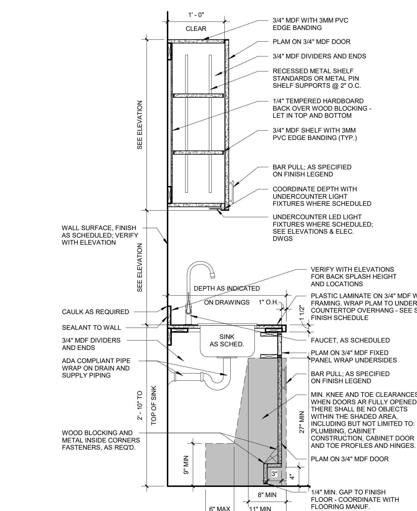
3 BASE & WALL CAB - @ ADA SINK - PLAM CTR 1" = 1'-0"
