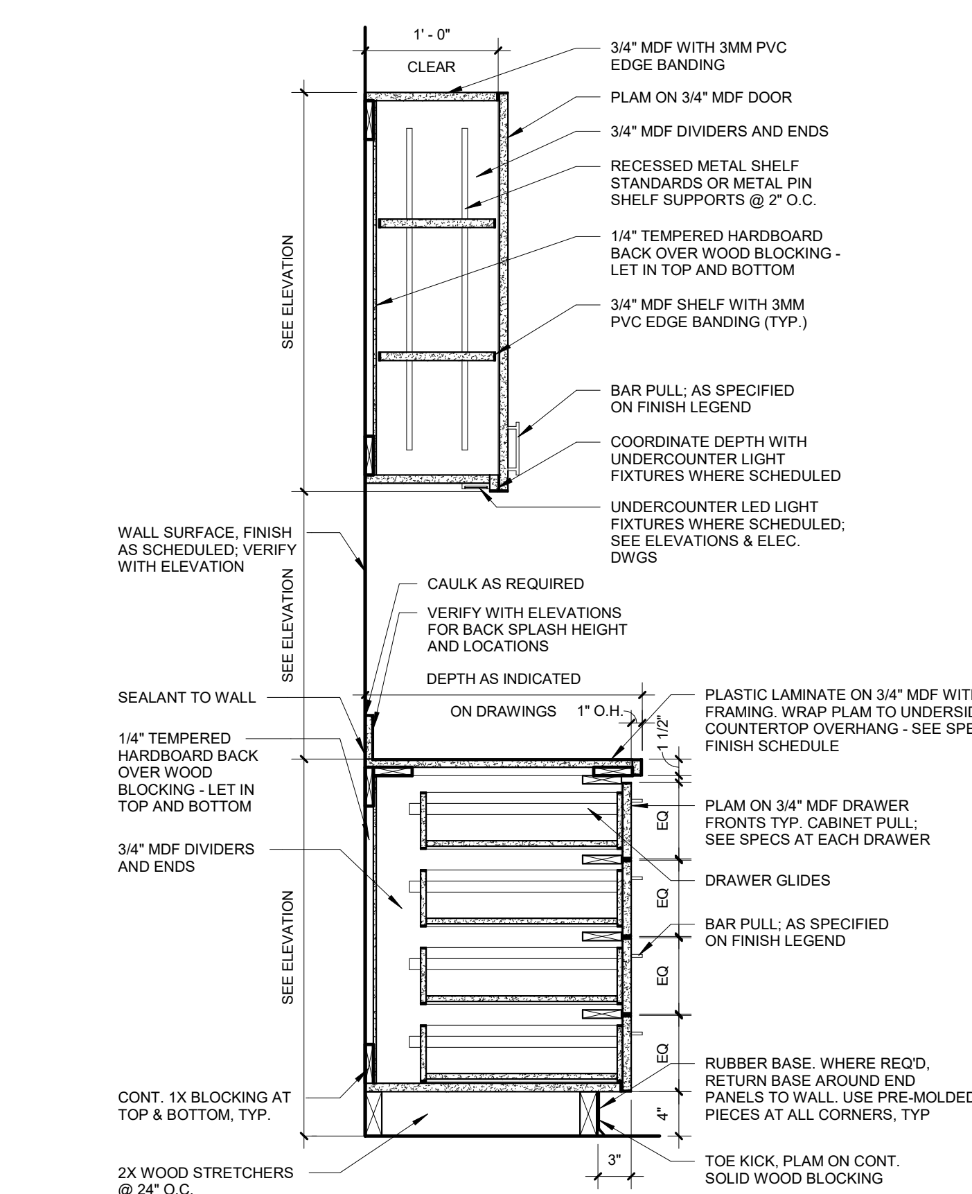
2 BASE & WALL CAB - 4 EQ DWRS - PLAM CTR 1" = 1'-0"
