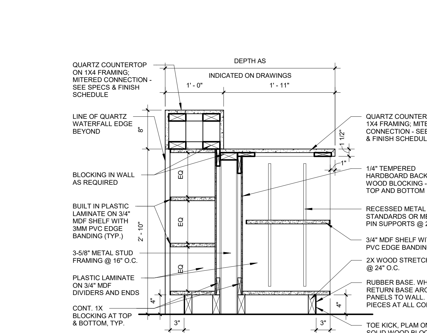
13 CAFE MERCH SHELVES - QTZ CTR 1" = 1'-0"
