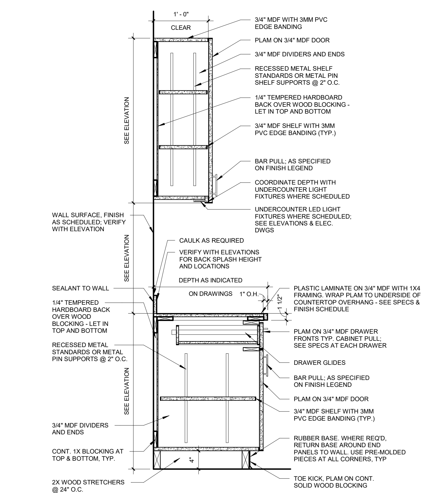
1 BASE & WALL CAB - DOORS & DWR - PLAM CTR 1" = 1'-0"
