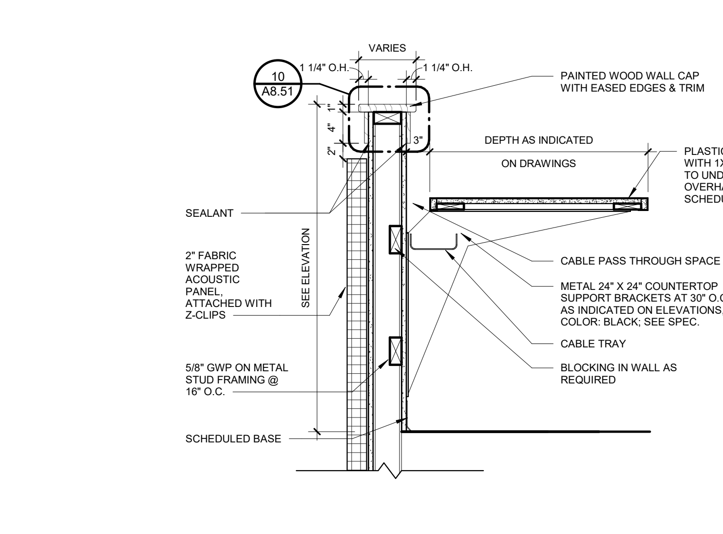
15 SOUND BOOTH - PLAM CTR 1" = 1'-0"
