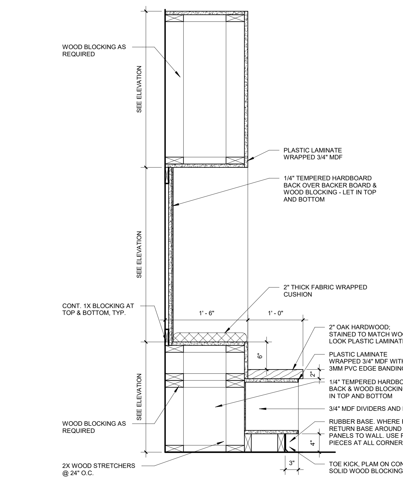
7 BASE CABS - KIDS BENCH 1" = 1'-0"
