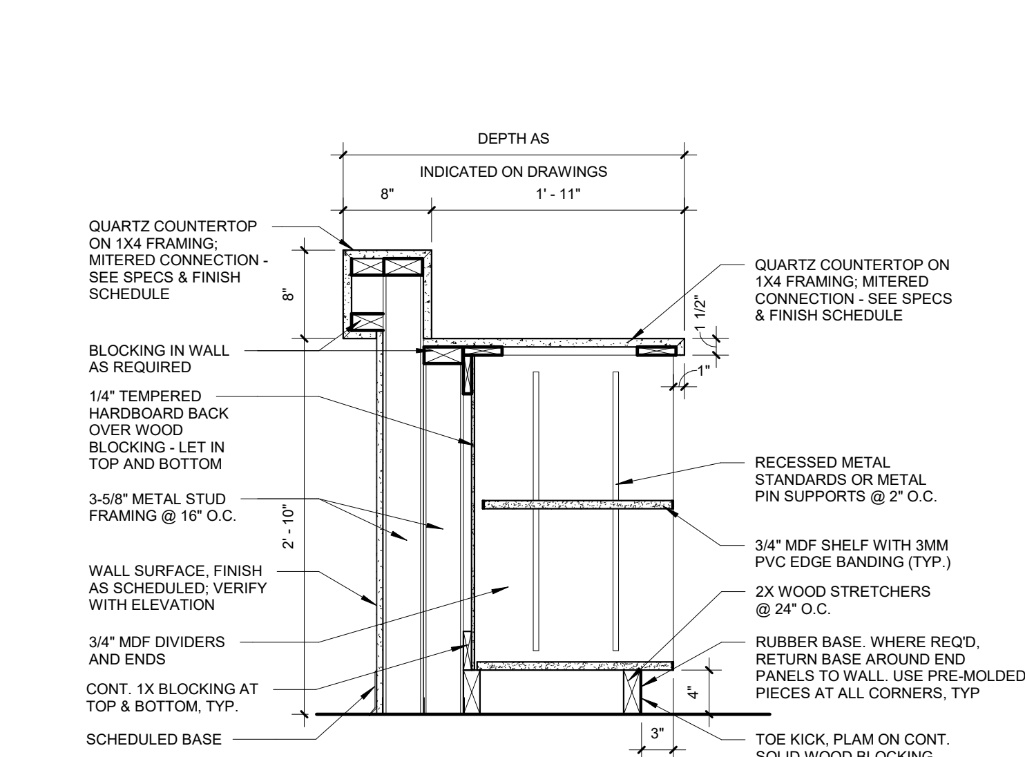
12 CAFE FRONT TRANSACTION - QTZ CTR 1" = 1'-0"
