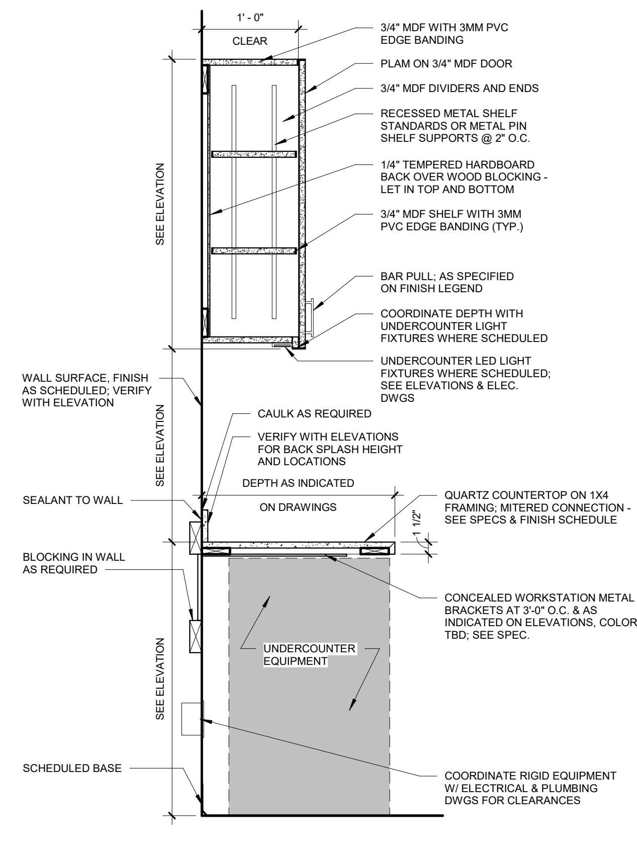
8 WALL & BASE CABS - UC EQUIPMENT - QZ CTR 1" = 1'-0"
