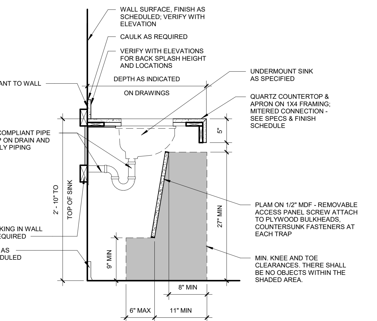
9 VANITY BASE CABS - APRON & SINK - QZ CTR 1" = 1'-0"
