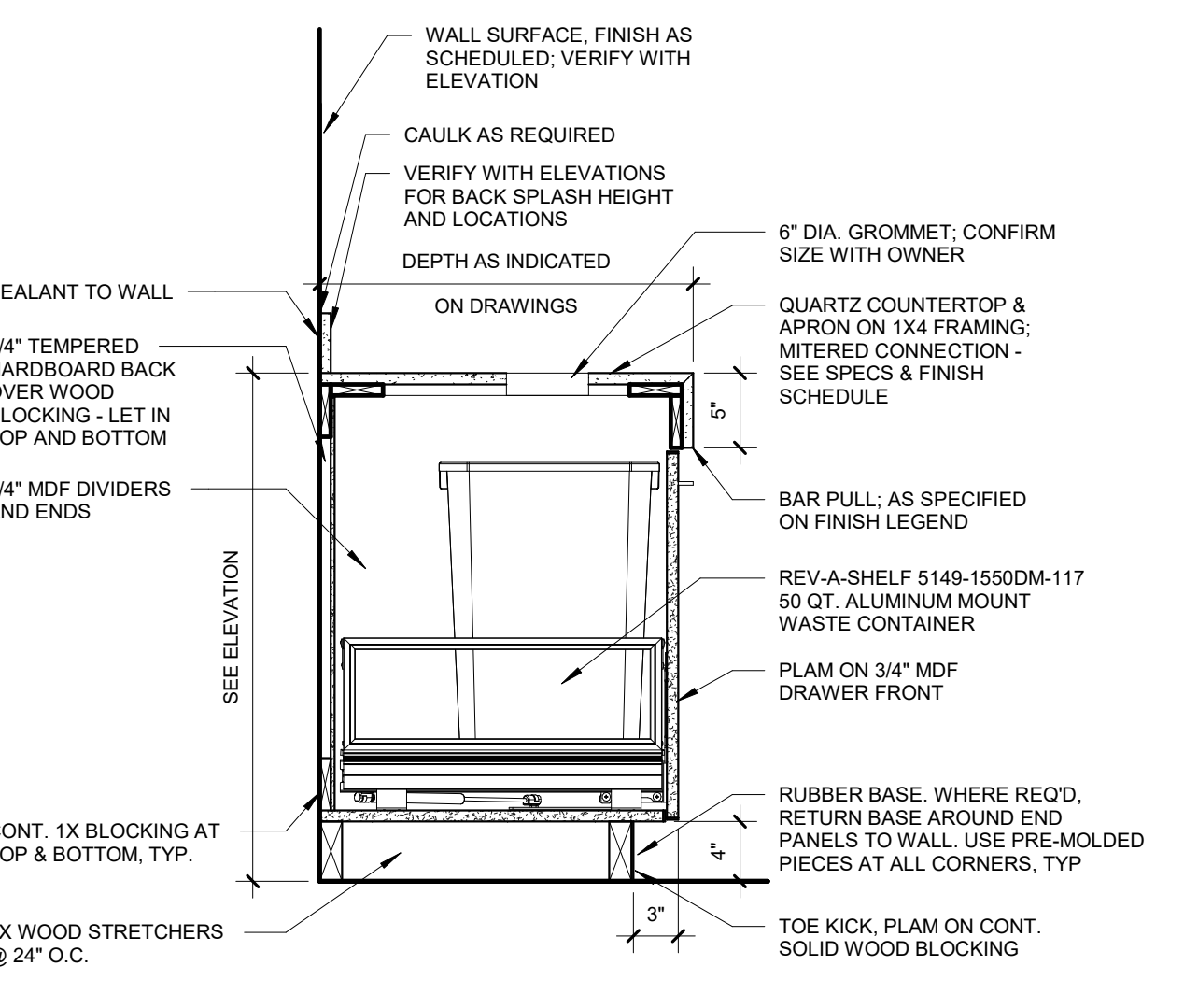
10 VANITY BASE CABS - TRASH DWR - QZ CTR 1" = 1'-0"
