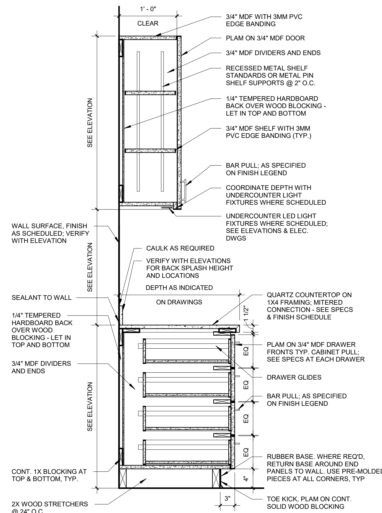
6 WALL & BASE CABS - ALL EQ DRAWERS - QZ CTR 1" = 1'-0"
