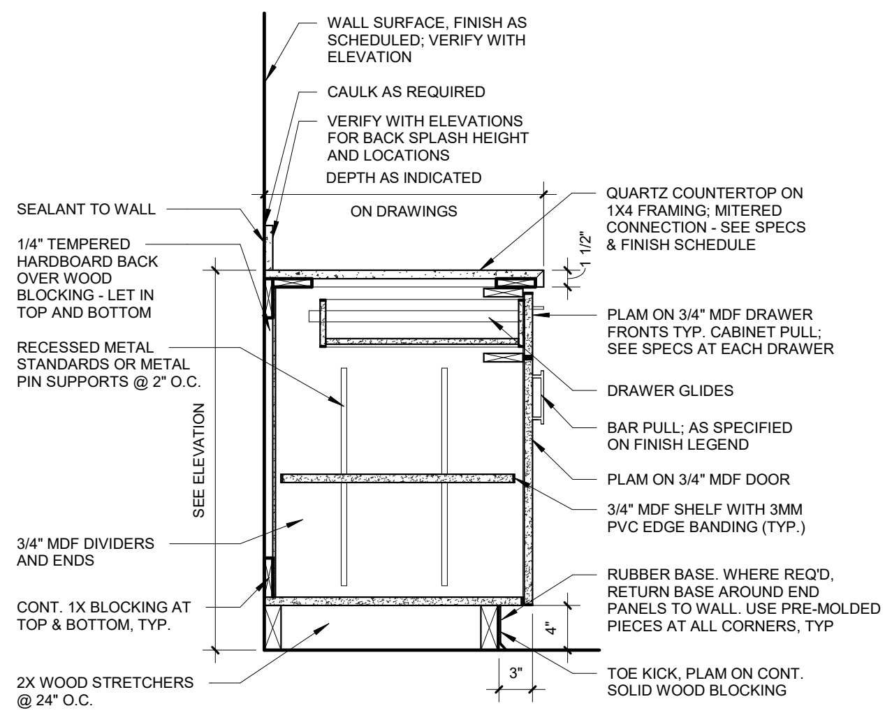
1 BASE CABS - DOORS & DWR - QZ CTR 1" = 1'-0"
