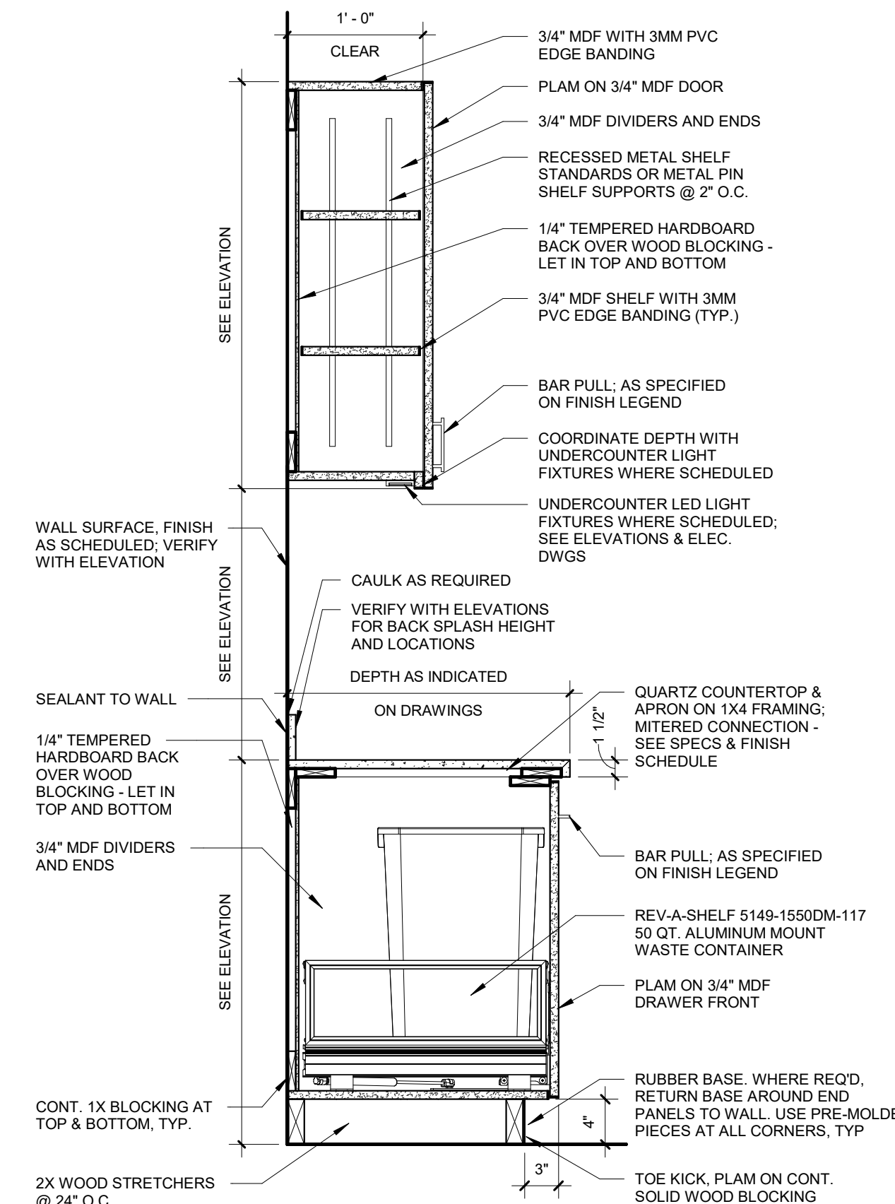
7 WALL & BASE CABS - TRASH DWR - QZ CTR 1" = 1'-0"
