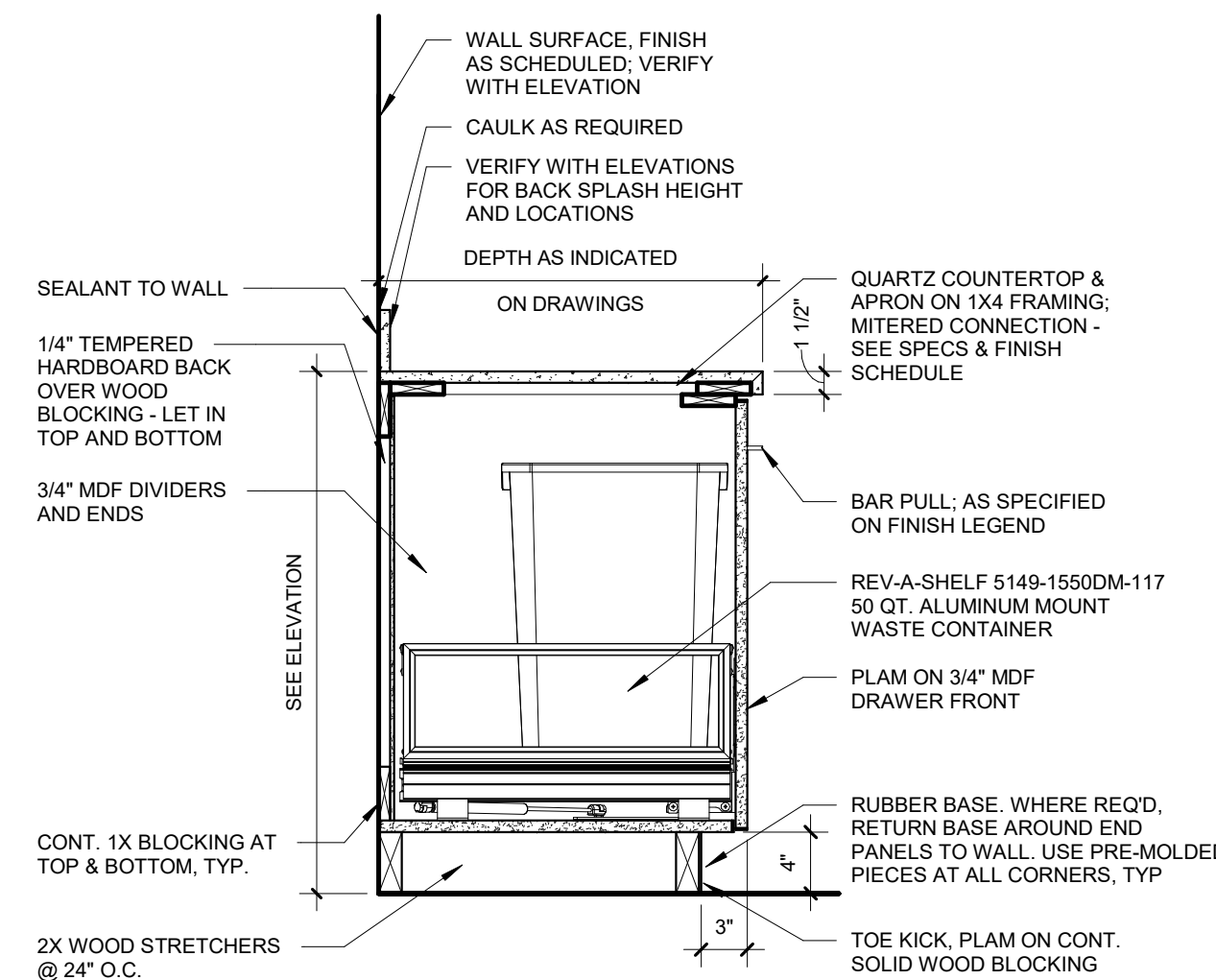
3 BASE CABS - TRASH DRAWER - QZ CTR 1" = 1'-0"
