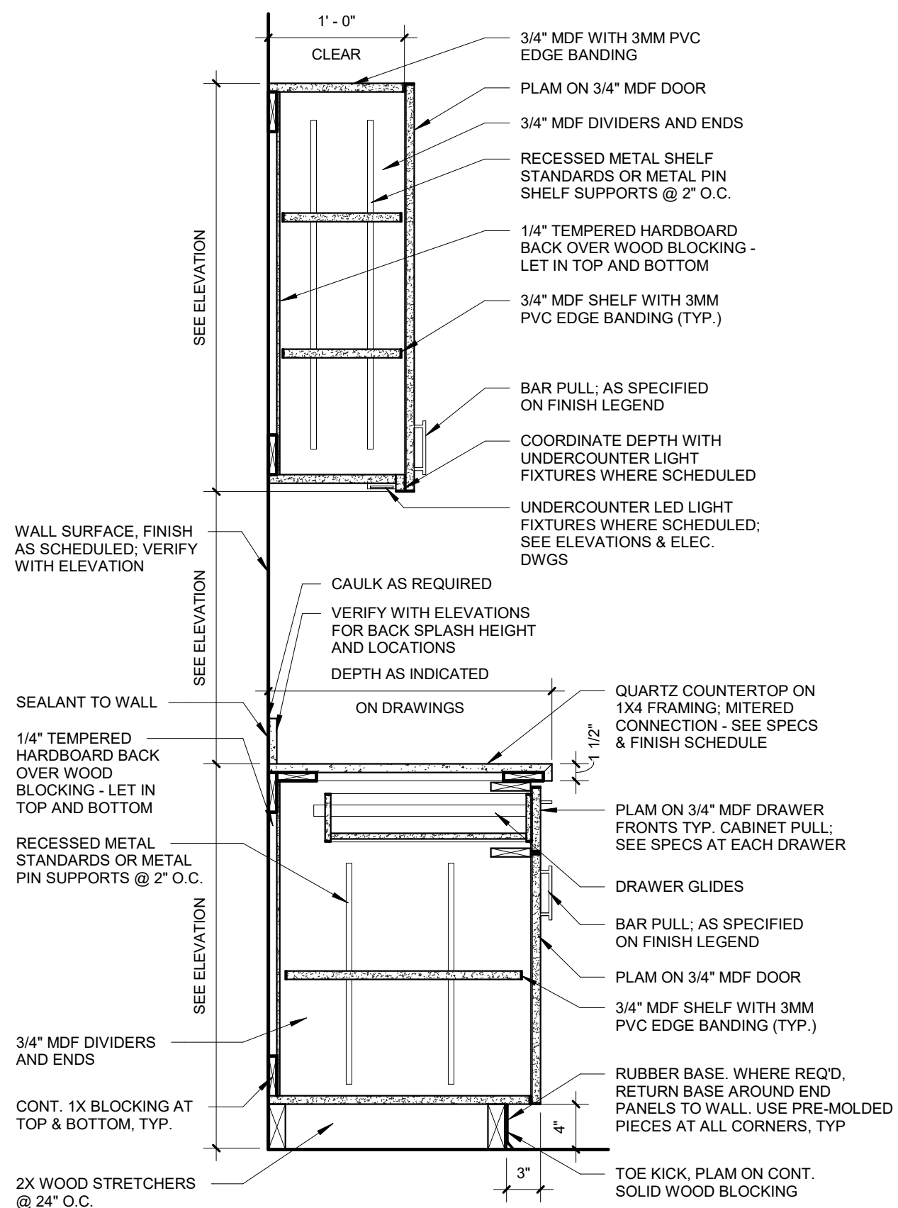
5 WALL & BASE CABS - DOORS & DWR - QZ CTR 1" = 1'-0"
