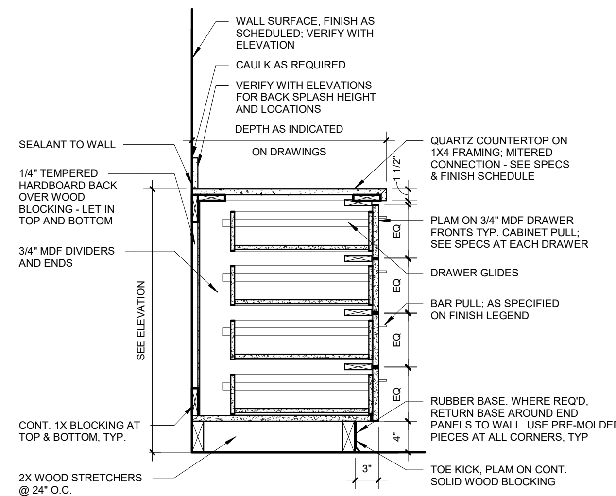
2 BASE CABS - ALL EQ DRAWERS - QZ CTR 1" = 1'-0"
