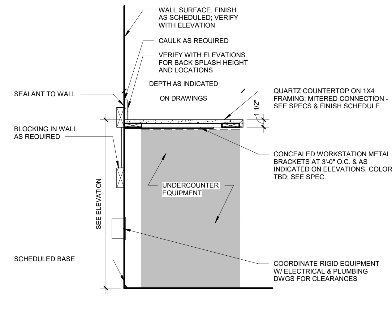
4 BASE CABS - UC EQUIPMENT - QZ CTR 1" = 1'-0"
