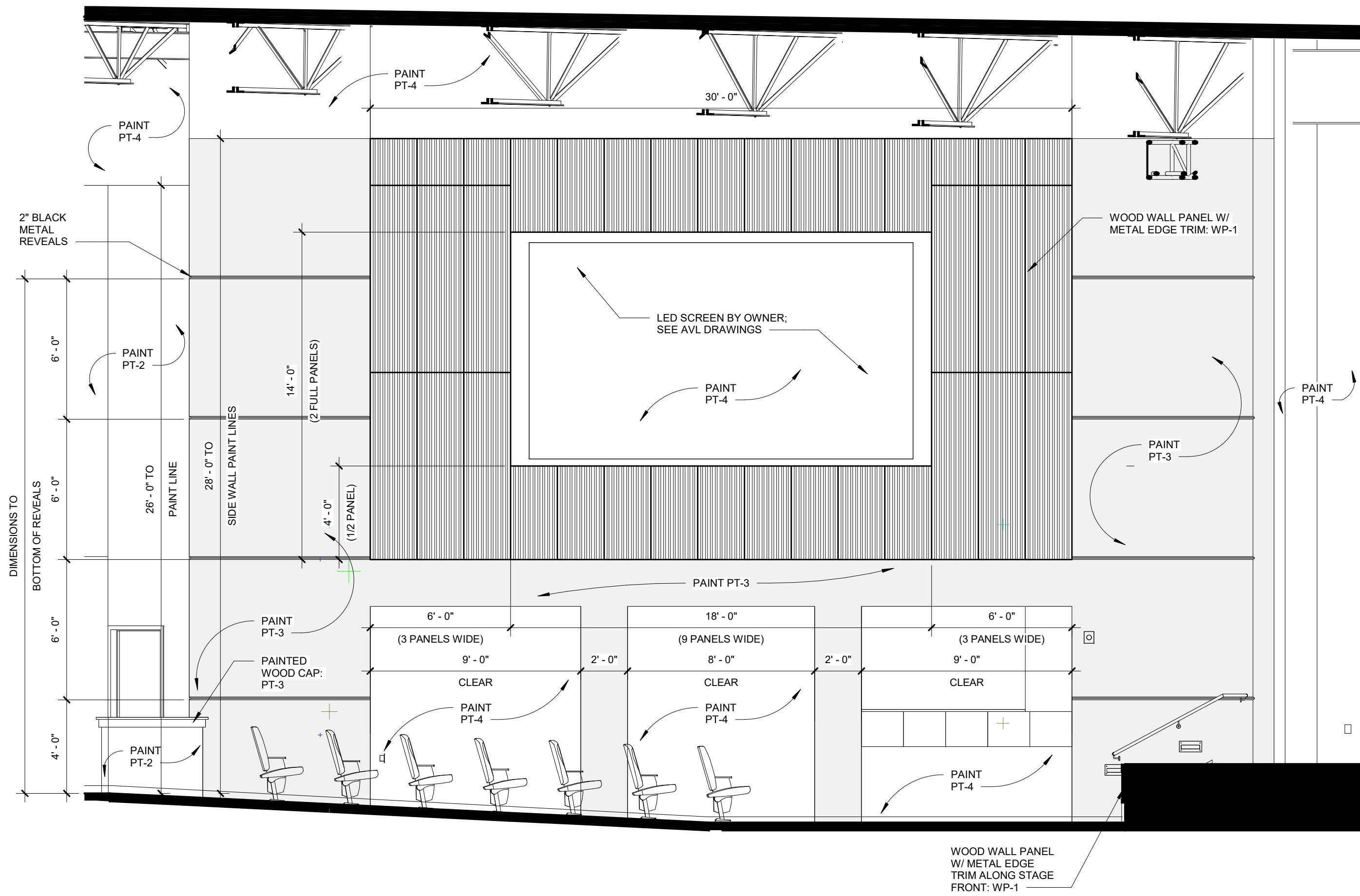
2 WORSHIP - 02 1/4" = 1'-0"
