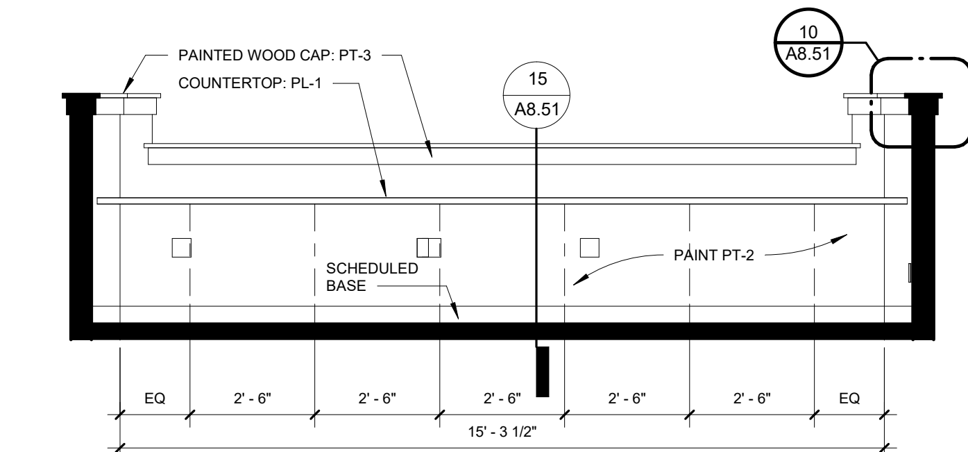
4 AUDIO BOOTH - 01 3/8" = 1'-0"
