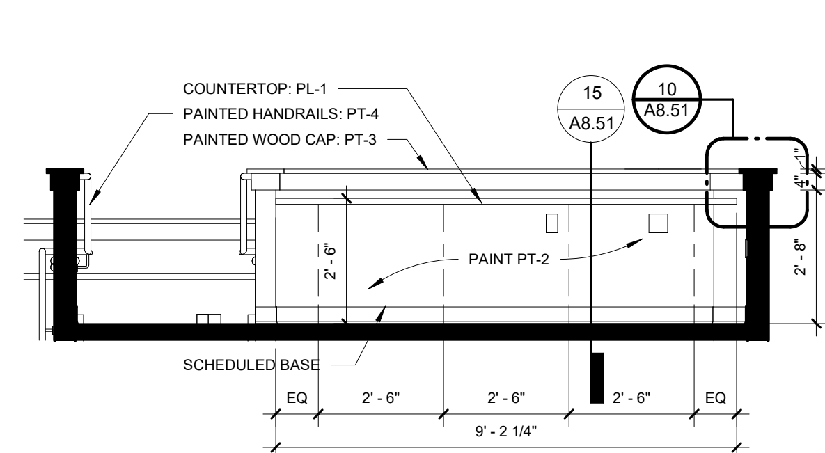
5 AUDIO BOOTH - 02 3/8" = 1'-0"
