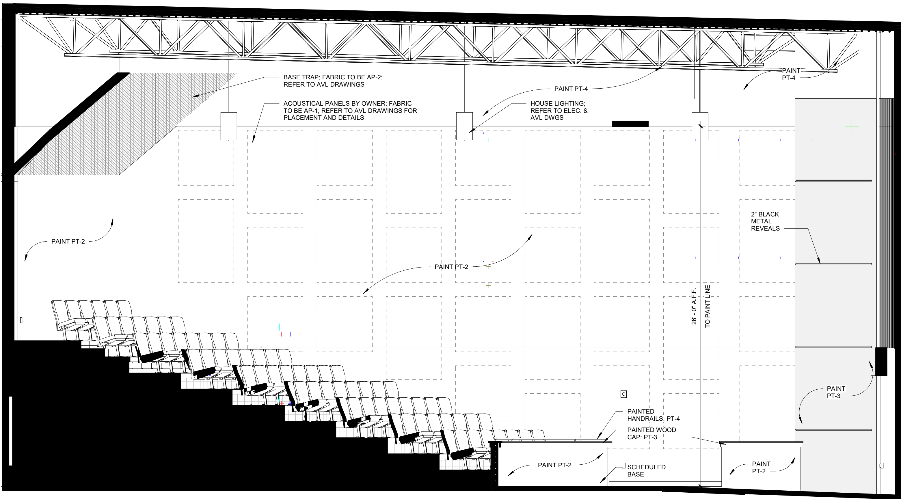
1 WORSHIP - 03 1/4" = 1'-0"
