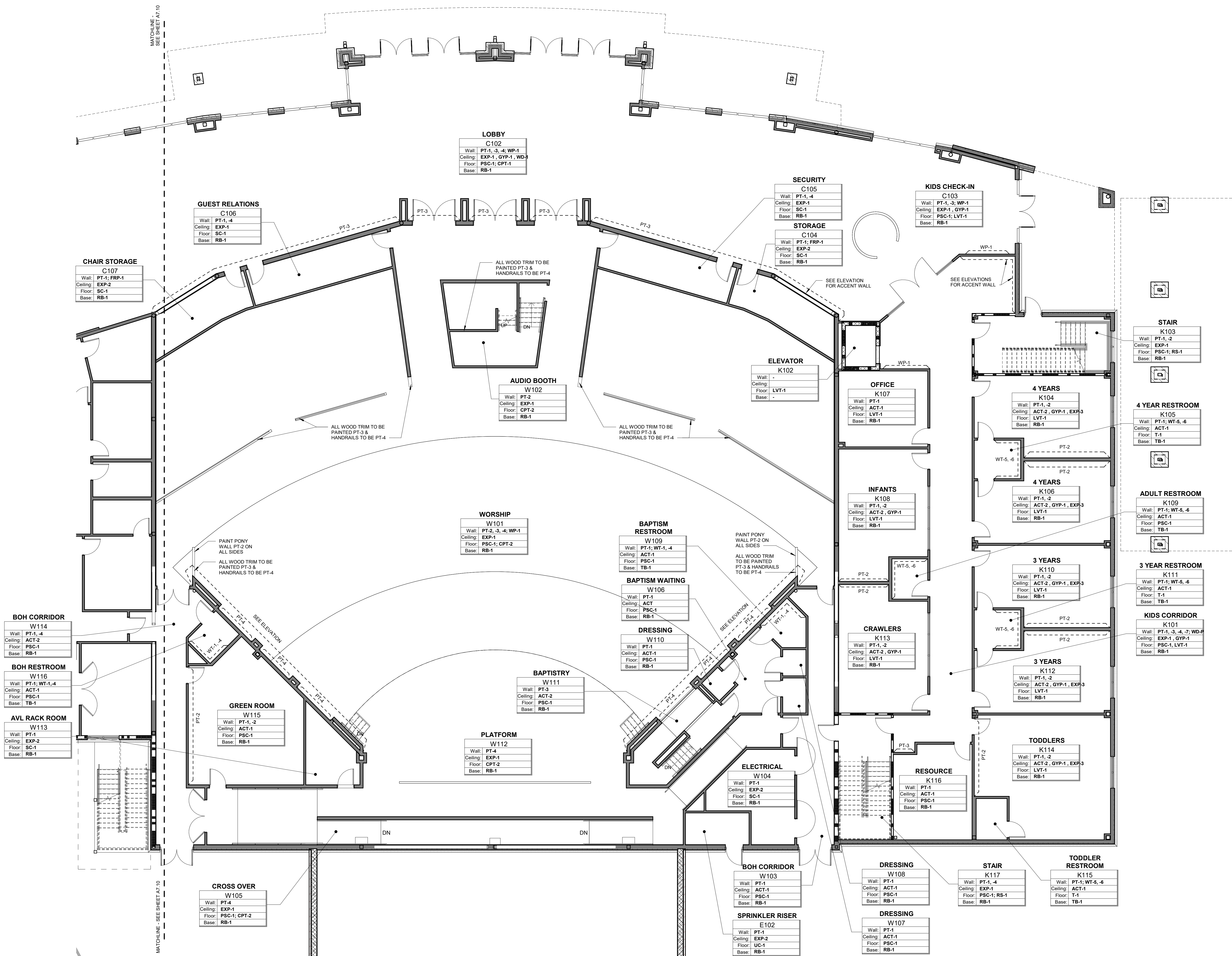
1 FIRST FLOOR FINISH PLAN - EAST 1/8" = 1'-0"
