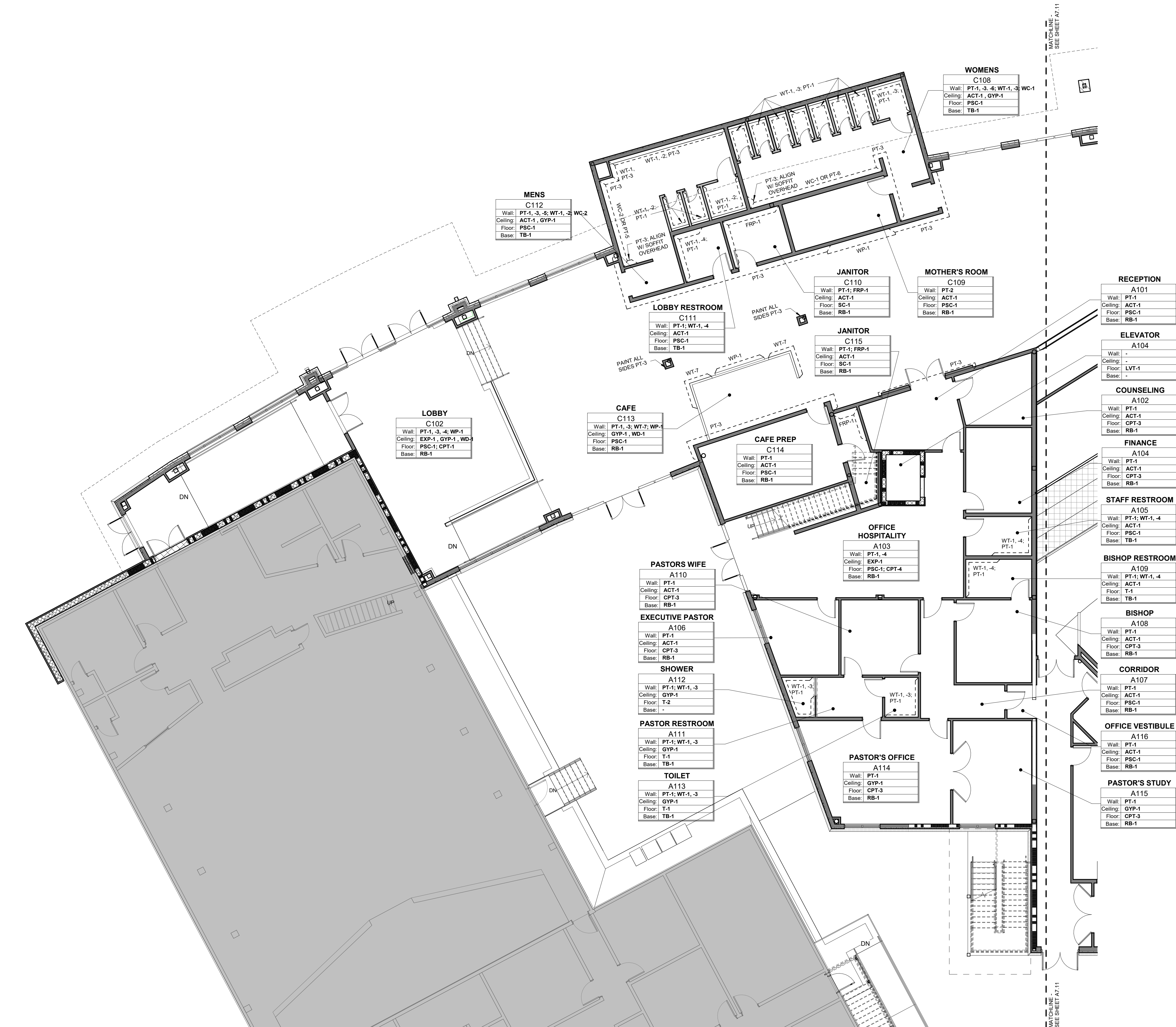
1 FIRST FLOOR FINISH PLAN - WEST 1/8" = 1'-0"
