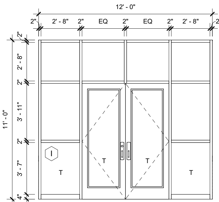
9 STOREFRONT ELEVATION I 1/4" = 1'-0"
