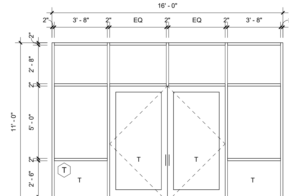
20 STOREFRONT ELEVATION T 1/4" = 1'-0"
