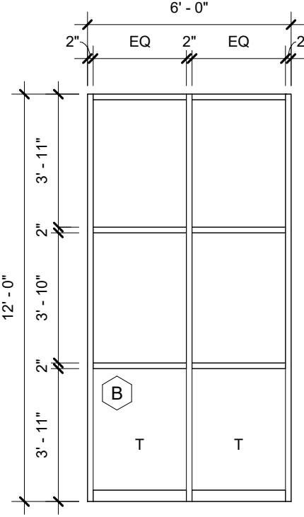
2 STOREFRONT ELEVATION B 1/4" = 1'-0"
