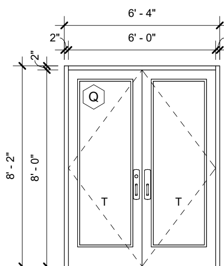
17 STOREFRONT ELEVATION Q 1/4" = 1'-0"
