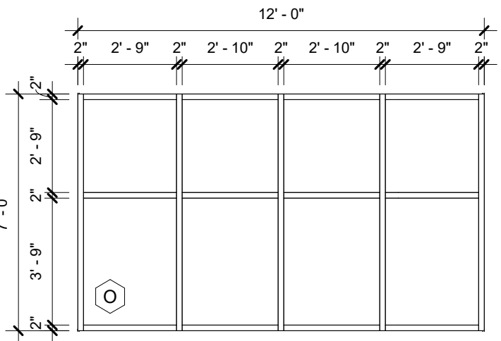
15 STOREFRONT ELEVATION O 1/4" = 1'-0"
