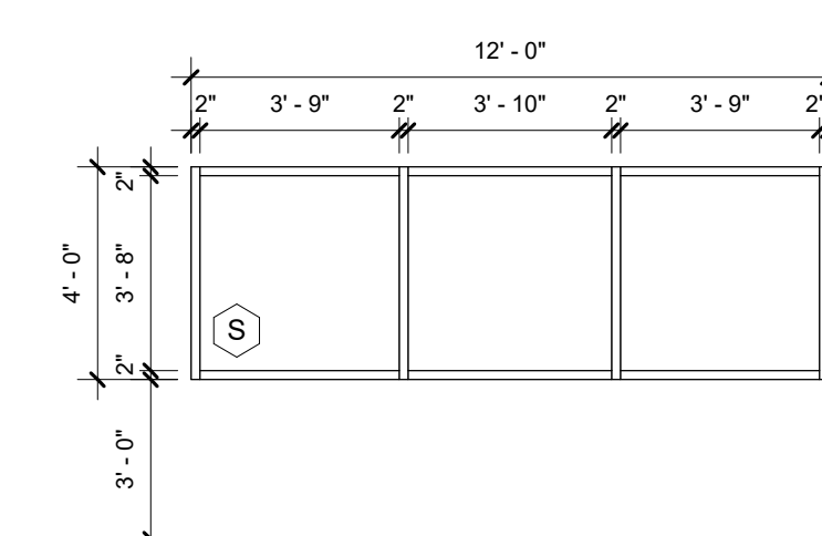
19 STOREFRONT ELEVATION S 1/4" = 1'-0"
