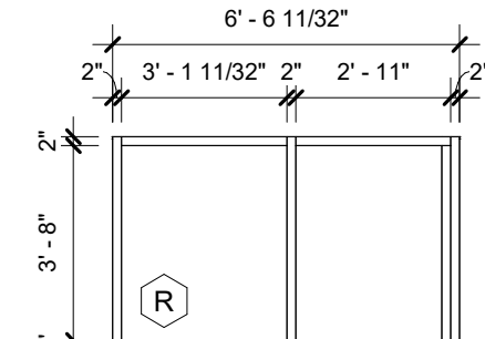
18 STOREFRONT ELEVATION R 1/4" = 1'-0"
