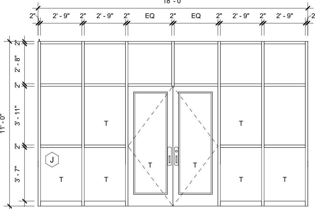
10 STOREFRONT ELEVATION J 1/4" = 1'-0"
