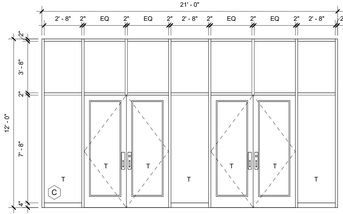
3 STOREFRONT ELEVATION C 1/4" = 1'-0"
