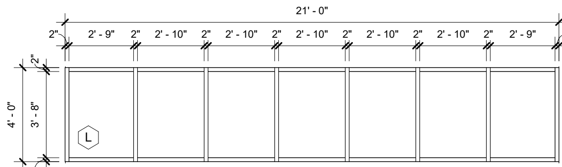
12 STOREFRONT ELEVATION L 1/4" = 1'-0"
