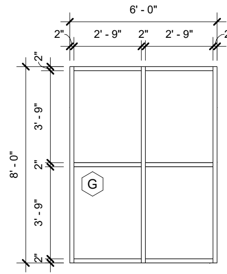
7 STOREFRONT ELEVATION G 1/4" = 1'-0"
