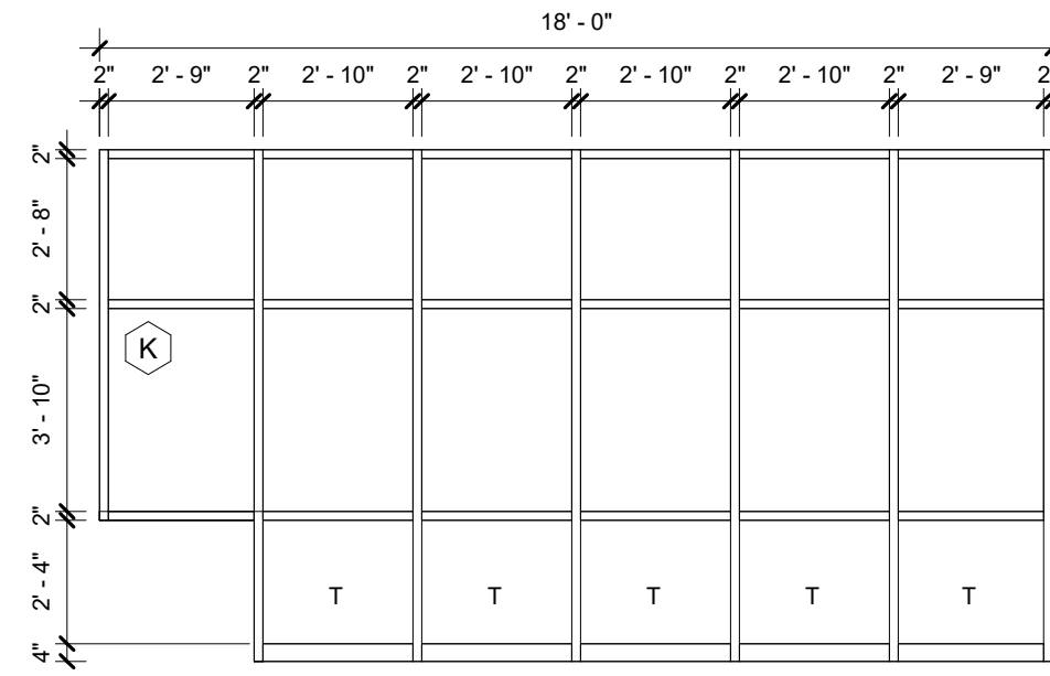
11 STOREFRONT ELEVATION K 1/4" = 1'-0"
