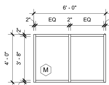
13 STOREFRONT ELEVATION M 1/4" = 1'-0"
