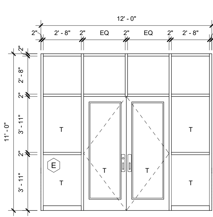
5 STOREFRONT ELEVATION E 1/4" = 1'-0"
