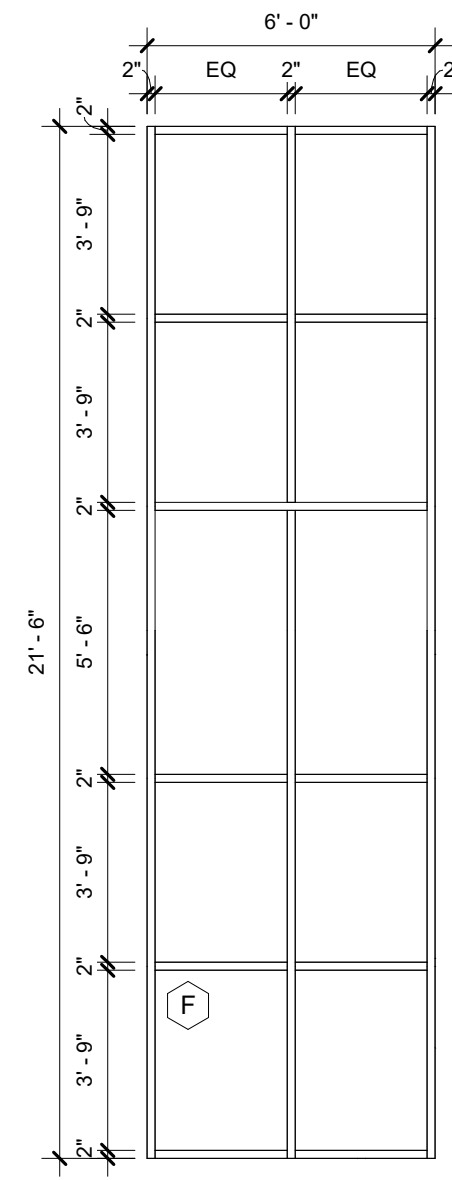
6 CURTAINWALL ELEVATION F 1/4" = 1'-0"
