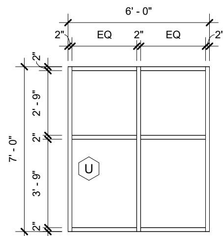
8 STOREFRONT ELEVATION H (FIRE RATED) 1/4" = 1'-0"
