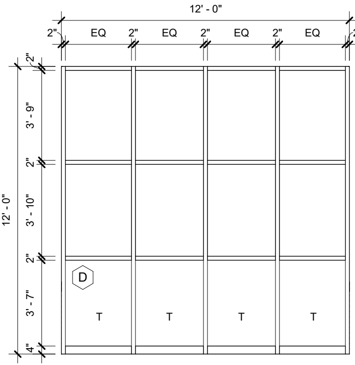
4 STOREFRONT ELEVATION D 1/4" = 1'-0"
