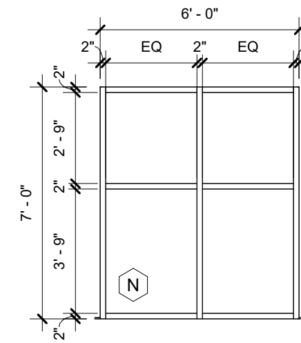
14 STOREFRONT ELEVATION N 1/4" = 1'-0"
