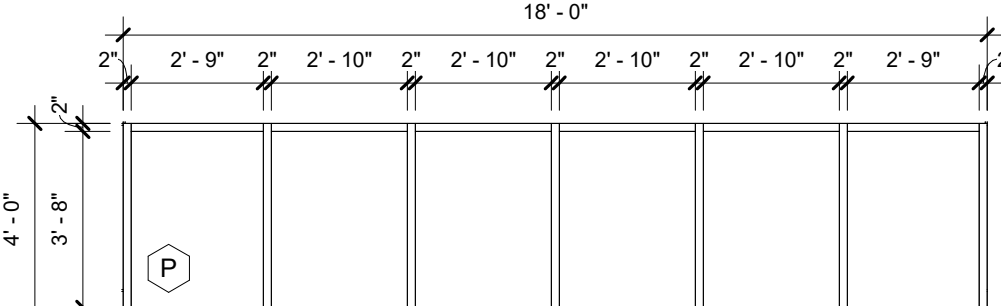
16 STOREFRONT ELEVATION P 1/4" = 1'-0"
