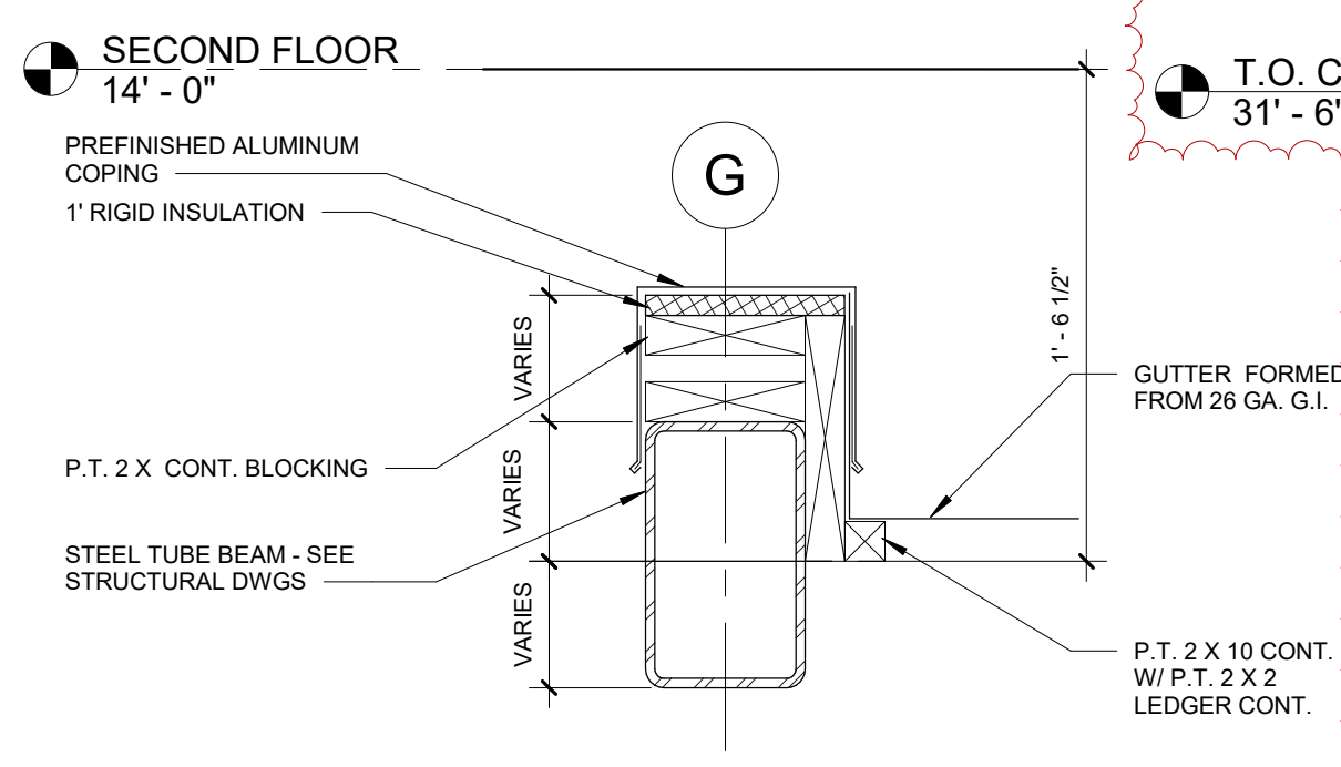
2 CHILDREN'S ENTRANCE FRAMING DTL. 1 1/2" = 1'-0"
