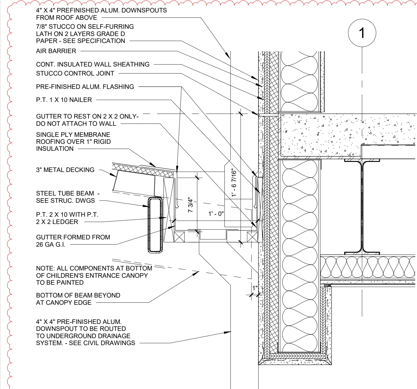
1 SECTION THROUGH CANOPY GUTTER @ STUCCO WALL 1 1/2" = 1'-0"
