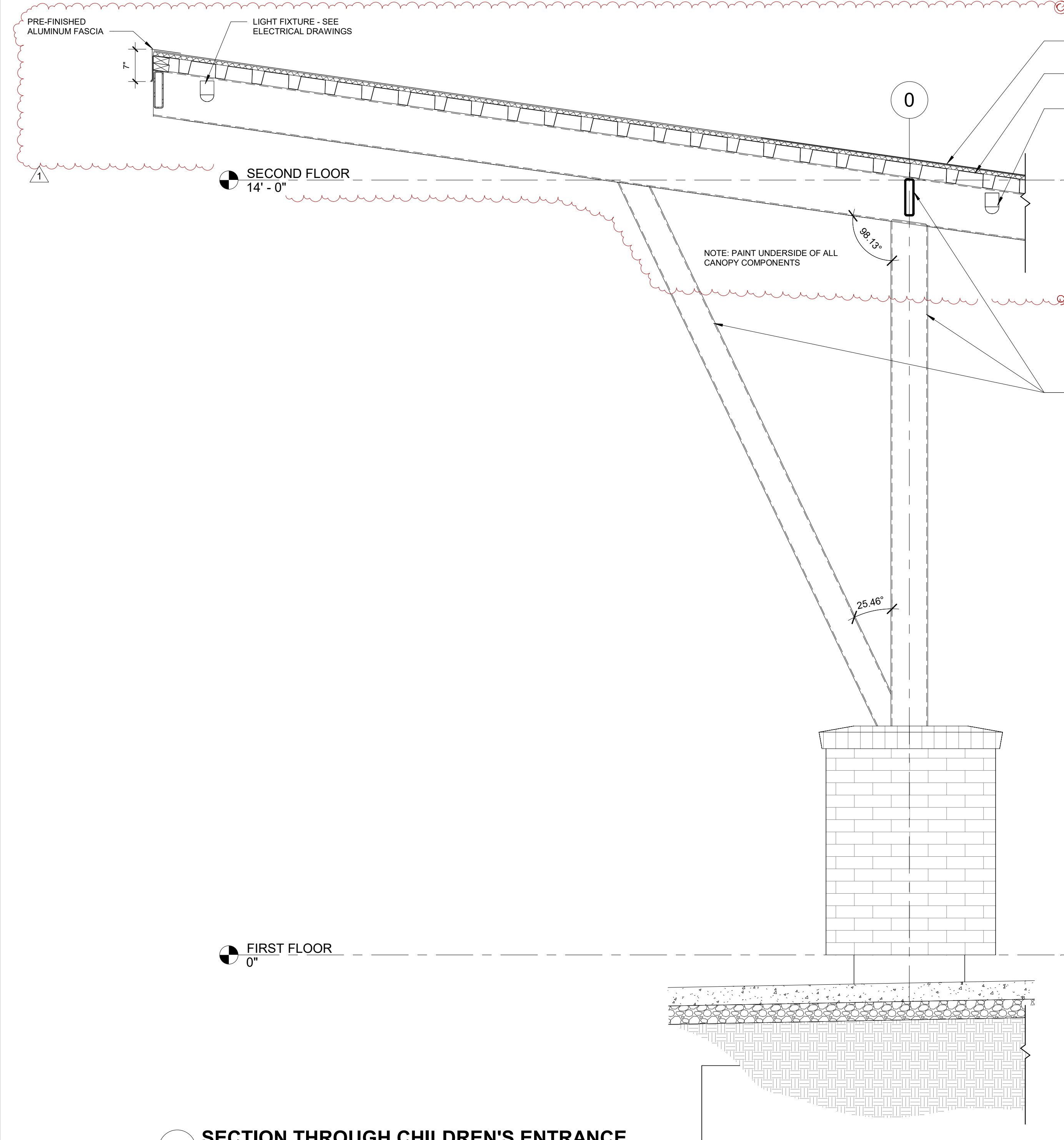
3 SECTION THROUGH CHILDREN'S ENTRANCE 3/4" = 1'-0"
