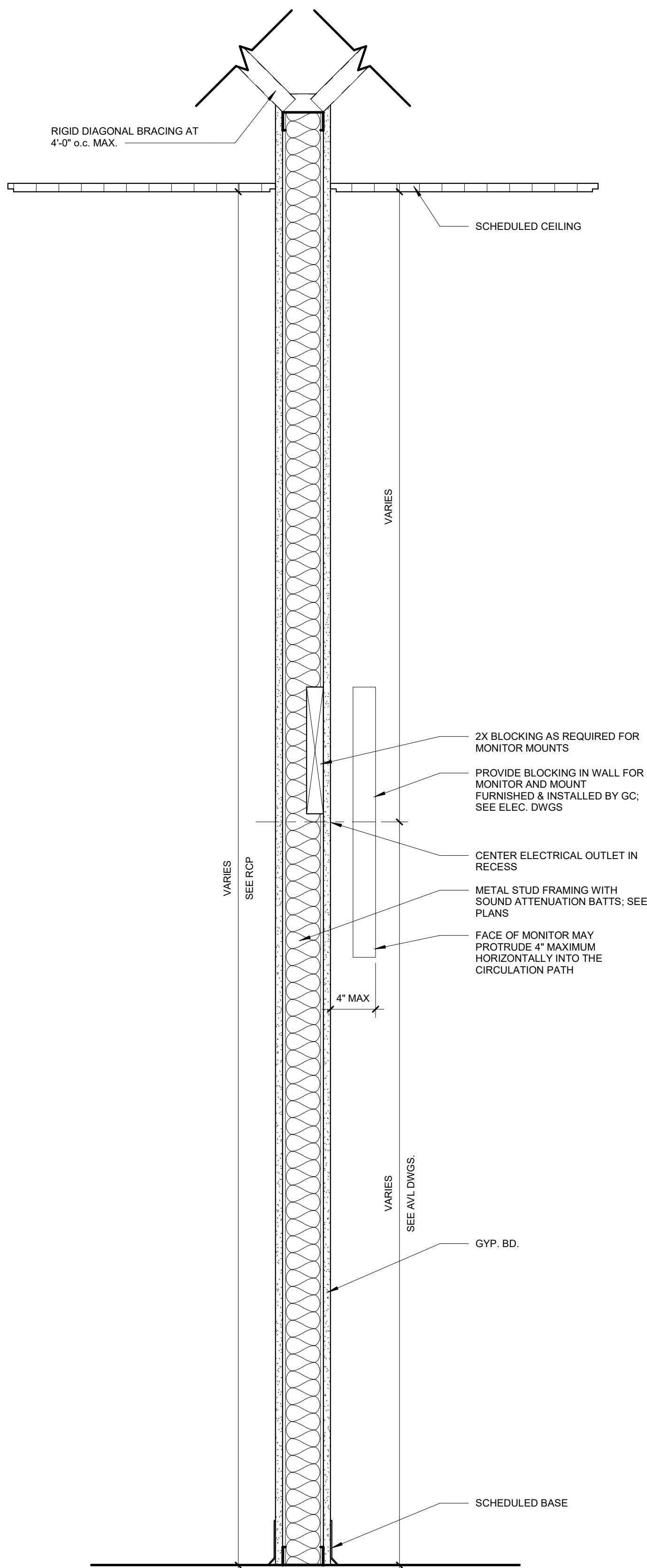
1 WALL SECTION - SURFACE MOUNTED TV 1 1/2" = 1'-0"
