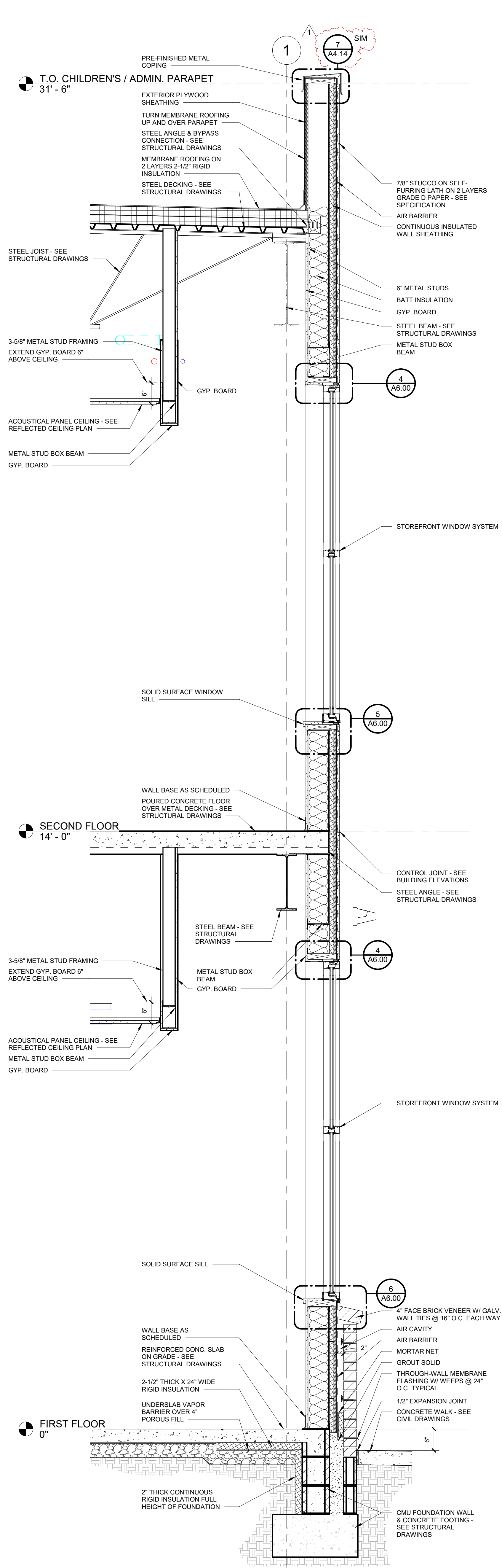
3 WALL SECTION @ EAST ELEVATION 3/4" = 1'-0"
