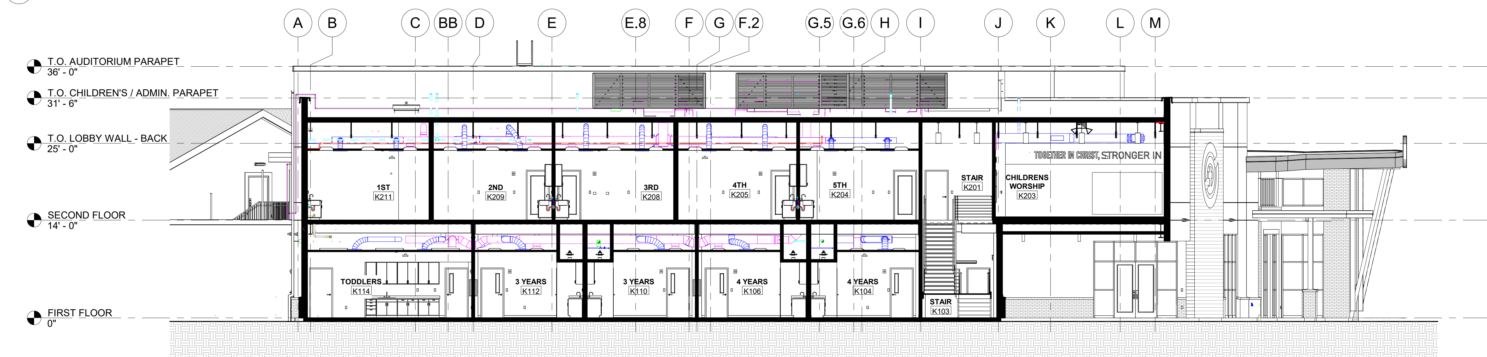
4 BUILDING SECTION FACING WEST 01 1/8" = 1'-0"
