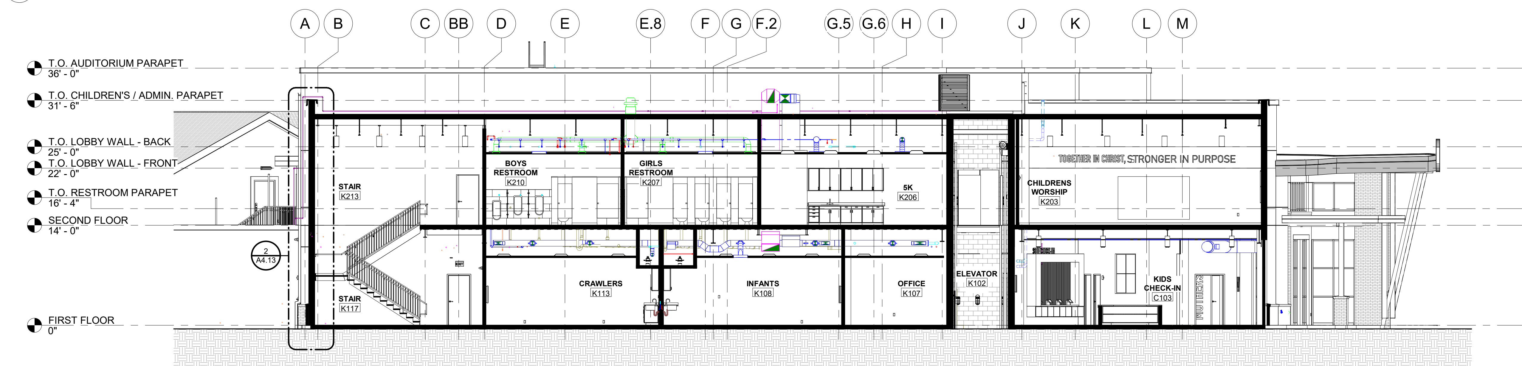
3 BUILDING SECTION FACING WEST 02 1/8" = 1'-0"
