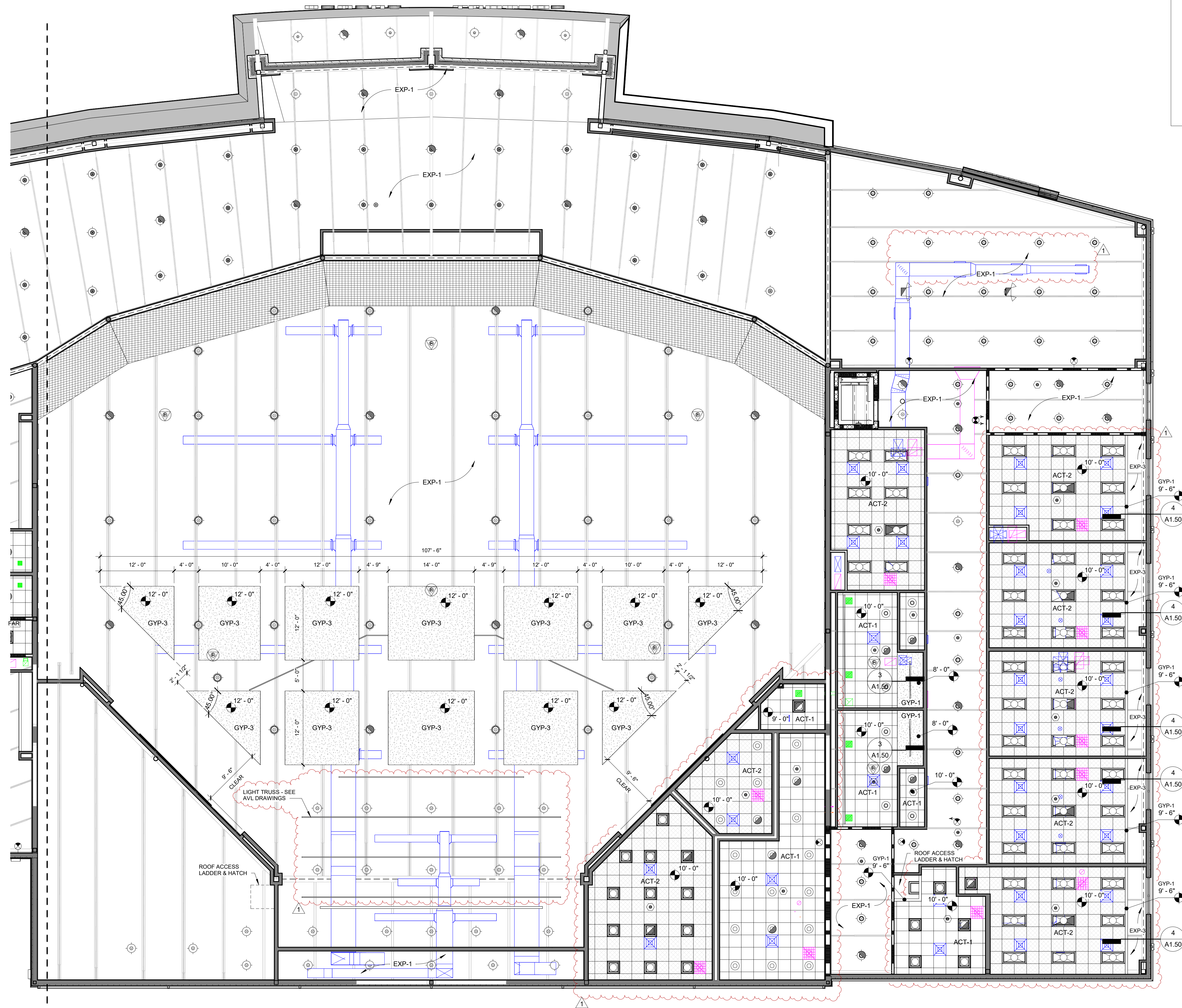
1 SECOND FLOOR REFLECTED CEILING PLAN - EAST 1/8" = 1'-0"
