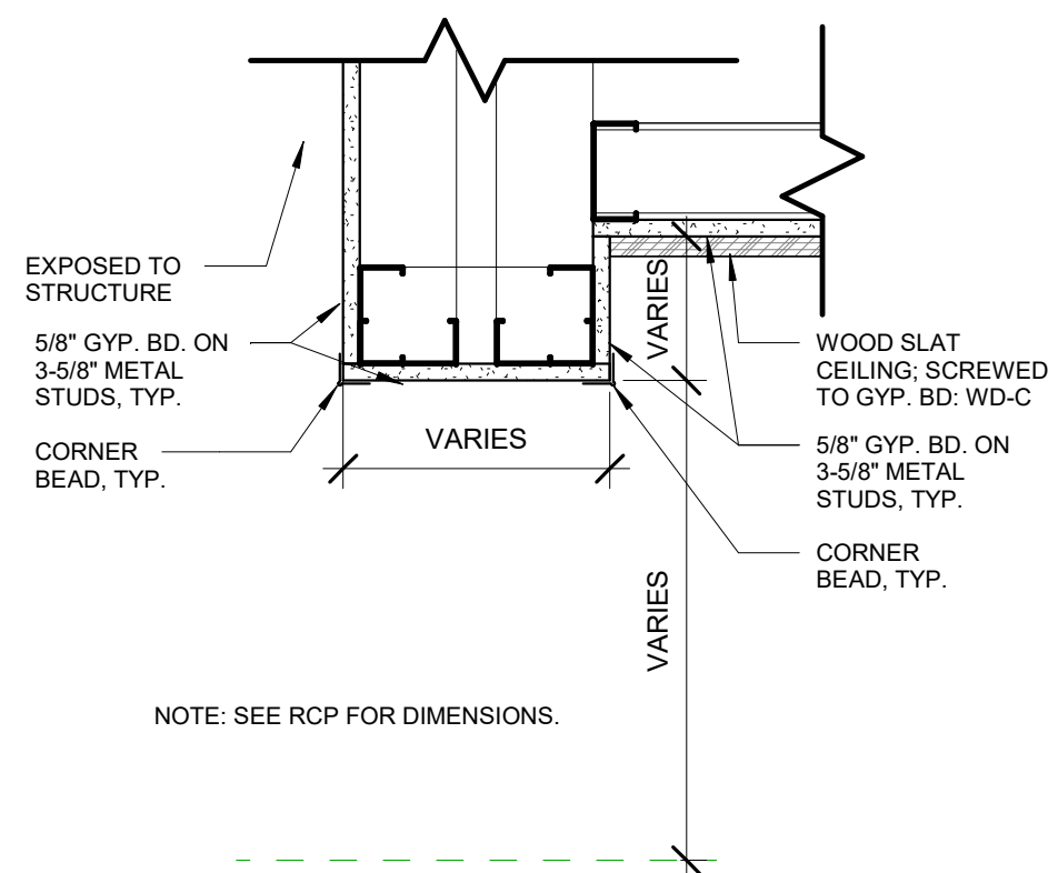
6 CEILING DETAIL - EXPOSED TO WD-C 1 1/2" = 1'-0"
