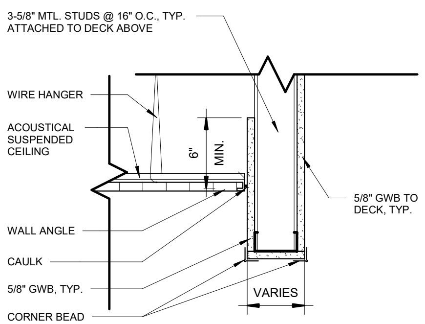
4 CEILING DETAIL - ACT TO EXPOSED 1 1/2" = 1'-0"
