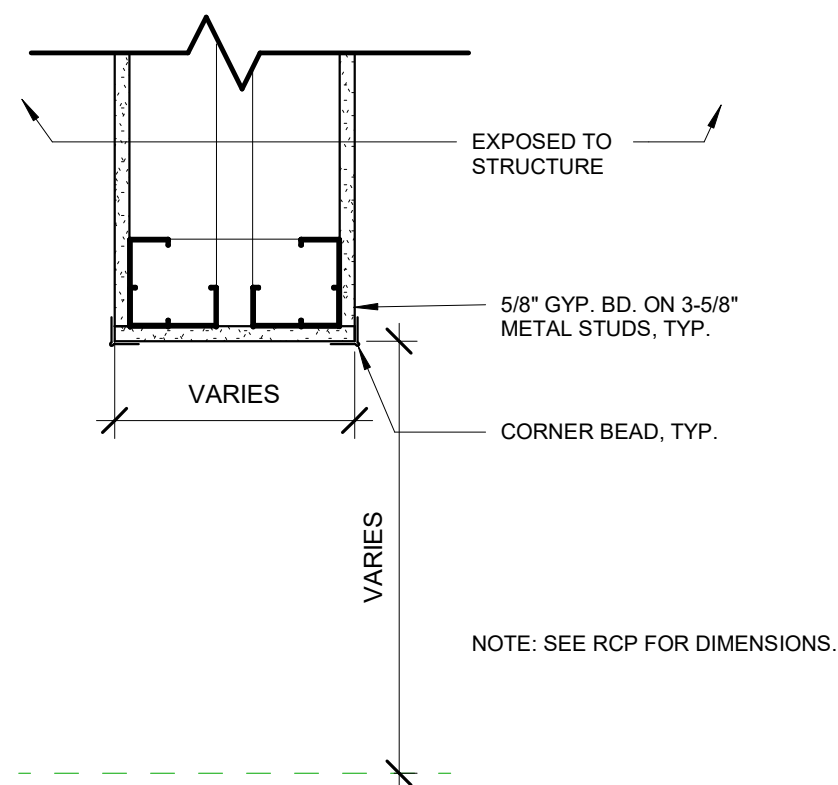
5 CEILING DETAIL - EXPOSED TO EXPOSED 1 1/2" = 1'-0"
