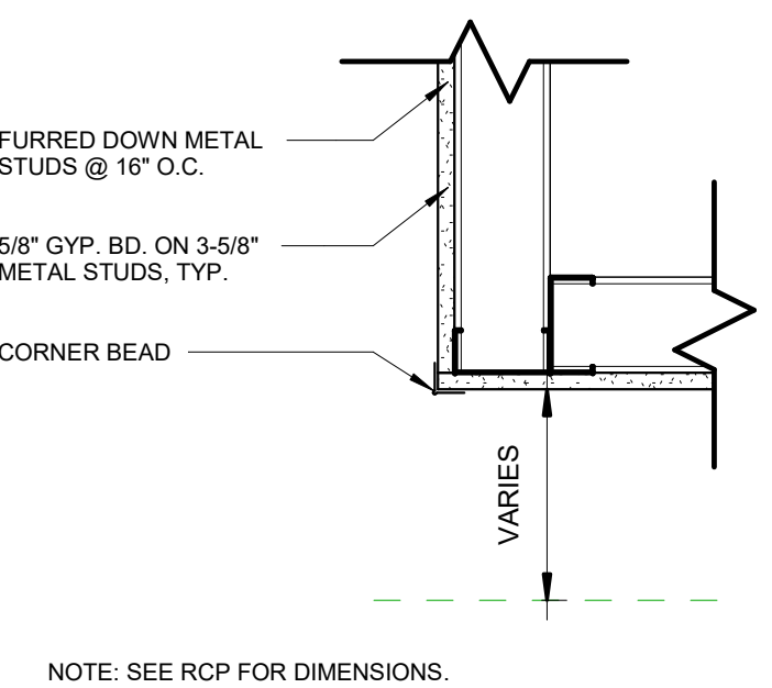
2 CEILING DETAIL - EXPOSED TO GYP 1 1/2" = 1'-0"
