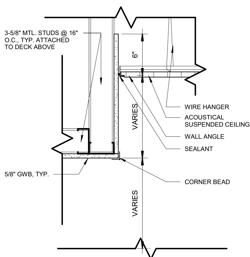
3 CEILING DETAIL - ACT TO GYP 1 1/2" = 1'-0"
