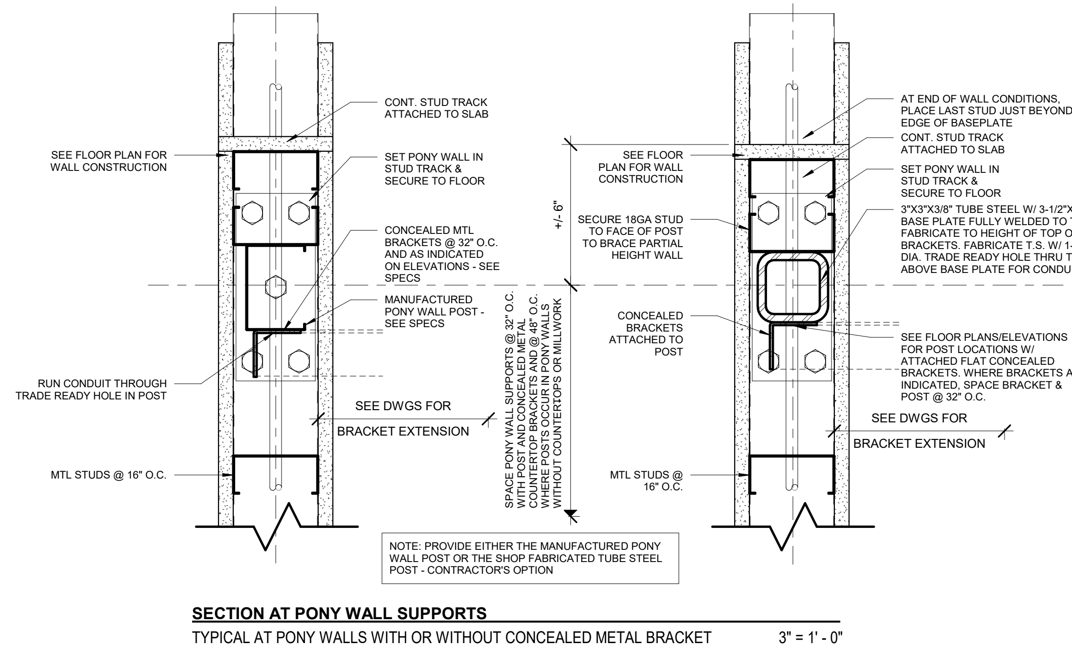
1 PONY WALL SUPPORT DETAIL
