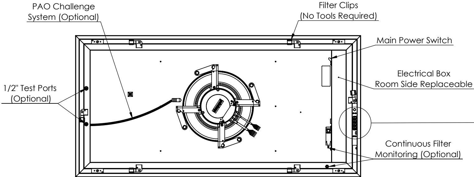
FACE FRAME AND HEPA FILTER REMOVED FOR CLARITY
