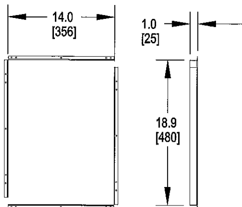
SUPPLY AIR DUCT FLANGES INSTALLED DIMENSIONS
