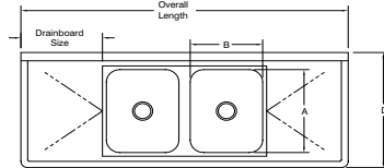
2 Compartment With 2 Drainboards Shown
