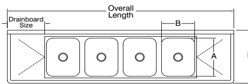
4 Compartment With 2 Drainboards Shown
