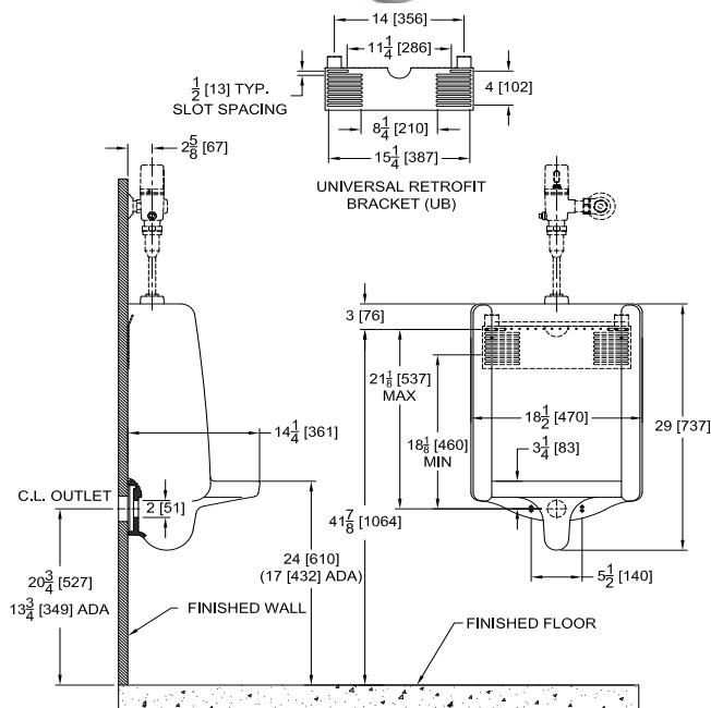
Rough-in/Overview dimensions for Z5758 Series
