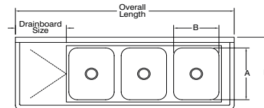
3 Compartment With 1 Left Drainboard Shown
