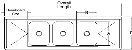
3 Compartment With 2 Drainboards Shown
