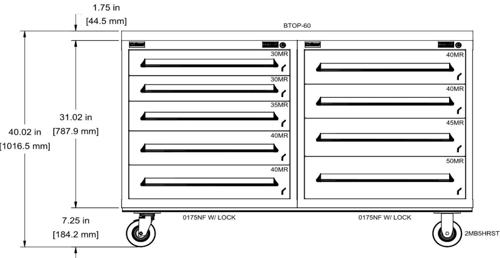
FRONT ELEVATION LAYOUT
