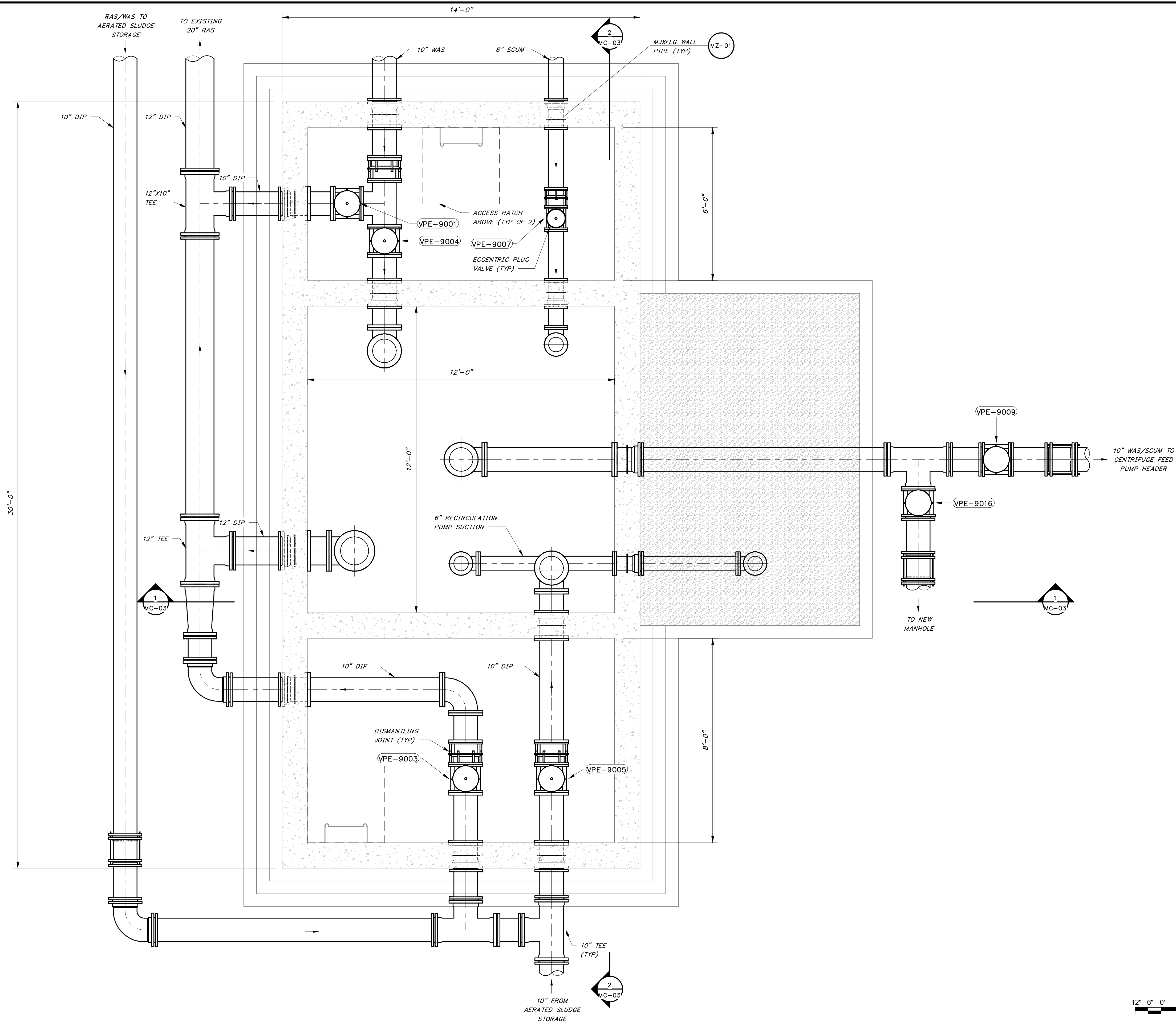
DETAIL 1 1/2" = 1'-0"
