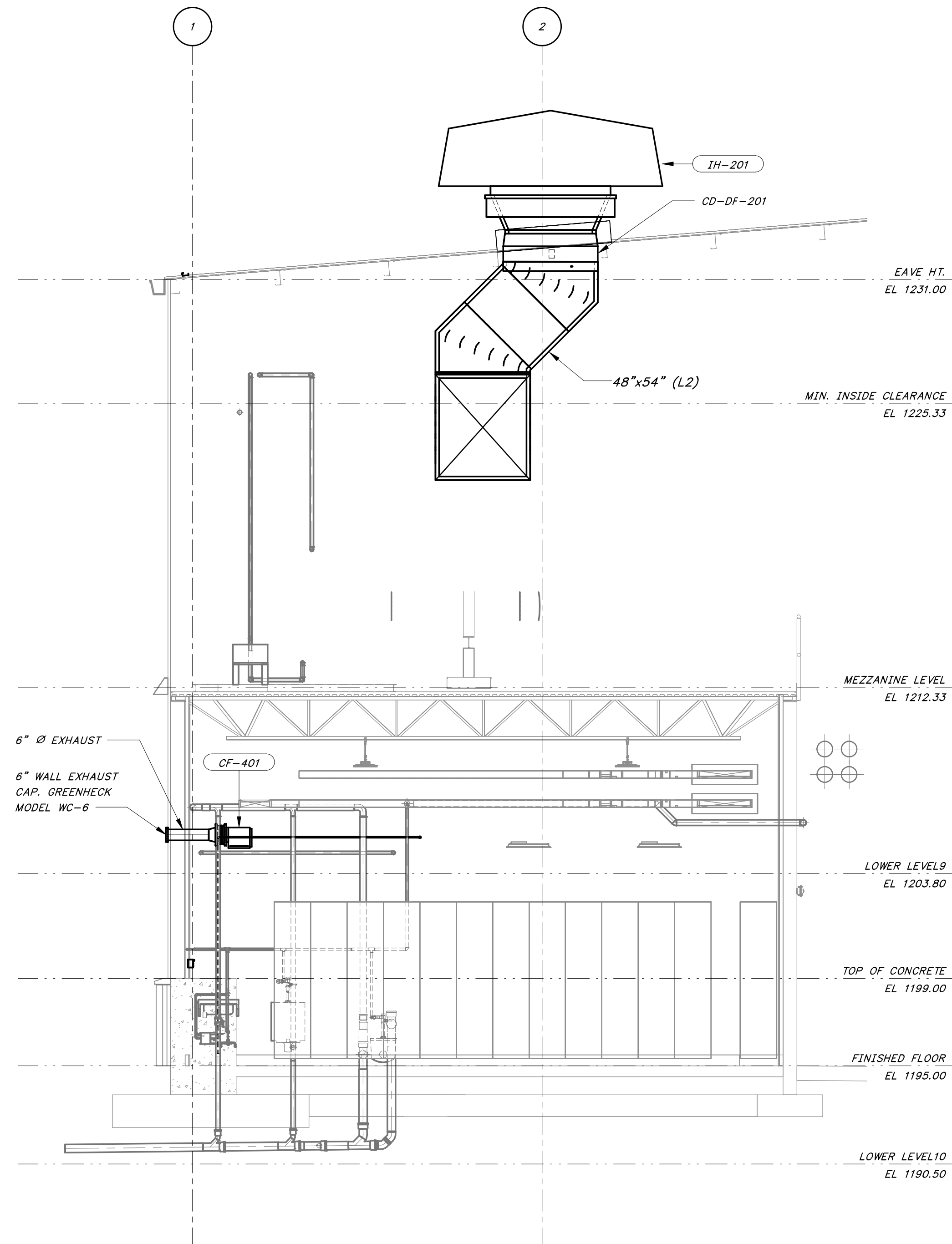
1 DRYER ROOM & BOILER ROOM SECTION - SOUTH HA-02 1/4" = 1'-0"
