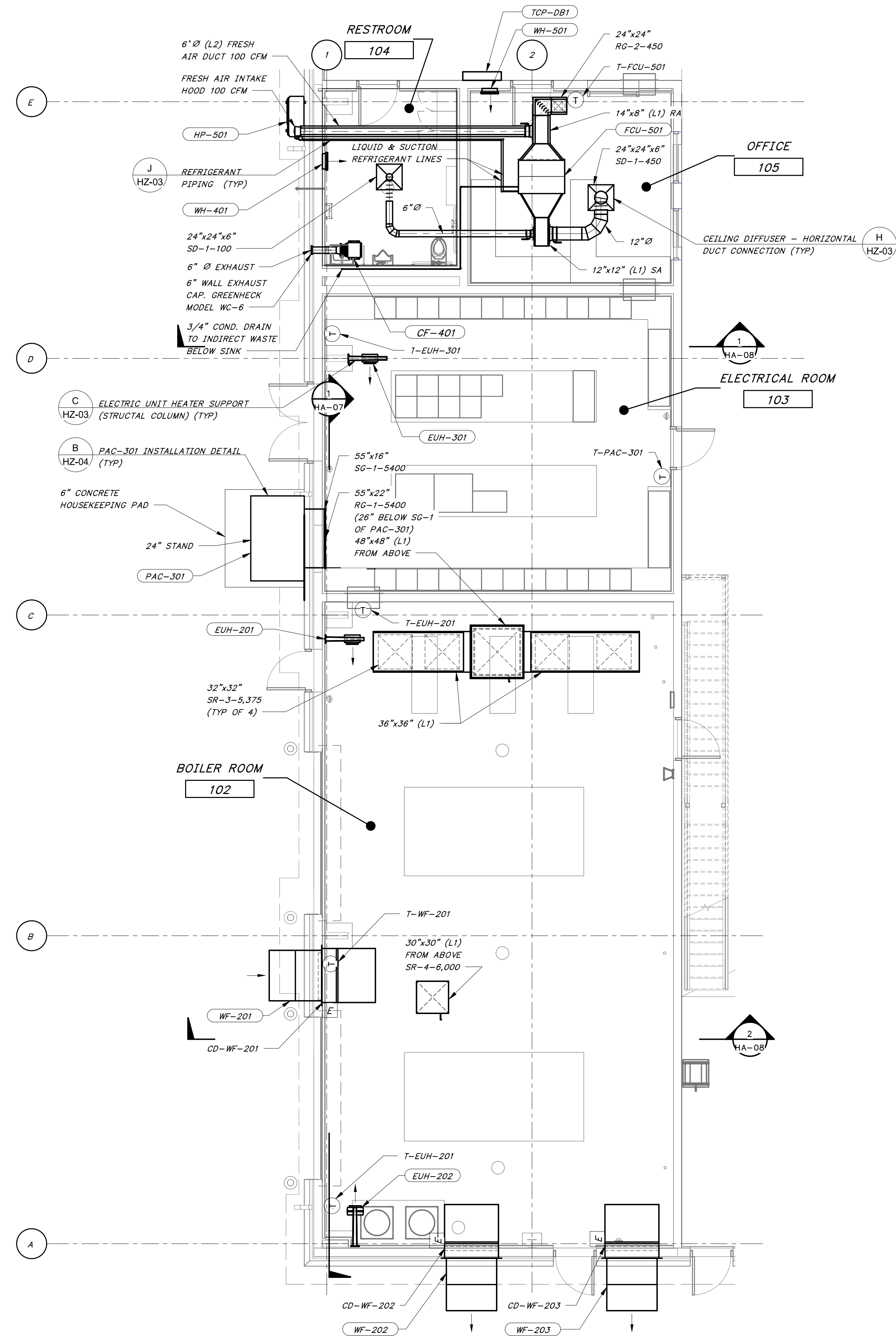
LOWER LEVEL- ENLARGED PLAN 3/16" = 1'-0"
