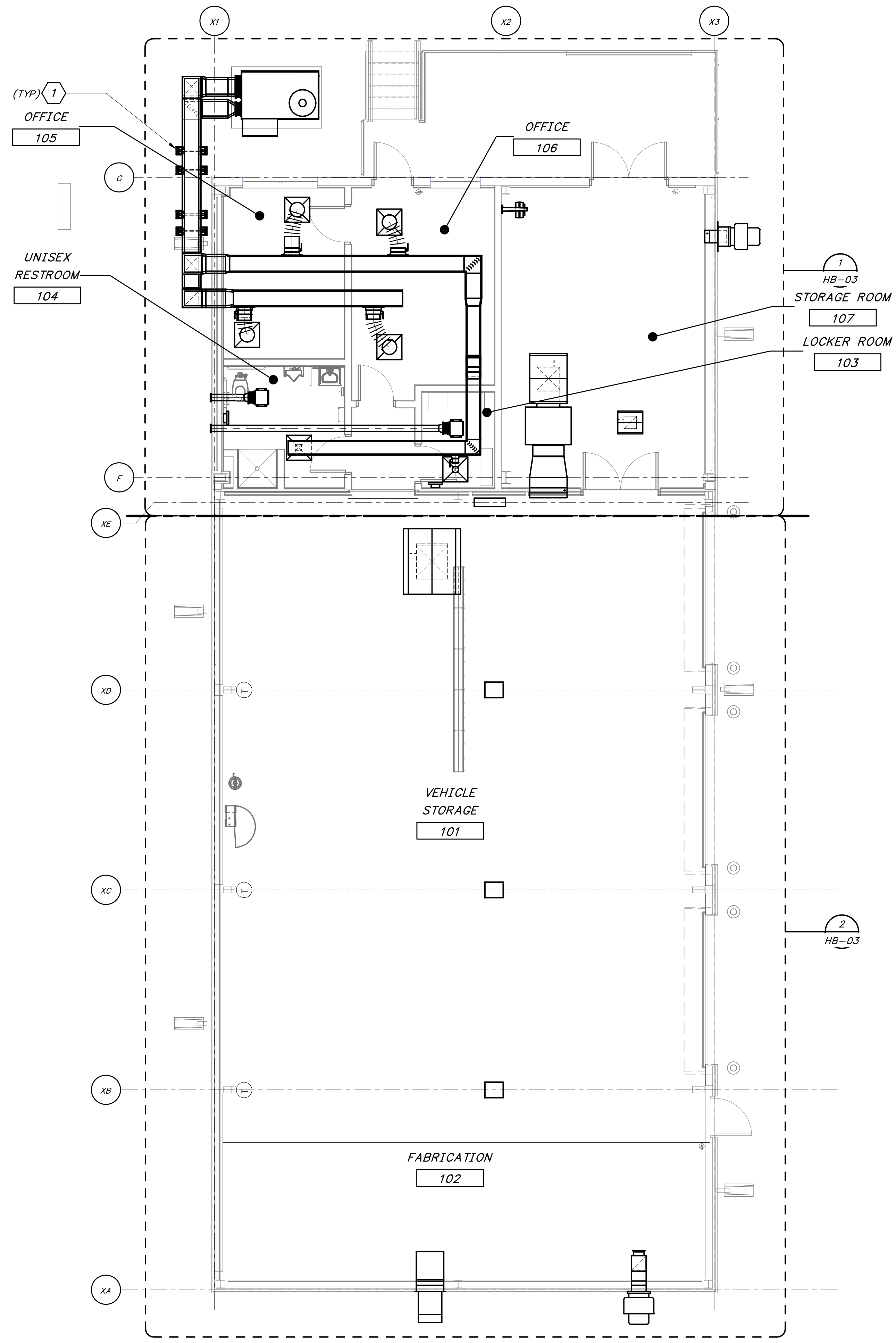
OVERALL - HVAC PLAN 3/16" = 1'-0"
