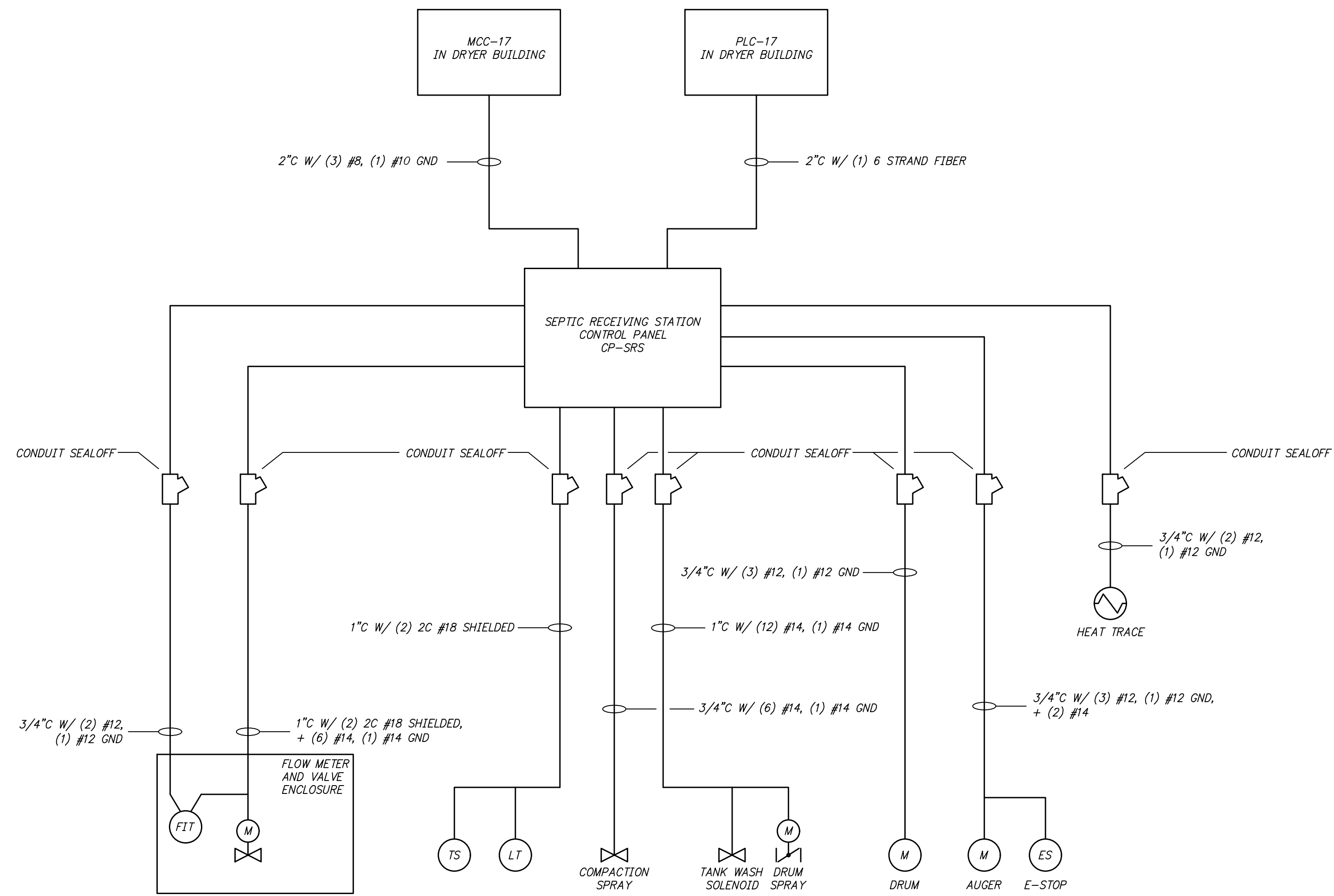
SEPTIC RECEIVING STATION POWER AND CONTROLS RISER DIAGRAM DETAIL B N.T.S. ED-1
