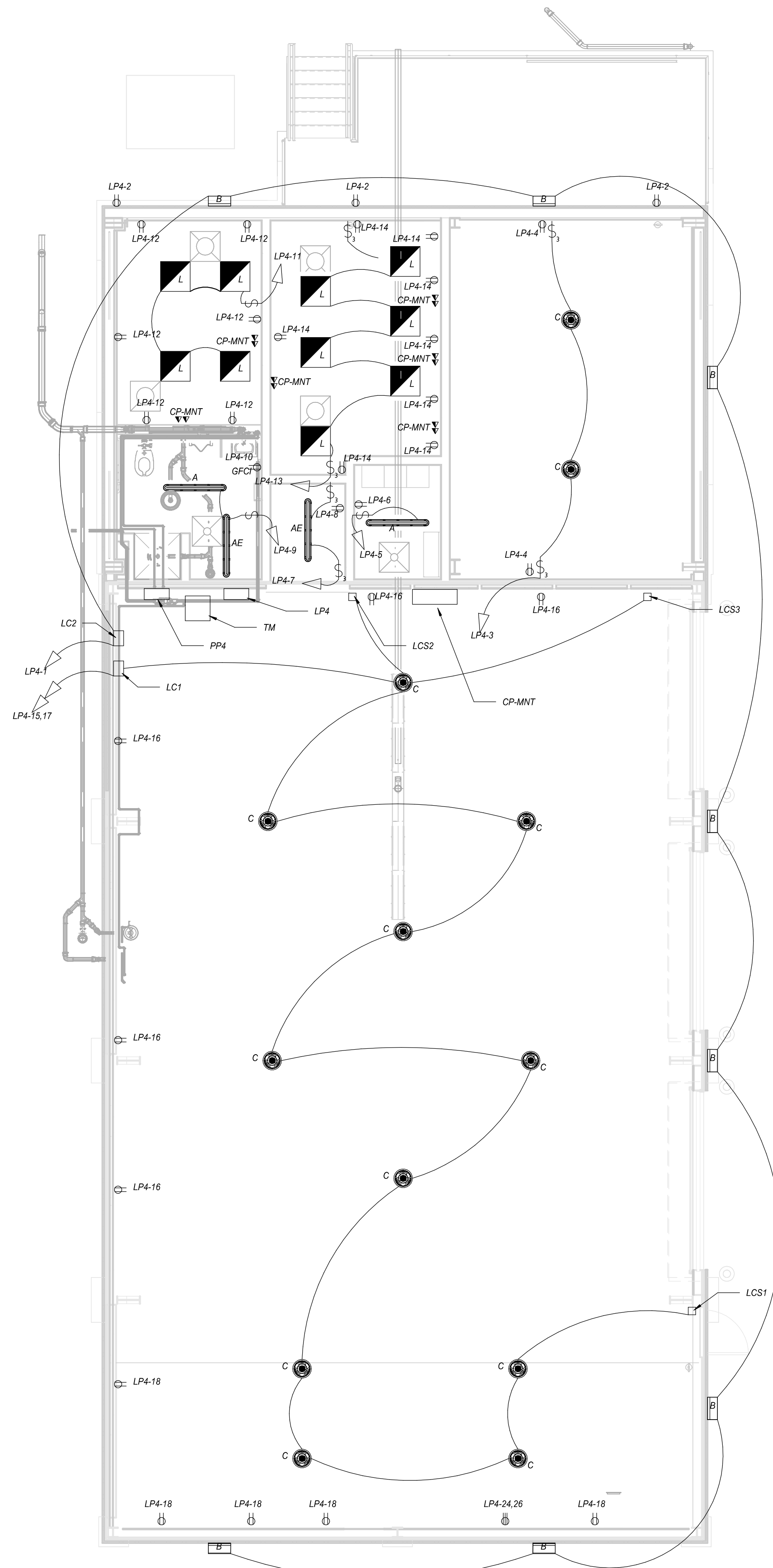
DETAIL 3/16" = 1'-0" 1
