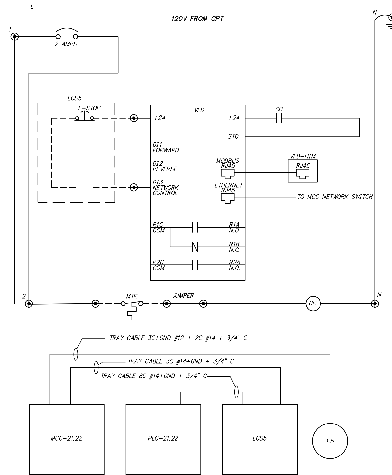
EXTRUDER TRACTION DRIVE CONTROL AND RISER DIAGRAM (TYP OF 2)
