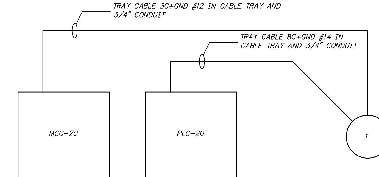
SCREW CONVEYOR GATE ACTUATORS CONTROL AND RISER DIAGRAM (TYP OF 2)
