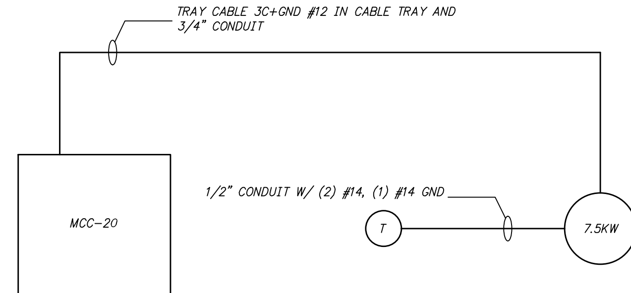
ELECTRIC UNIT HEATER CONTROL AND RISER DIAGRAM
