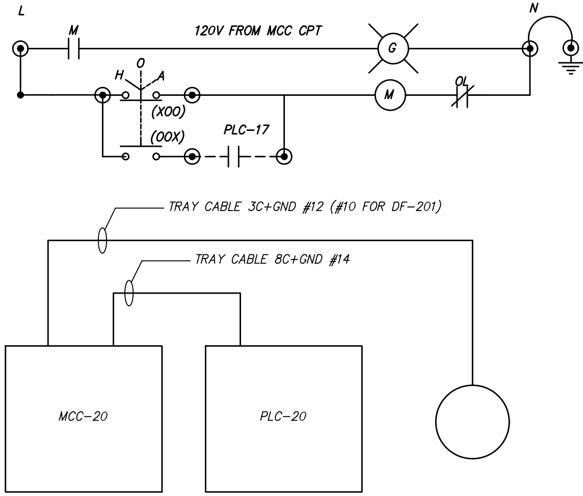
EXHAUST OR SUPPLY FAN CONTROL AND RISER DIAGRAM (TYP OF 8)
