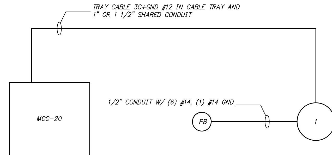
OVERHEAD COILING DOOR CONTROL AND RISER DIAGRAM
