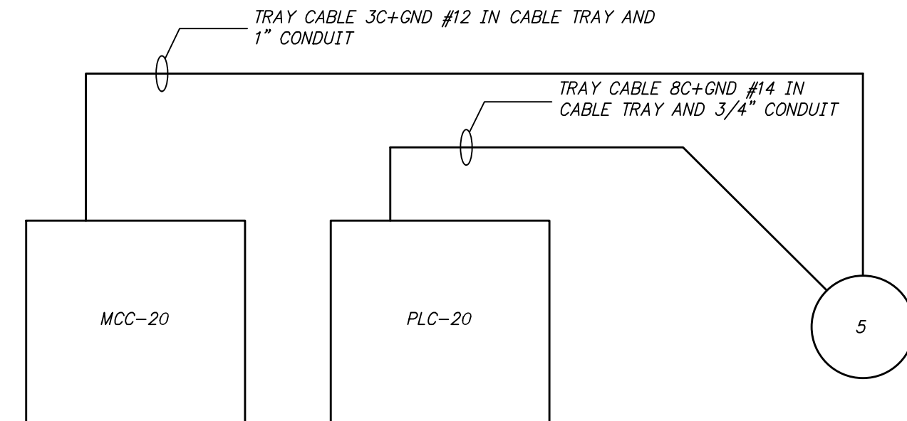
MAKEUP AIR UNIT MA-201 CONTROL AND RISER DIAGRAM
