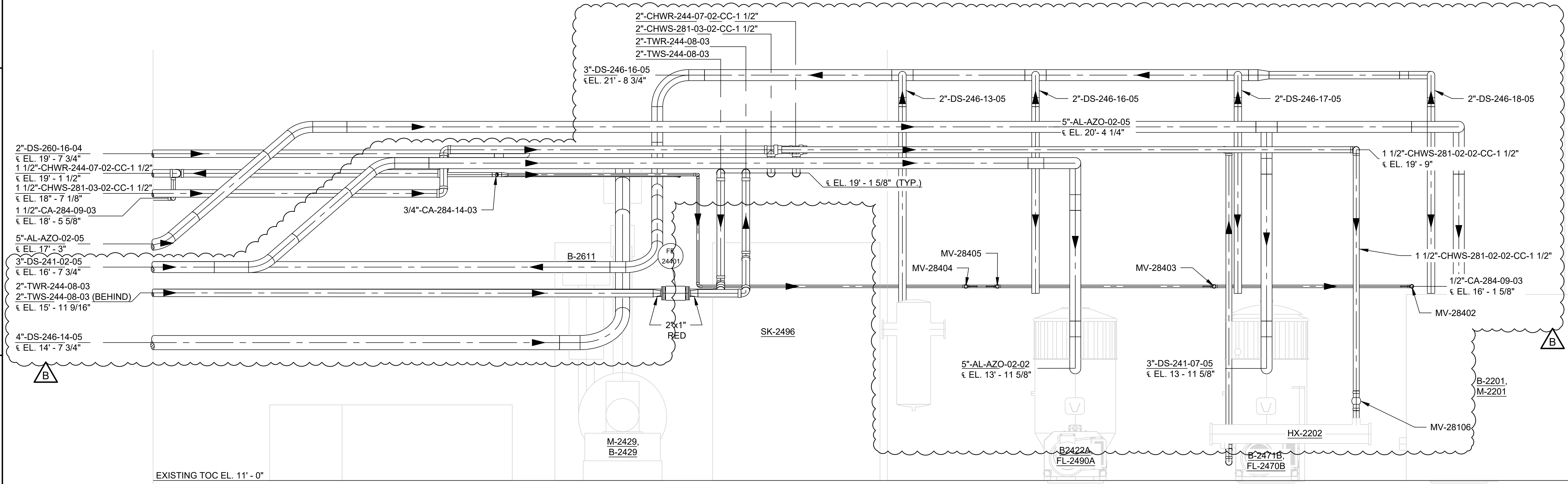
C1 PUMP ROOM ELEVATION VIEW 3/4" = 1'-0"
