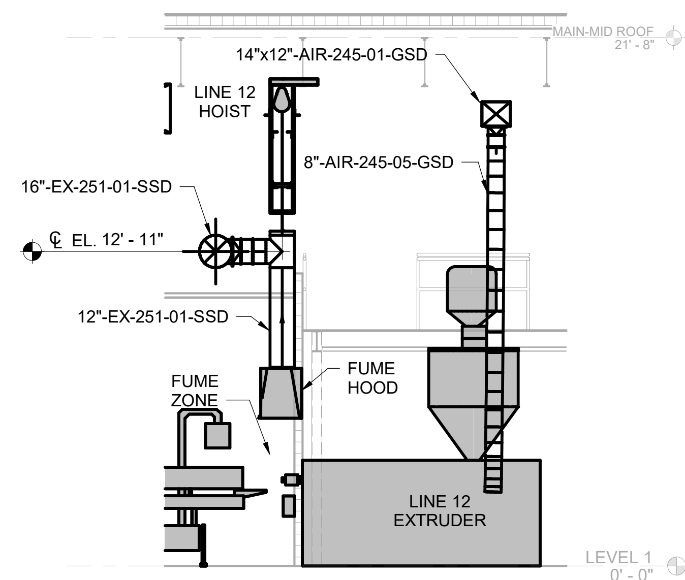
A1 EAST - 565 EXHAUST AIR AND EXTRUDER SUPPLY AIR
