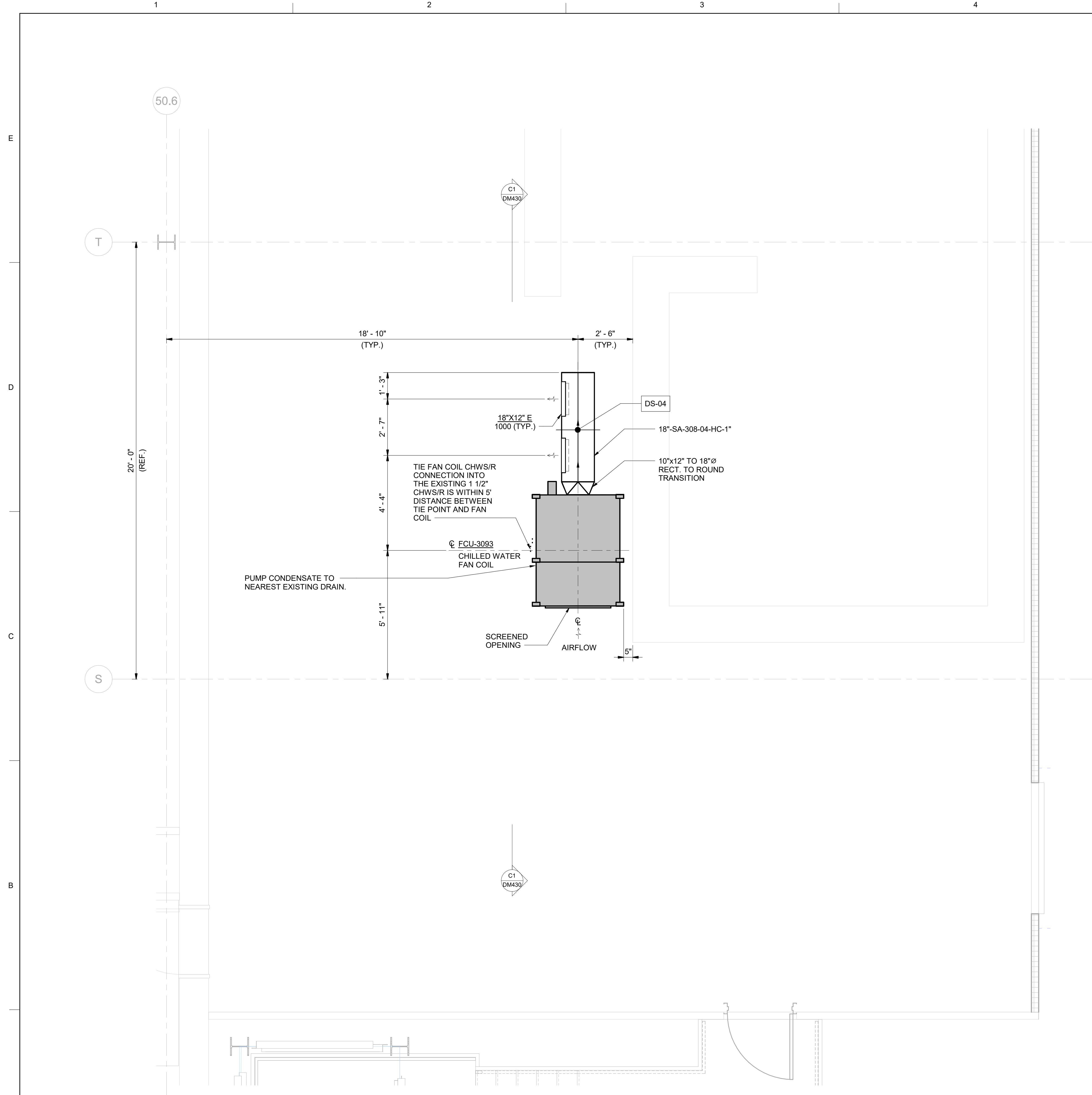
A1 DUCT - 565 PUMP ROOM ENLARGED SCALE: 1/2" = 1'-0"
