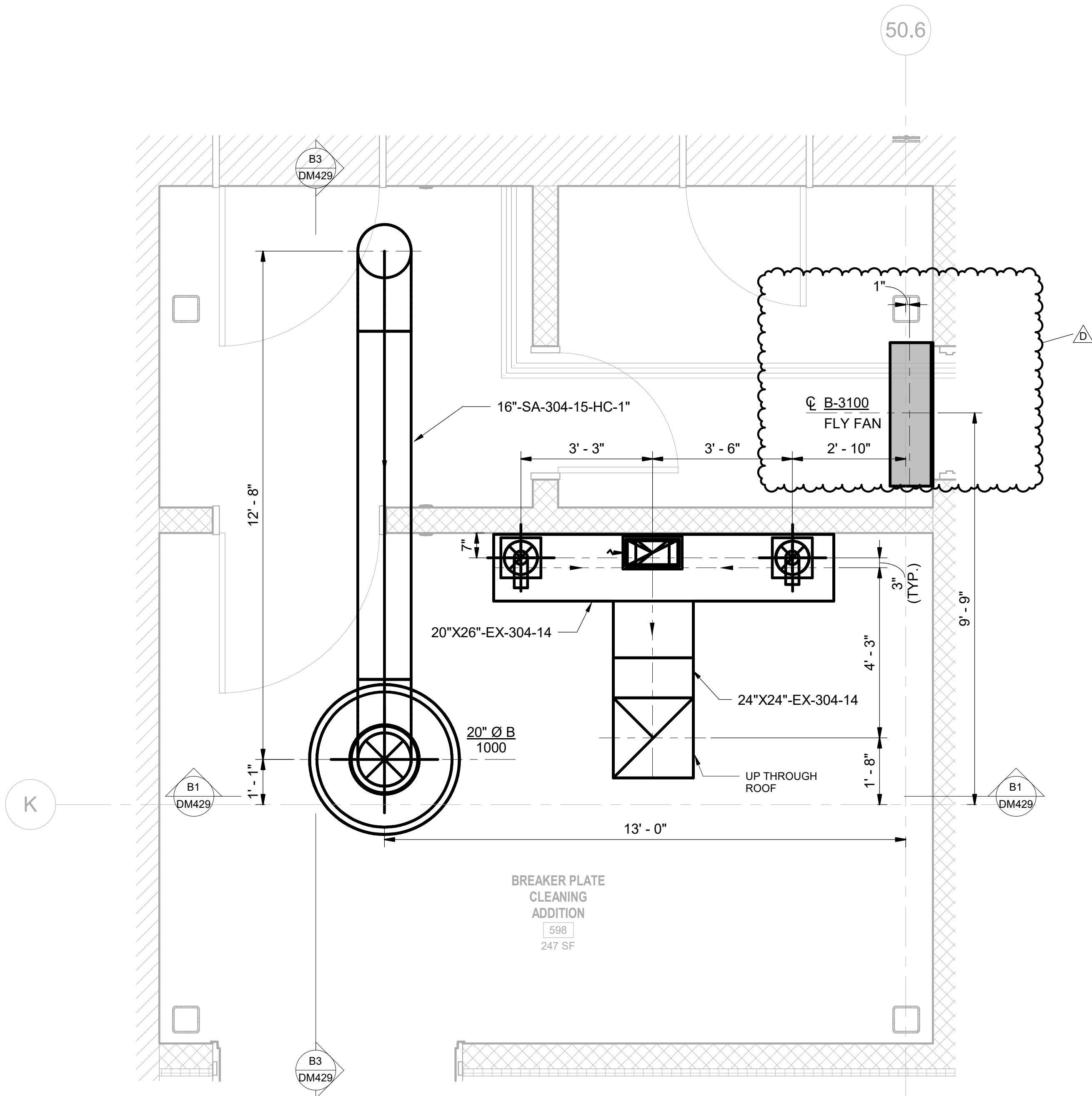
B1 DUCT - ENLARGED PLAN - 565 BREAKER PLATE SCALE: 1/2" = 1'-0"
