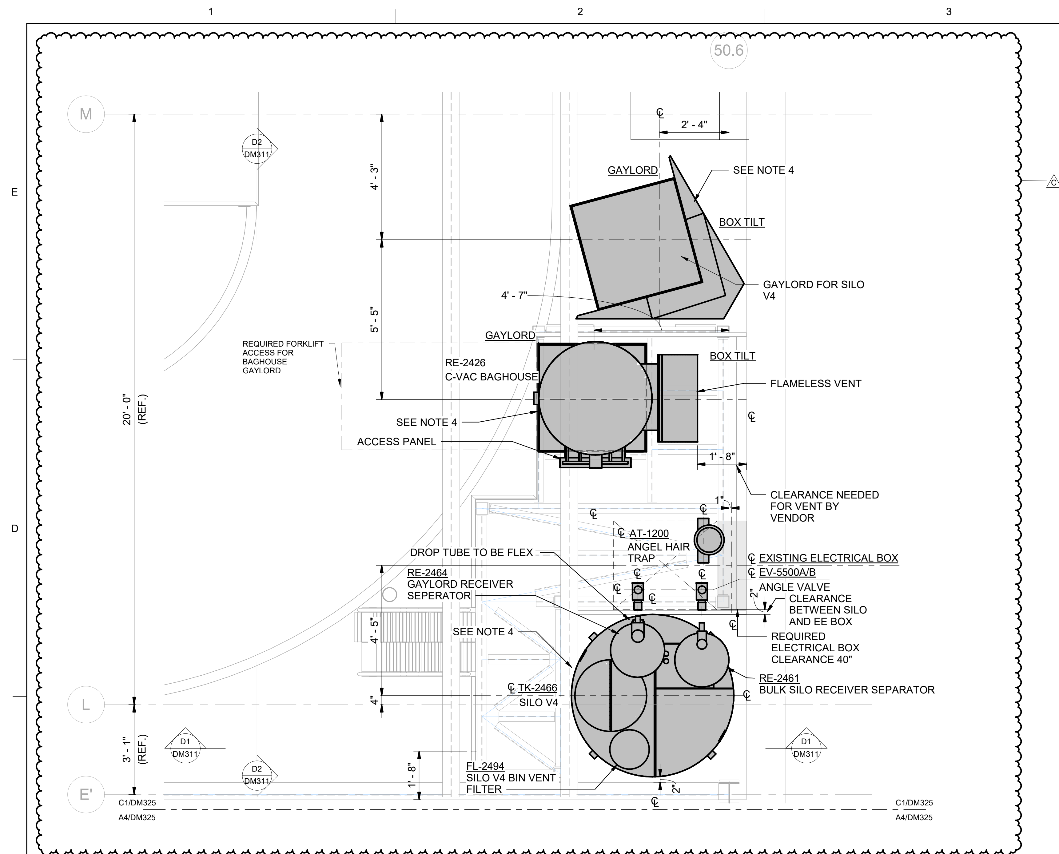
C1 ENLARGED PLAN - 565 CENTRALVAC BAG HOUSE & SILO V4 AREA SCALE: 1/2" = 1'-0"
