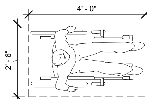
CLEAR FLOOR SPACE
