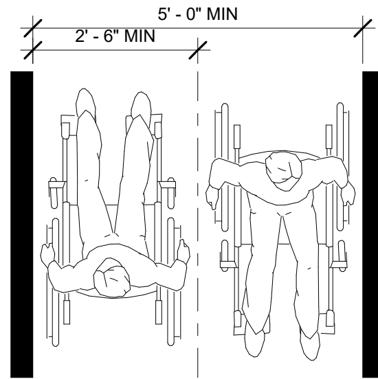
MINIMUM CLEAR WIDTH
