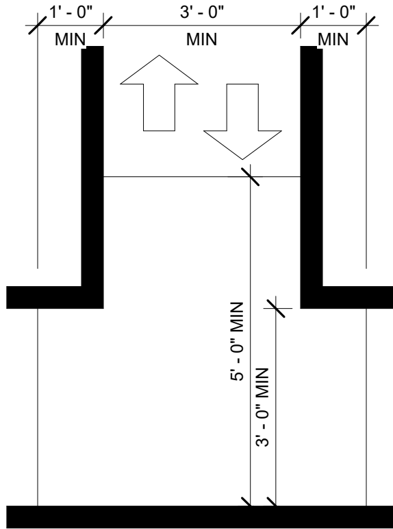
T-SHAPED TURNING SPACE
