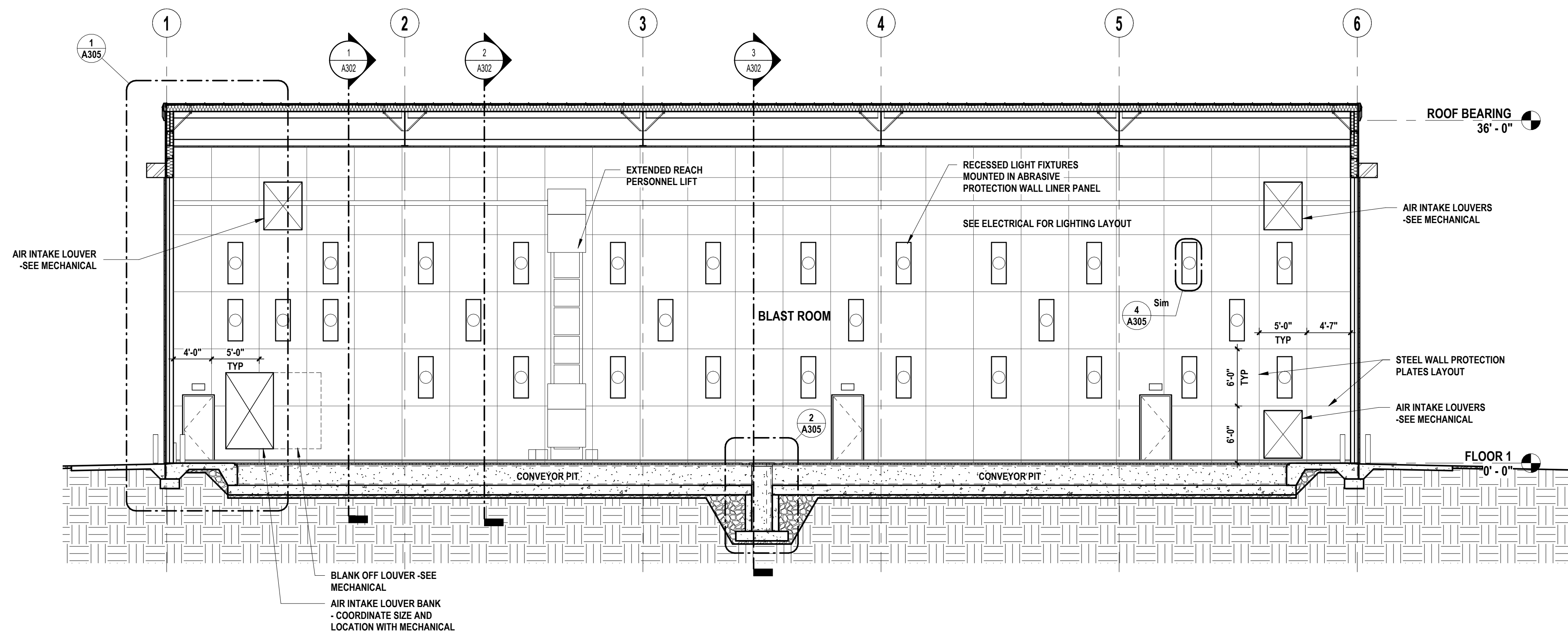
1 BUILDING SECTION - LONGITUDINAL WEST WALL 1/8" = 1'-0"
