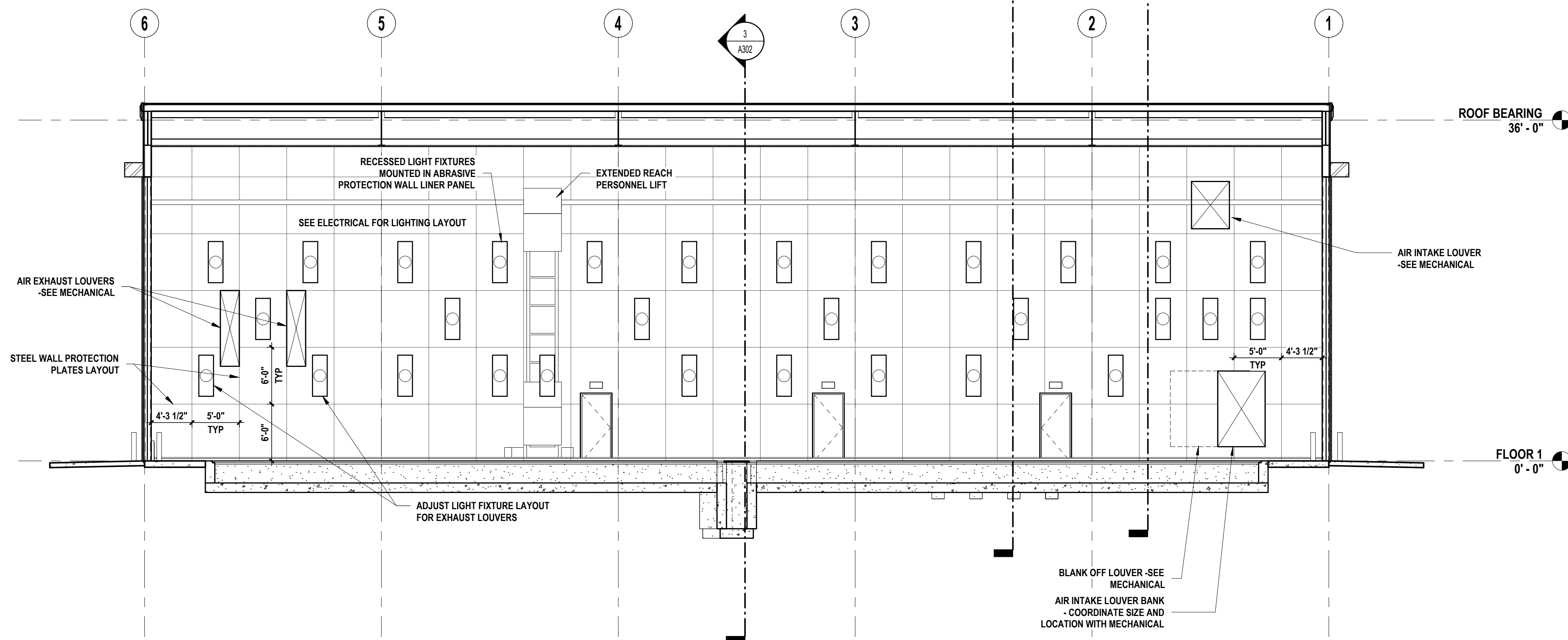
2 BUILDING SECTION - LONGITUDINAL EAST WALL 1/8" = 1'-0"
