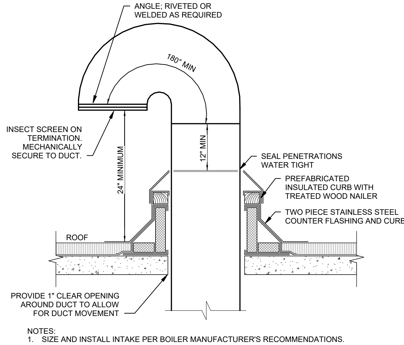
2 ROOF GOOSENECK DETAIL NTS
