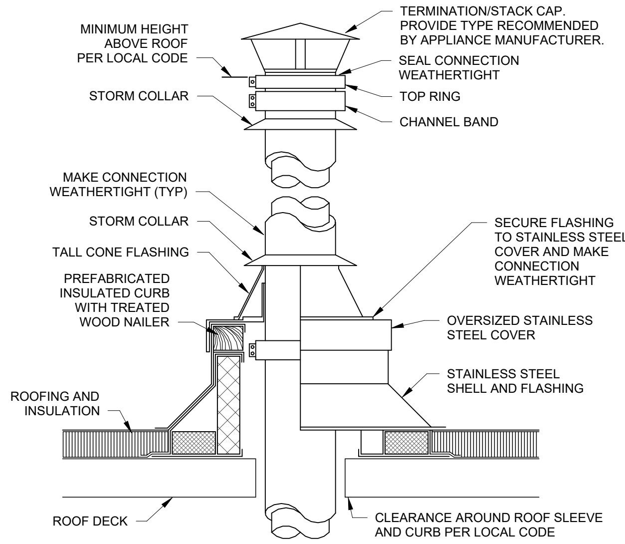
1 FLUE STACK DETAIL NTS
