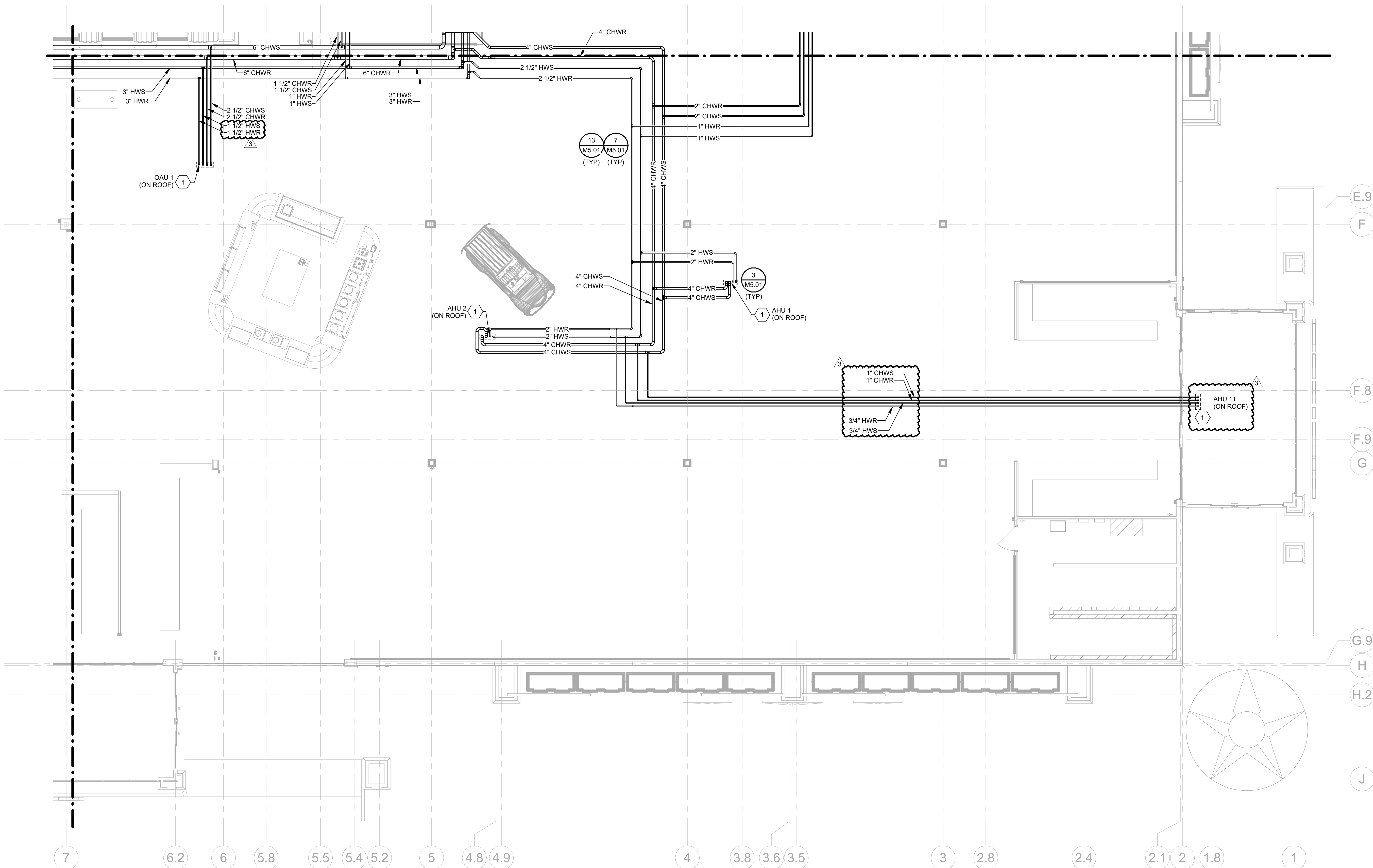
MECHANICAL PIPING FLOOR PLAN - AREA B 1/8" = 1'-0"
